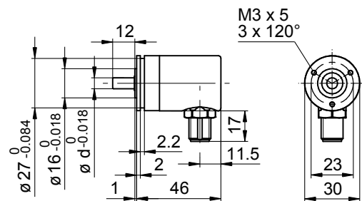
BMSV/BMMV 30R SSI, connector radial
