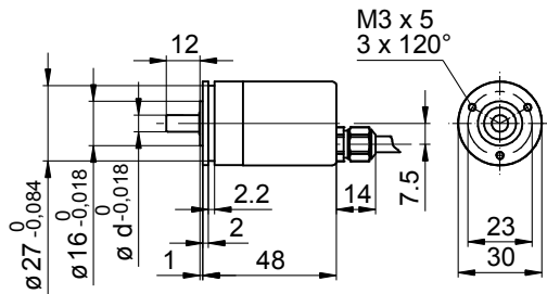
BMSV/BMMV 30R SSI, cable axial
