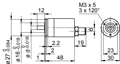
BMSV/BMMV 30R SSI, connector axial
