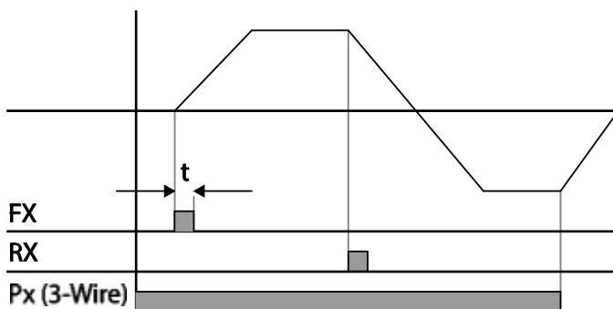
[Режим 3-wire]
