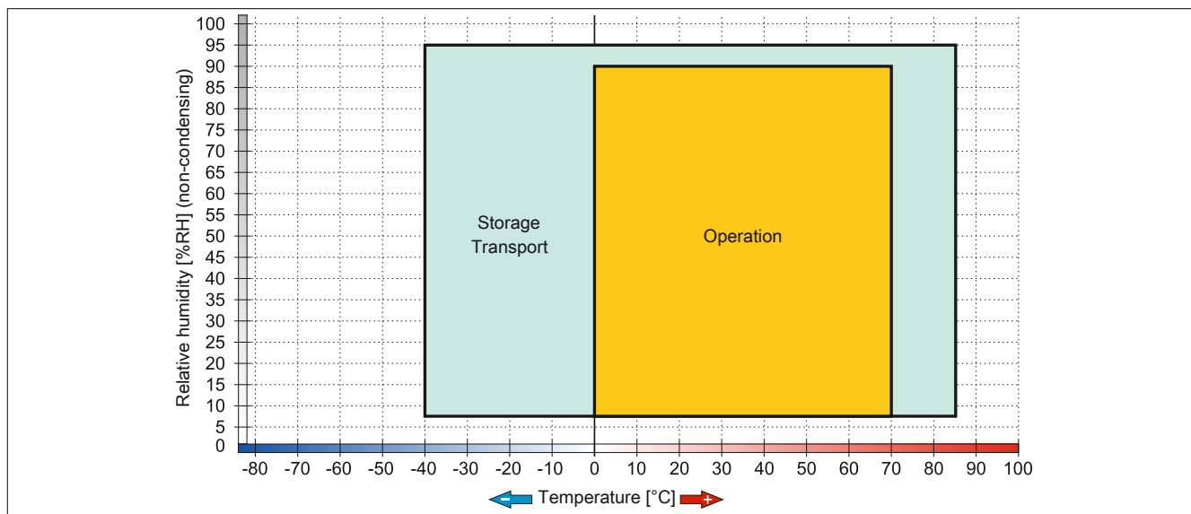
Figure 68: 5MMSSD.0128-01 ≤ Rev. C0 - Temperature/Humidity diagram
