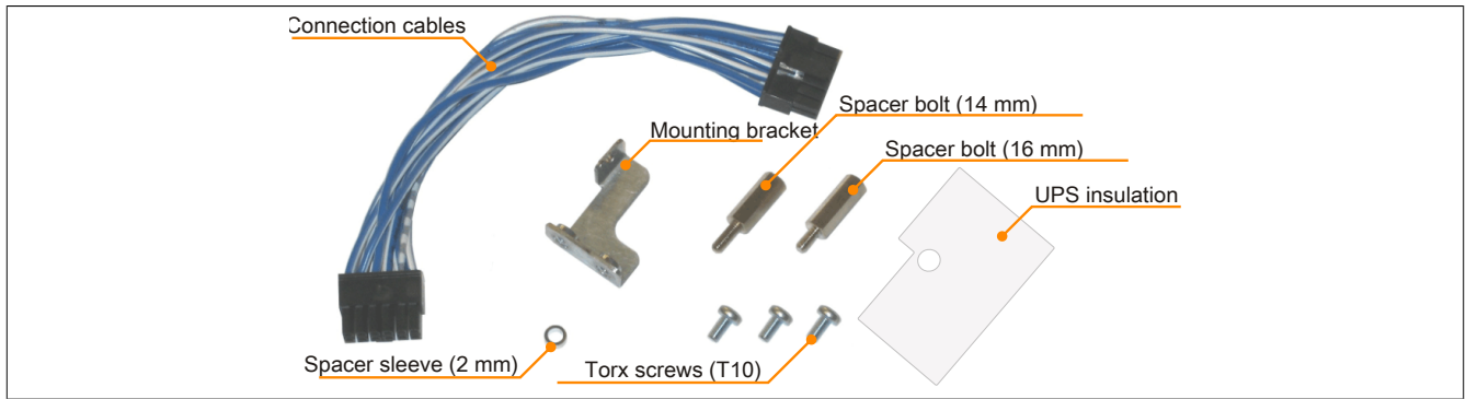
Figure 192: 5AC600. UPSI-00 Add-on UPS module - Installation materials
