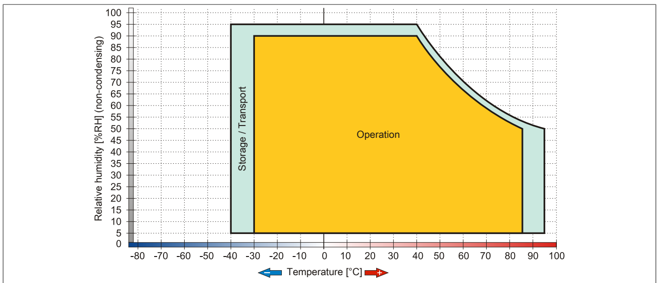
Figure 58: 5ACPCI.RAIC-04 - Temperature humidity diagram
