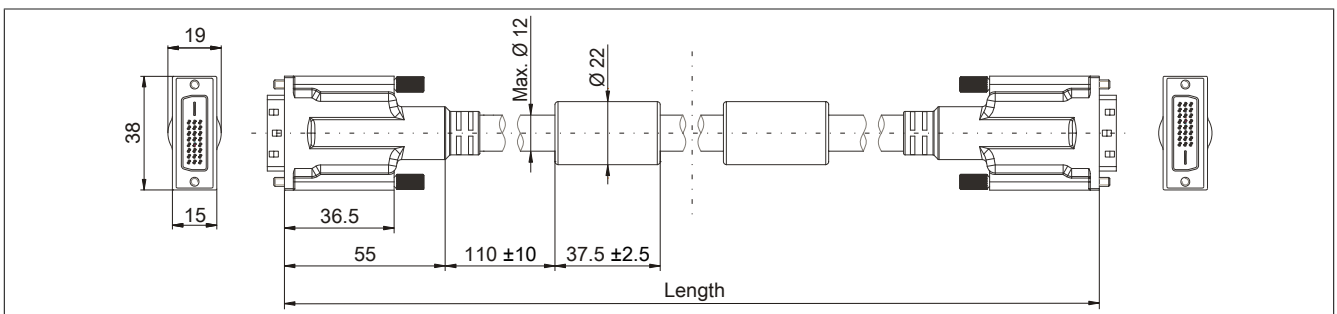
Figure 213: 5CASDL.0xxx-03 - Dimensions
