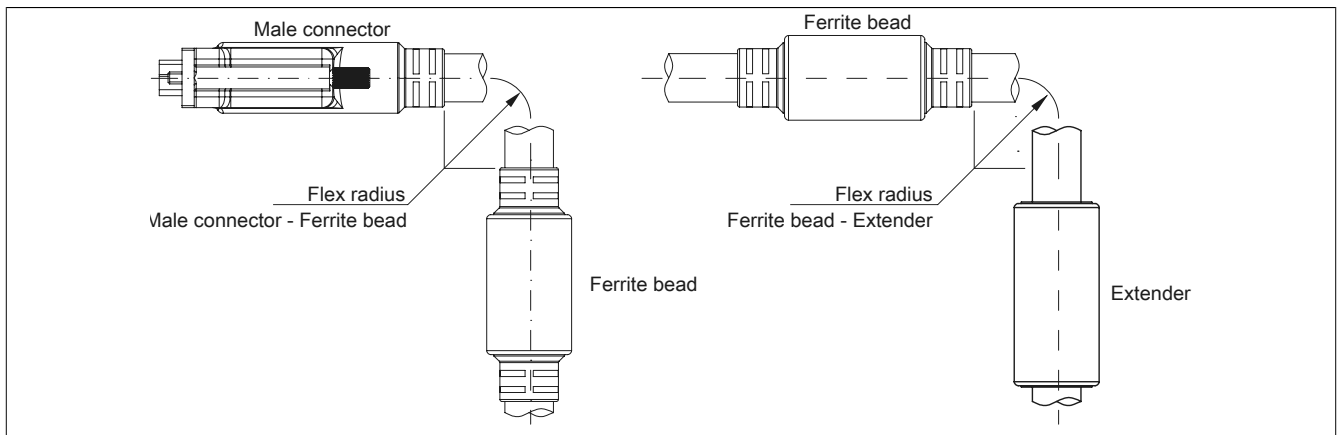
Figure 215: Flex radius specification with extender
