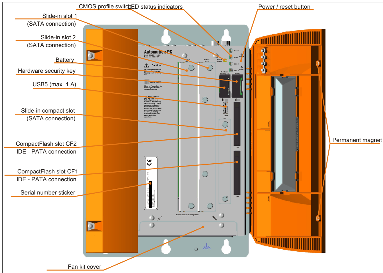
Figure 32: 5PC810.SX05-00 - Interfaces on front
