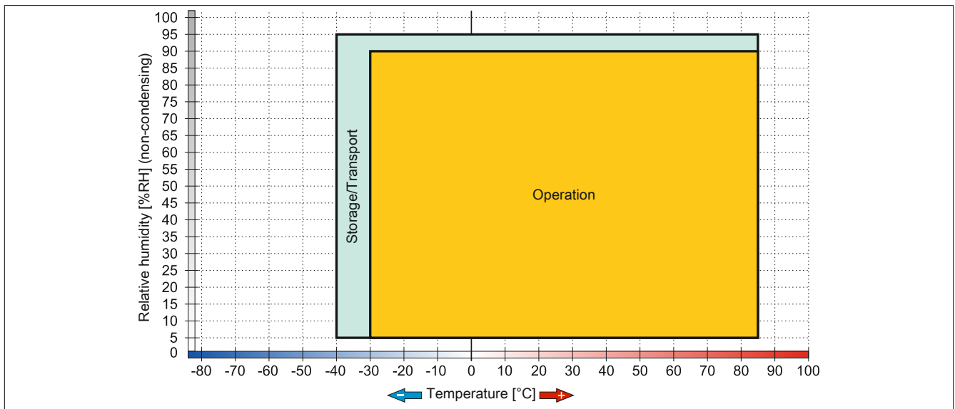
Figure 71: 5MMSSD.0256-00 - Temperature/Humidity diagram
