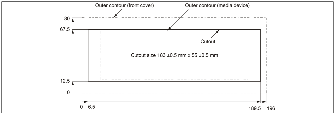
Figure 188: USB media drive with front cover - Installation cutout
