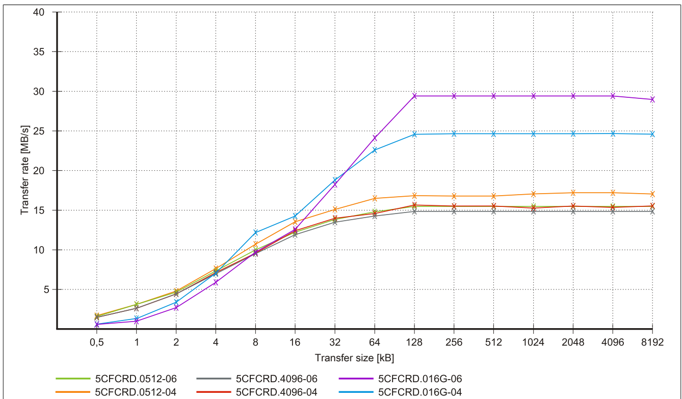
Figure 169: ATTO Disk Benchmark v2.34 write comparison - 5CFCRD.xxxx-04 and 5CFCRD.xxxx-06
