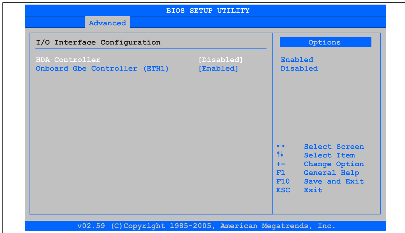
Figure 125: GM45 Advanced I/O Interface Configuration
