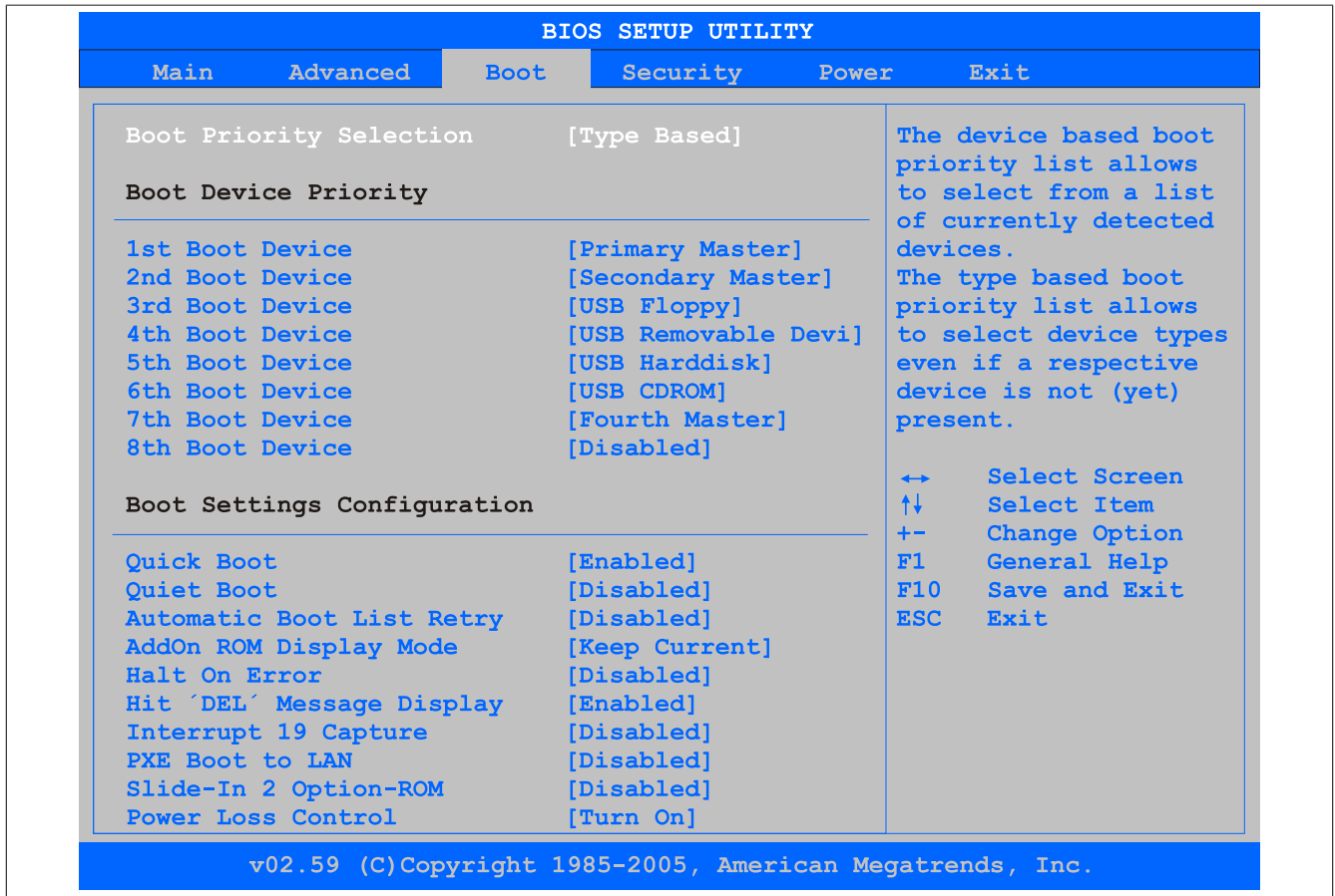
Figure 139: GM45 Boot Menü
