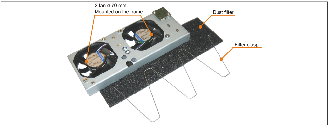
Figure 73: 5PC810.FA02-01 - Fan kit
