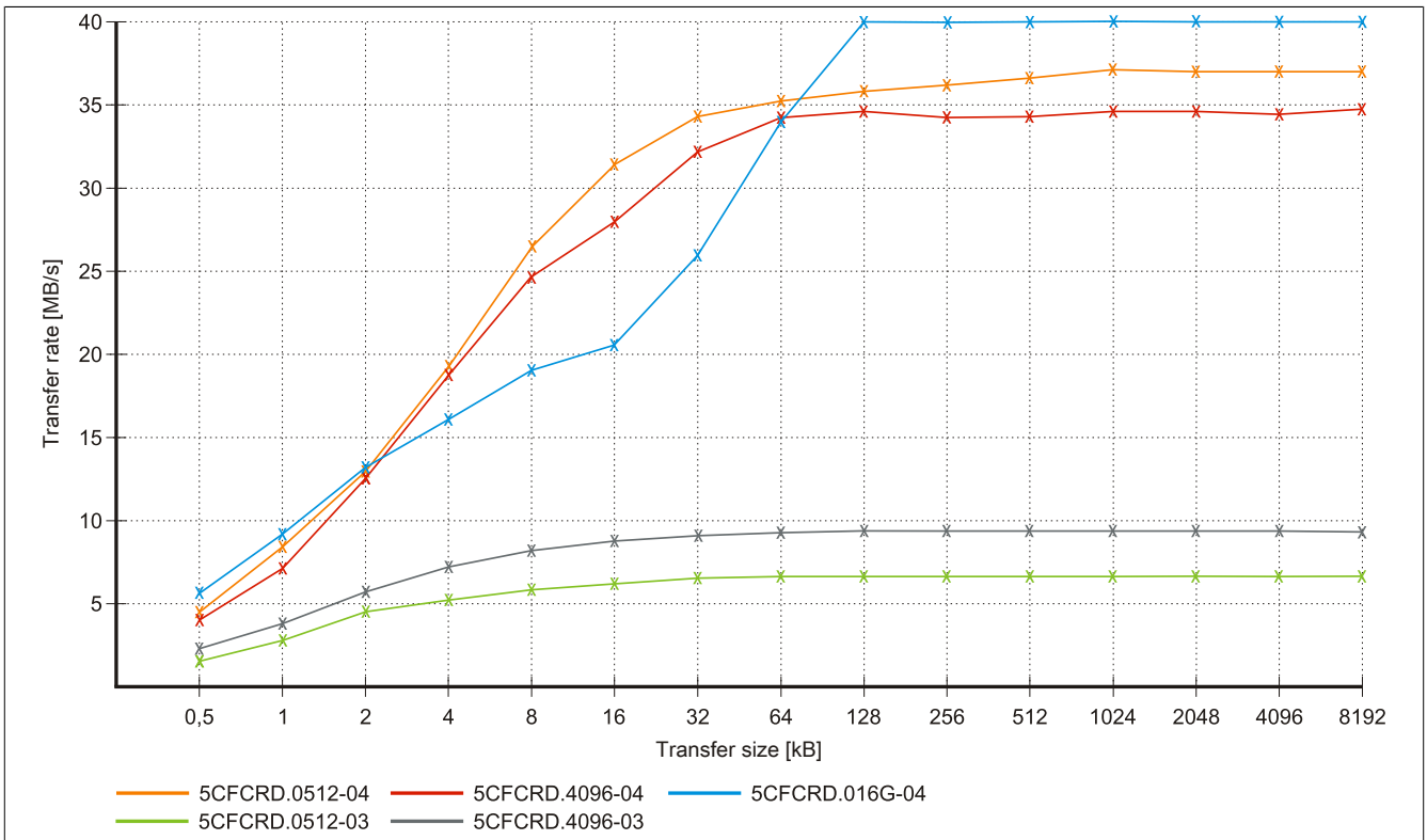
Figure 172: ATTO Disk Benchmark v2.34 read comparison - 5CFCRD.xxxx-03 and 5CFCRD.xxxx-04
