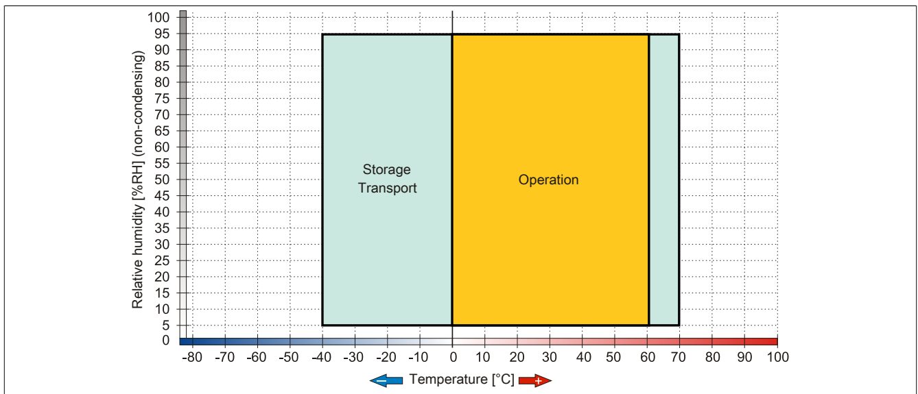
Figure 63: 5MMHDD.0250-00 - Temperature humidity diagram
