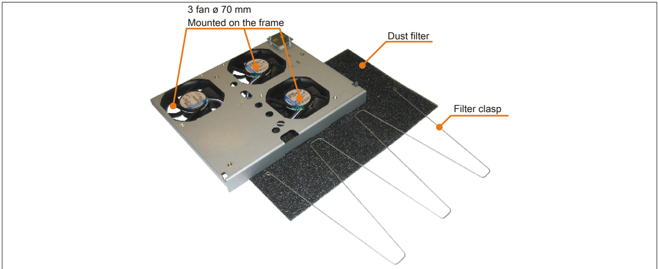
Figure 75: 5PC810.FA05-00 - Fan kit
