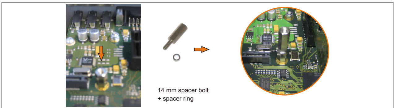
Figure 239: Screwing in the spacer bolt and spacer ring
