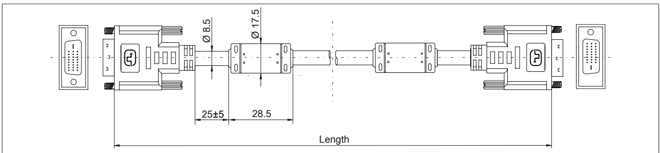
Figure 204: 5CADVI.0xxx-00 - Dimensions
