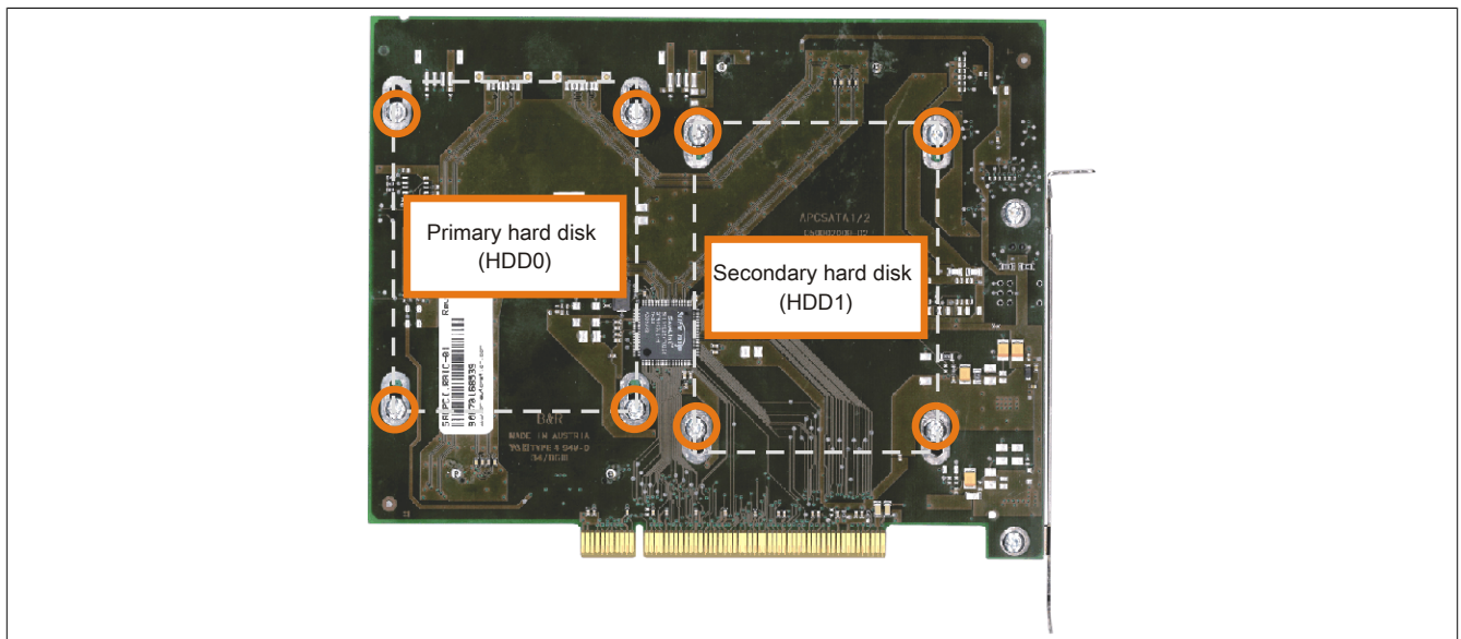
Figure 281: Screw layout on the back side of the 5ACPCI.RAIC-03 SATA RAID controller
