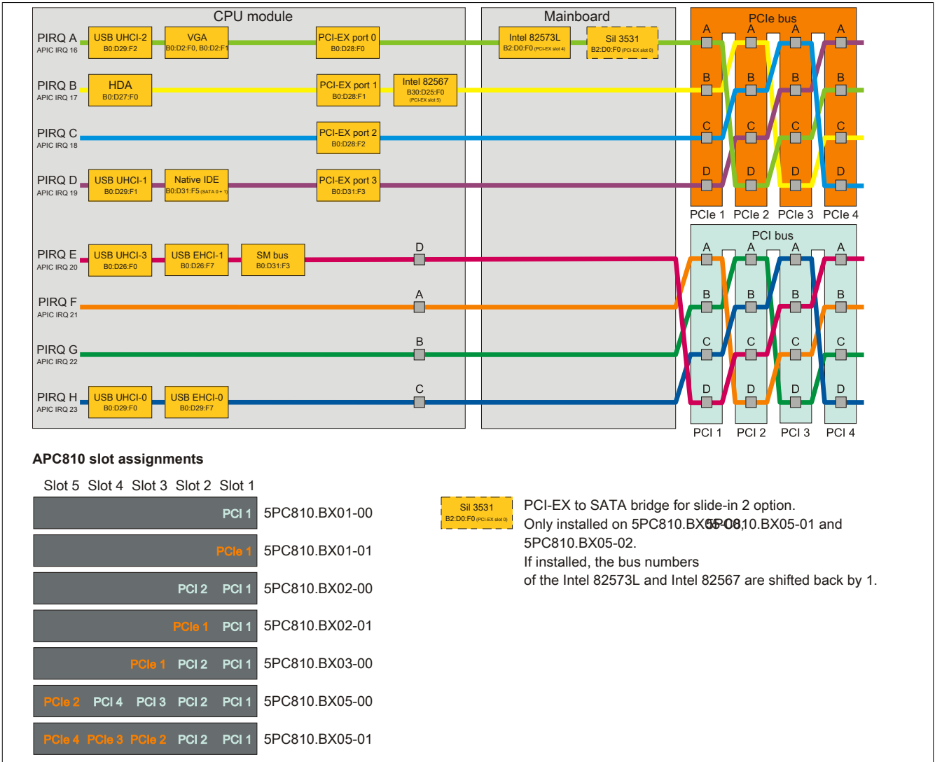
Figure 145: PCI and PCIe routing with enabled APIC for GM45 CPU boards (bus units 5PC810.BX0x-0x)
