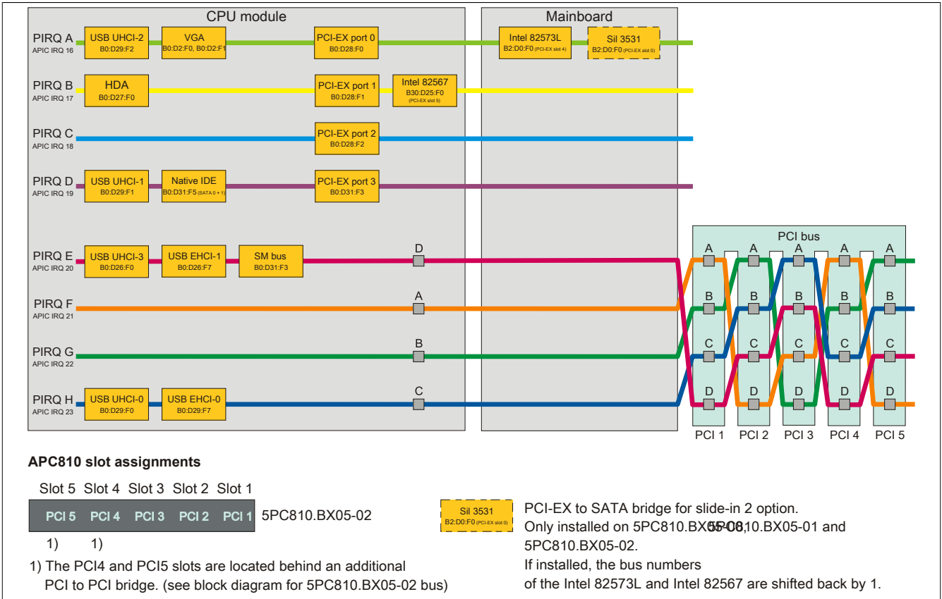
Figure 146: PCI and PCIe routing with the enabled 5PC810.BX05-02 APIC GM45 CPU board (bus unit 5PC810.BX05-02)
