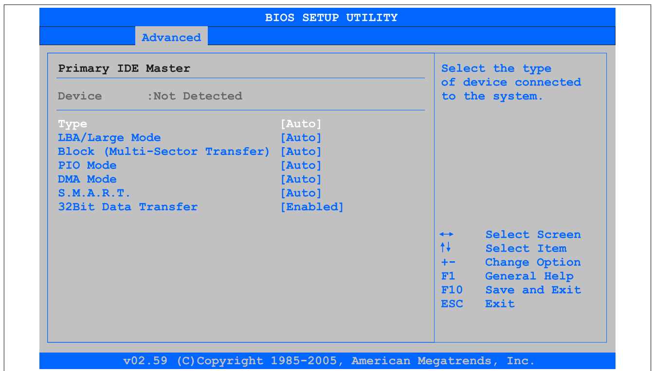
Figure 128: GM45 Primary IDE Master
