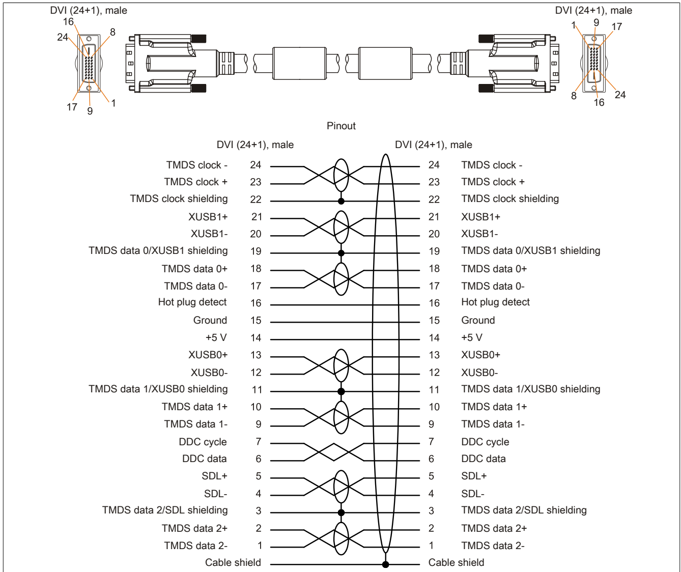
Figure 214: 5CASDL.0xxx-03 - Pinout
