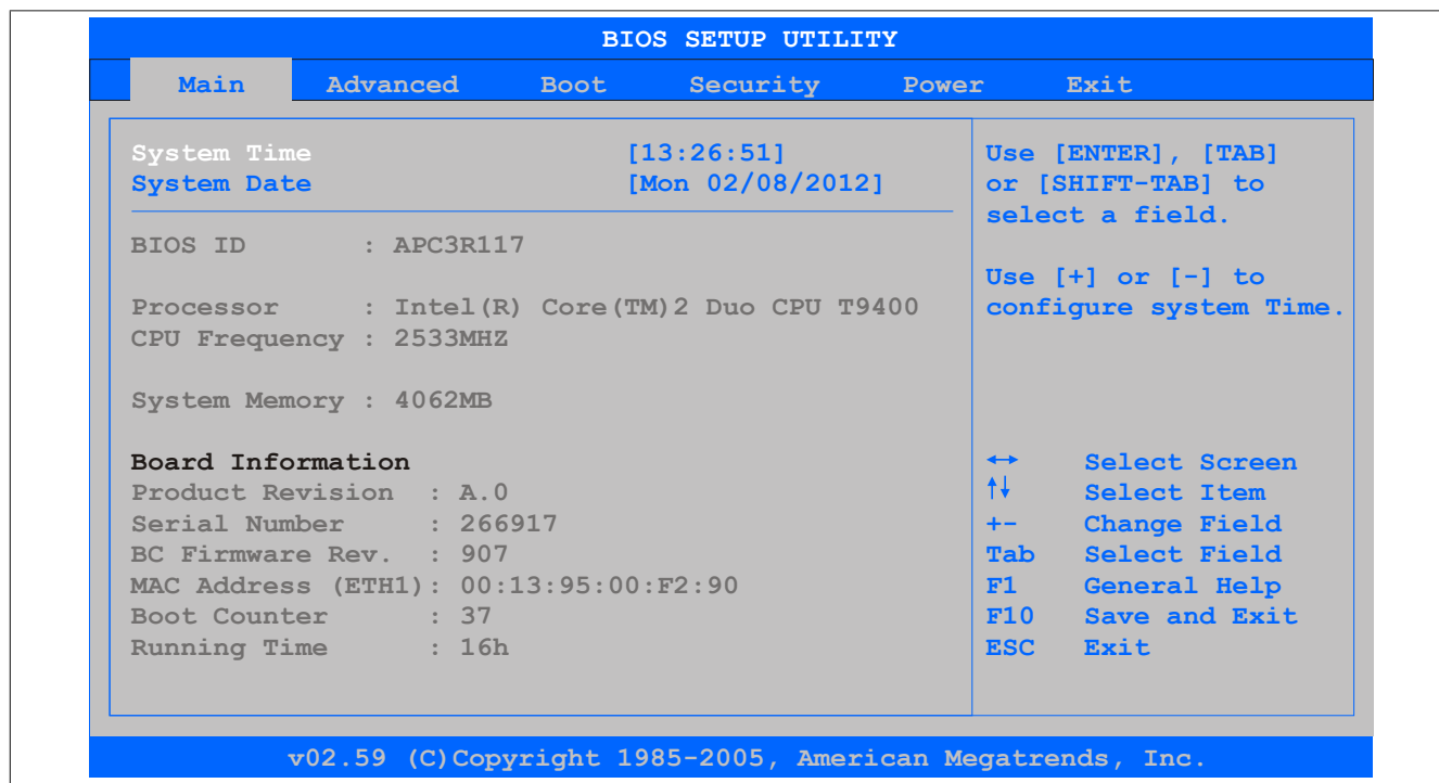
Figure 115: GM45 Main Menü
