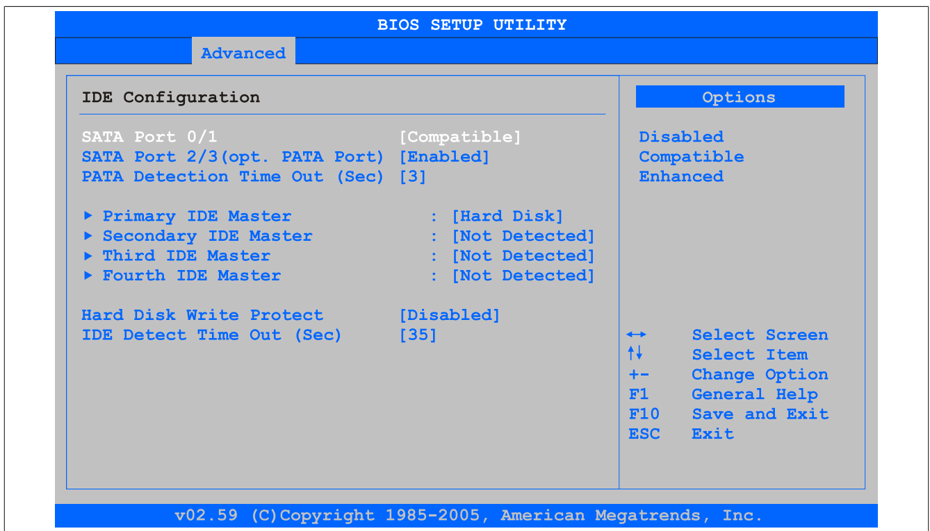
Figure 127: GM45 Advanced IDE Configuration
