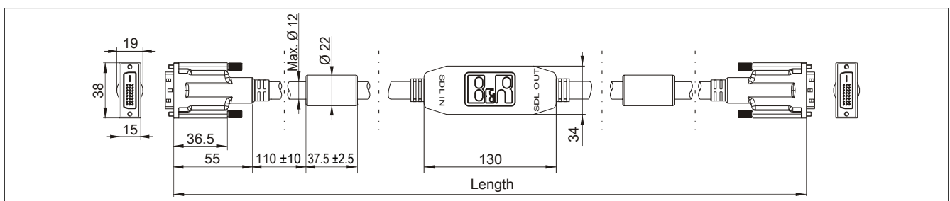
Figure 216: 5CASDL.0xx0-13 - Dimensions
