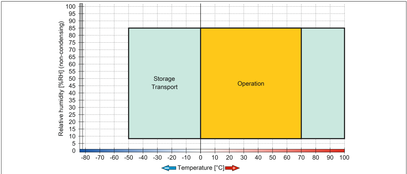
Figure 166: 5CFCRD.xxxx-06 - Temperature/Humidity diagram for CompactFlash cards
