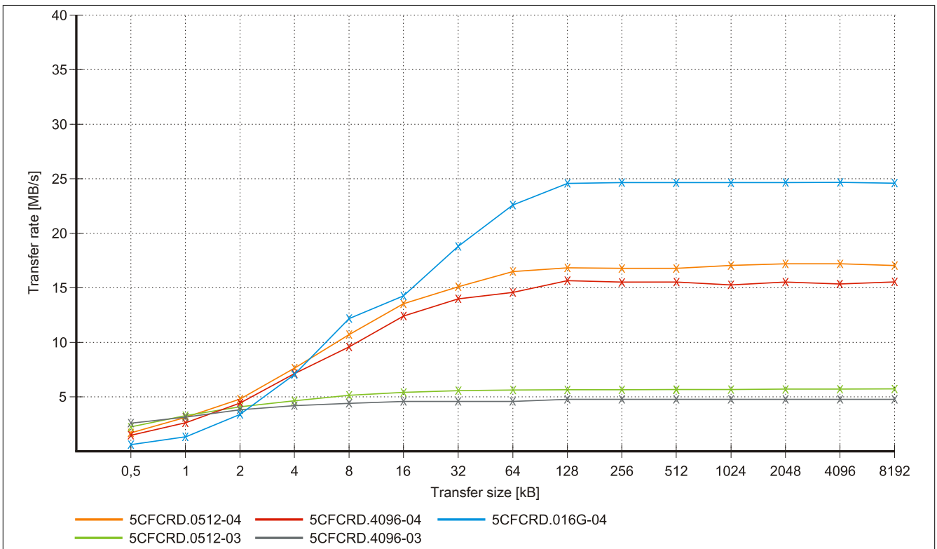
Figure 173: ATTO Disk Benchmark v2.34 write comparison - 5CFCRD.xxxx-03 and 5CFCRD.xxxx-04
