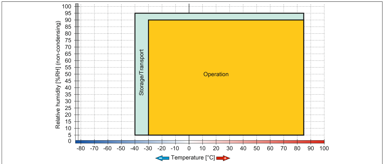
Figure 67: 5MMSSD.0060-01 ≥ Rev. D0 - Temperature/Humidity diagram
