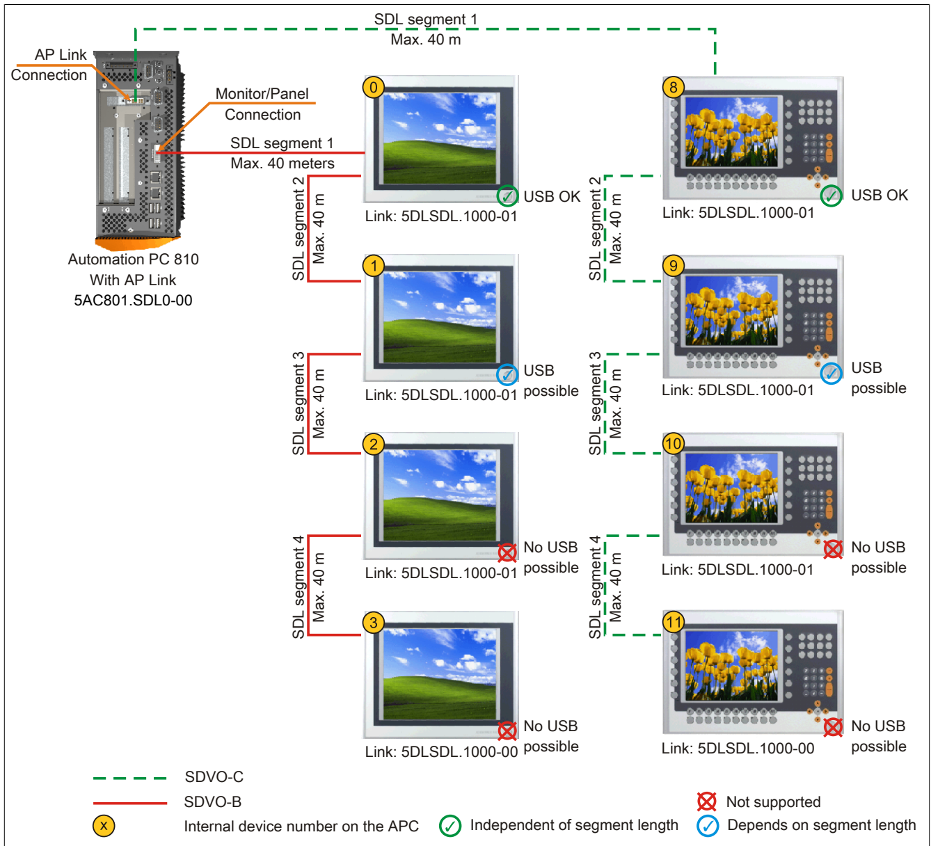
Figure 100: Eight Automation Panel 900 systems via onboard SDL and SDL AP Link
