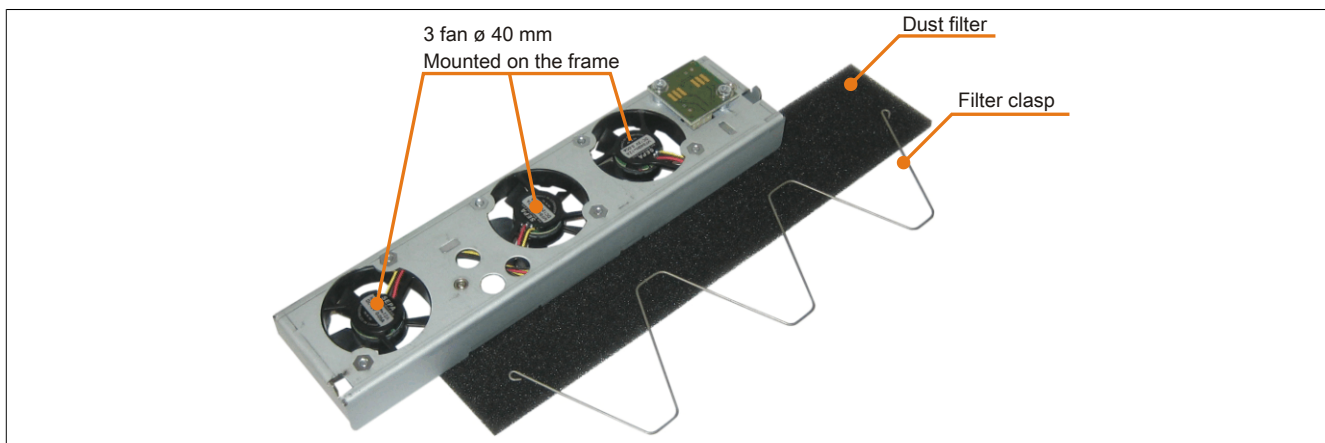
Figure 72: 5PC810.FA01-00 - Fan kit
