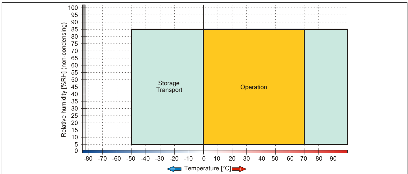
Figure 190: 5MMUSB.xxxx-01 - Temperature/Humidity diagram
