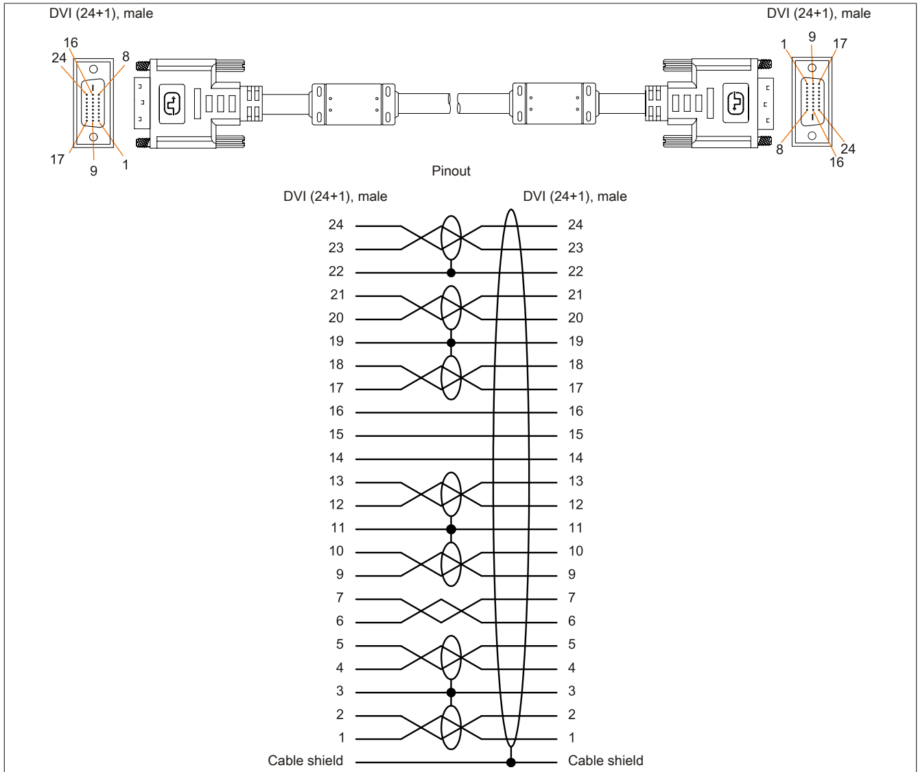
Figure 208: 5CASDL.0xxx-00 - Pinout
