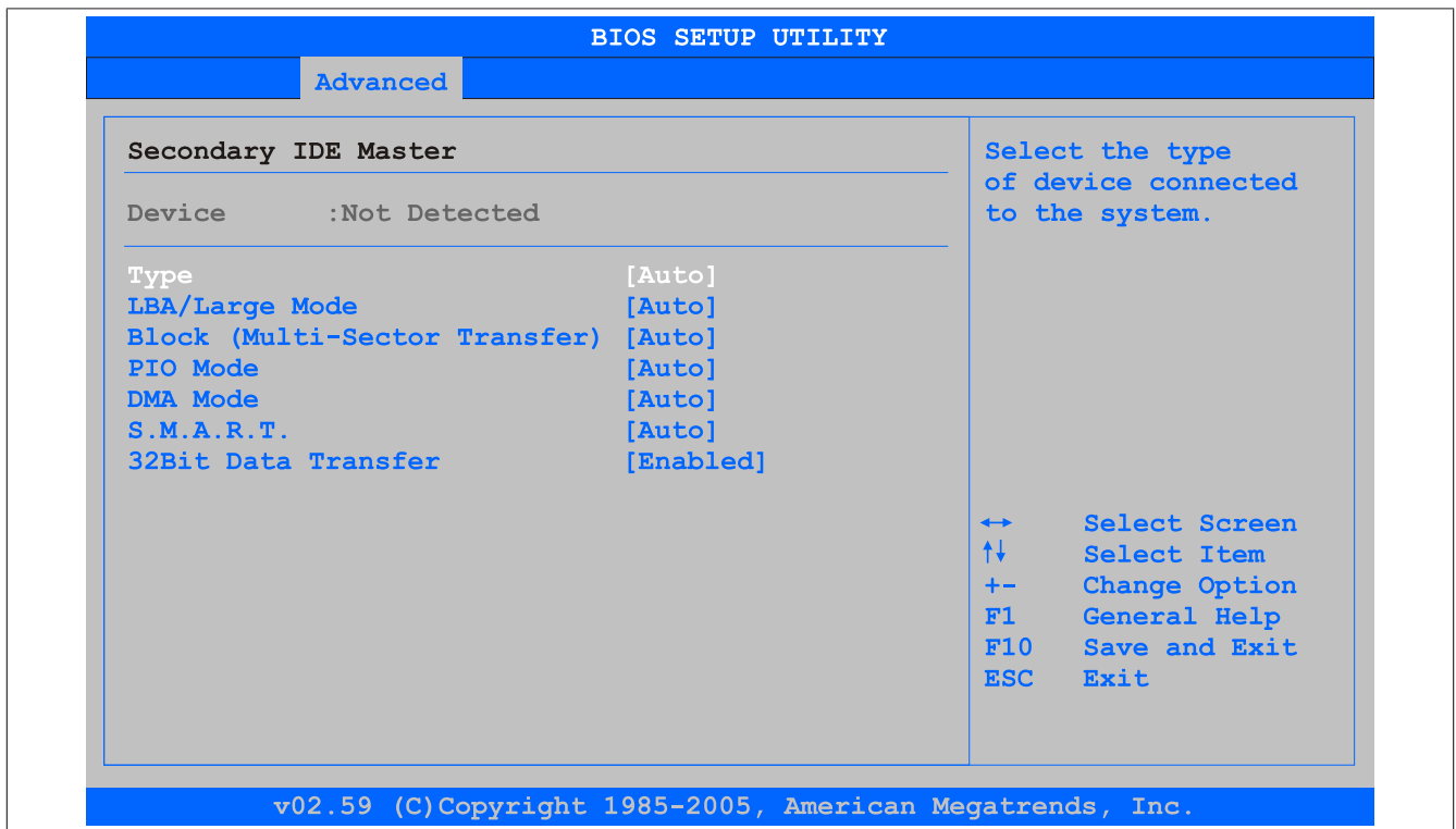
Figure 129: GM45 Secondary IDE Master
