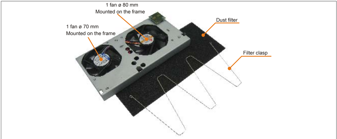
Figure 74: 5PC810.FA03-00 - Fan kit
