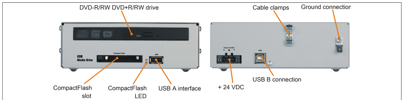
Figure 181: 5MD900.USB2-02 - Interfaces
