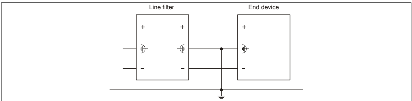
Figure 198: Connection example
