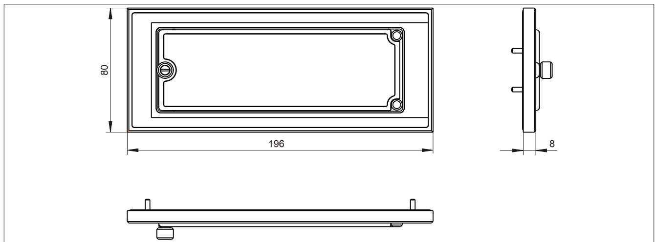
Figure 186: 5A5003.03 - Dimensions
