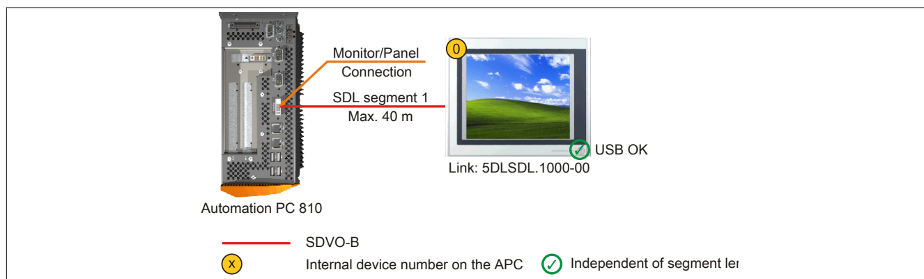
Figure 93: One Automation Panel 900 system via onboard SDL
