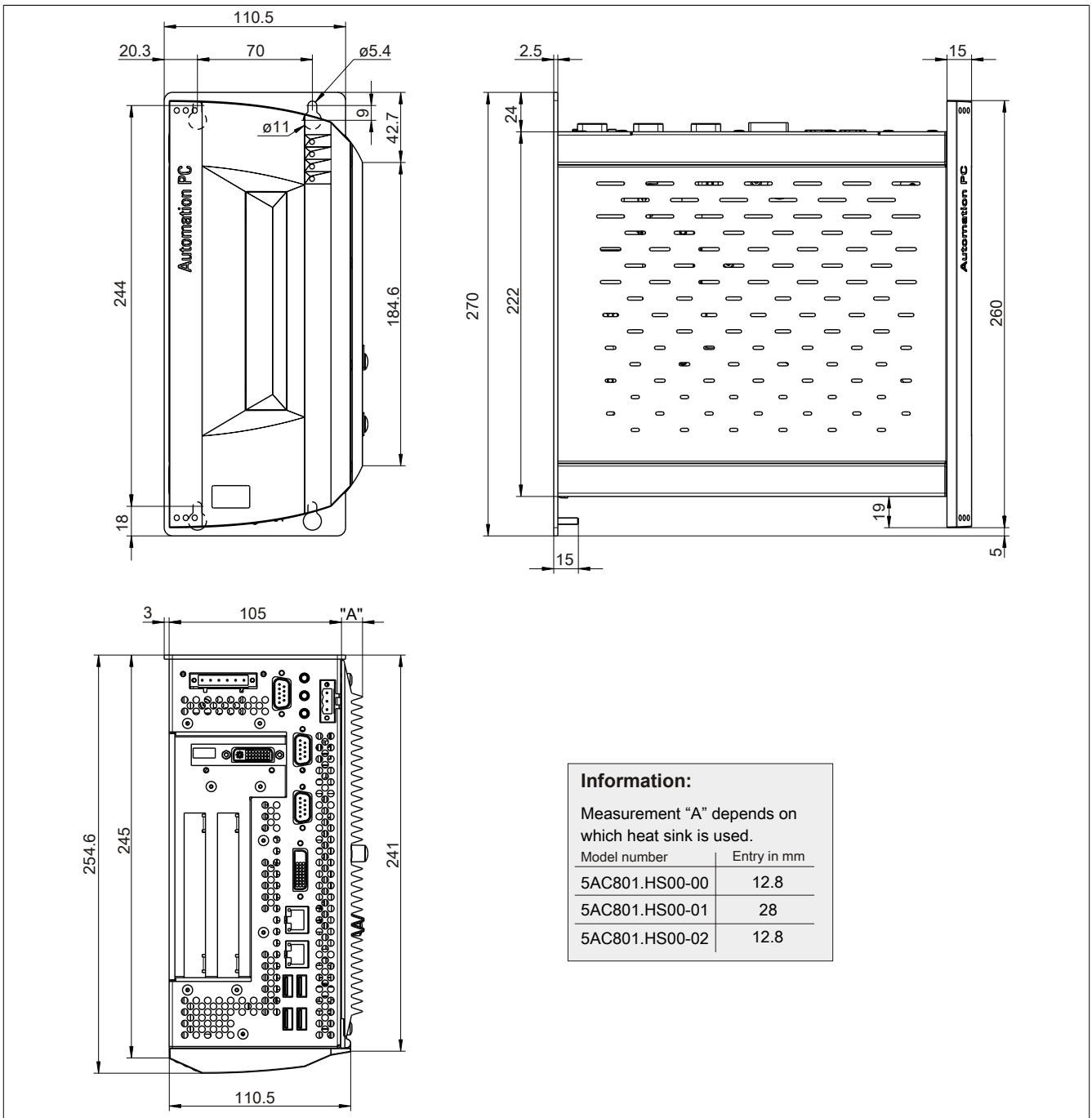
Figure 25: 5PC810.SX02-00 - Dimensions
