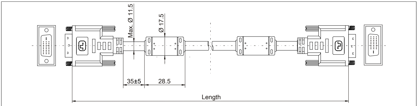
Figure 207: 5CASDL.0xxx-00- Dimensions
