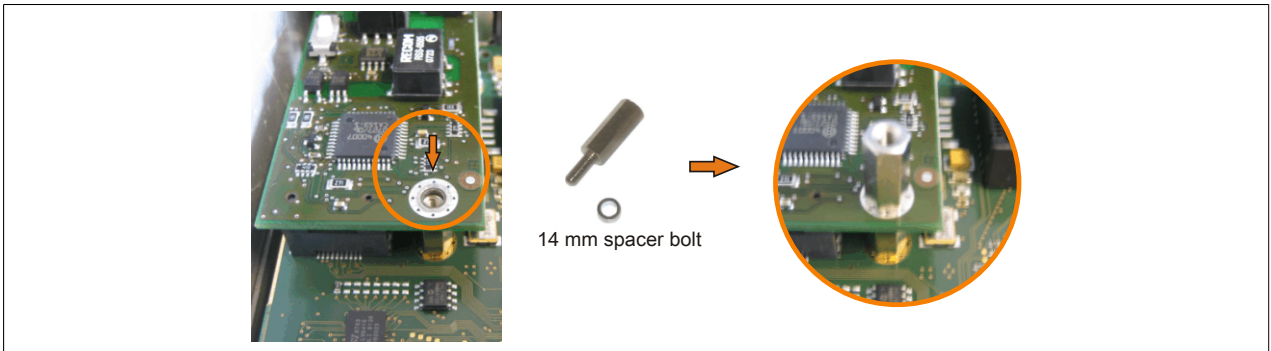
Figure 256: Screwing in the spacer bolt
