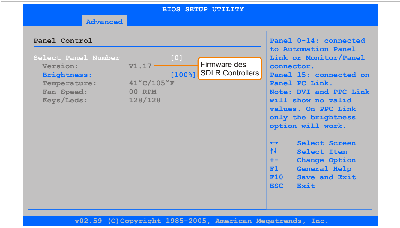
Figure 148: Firmwareversion des AP Link SDL Transmitter
