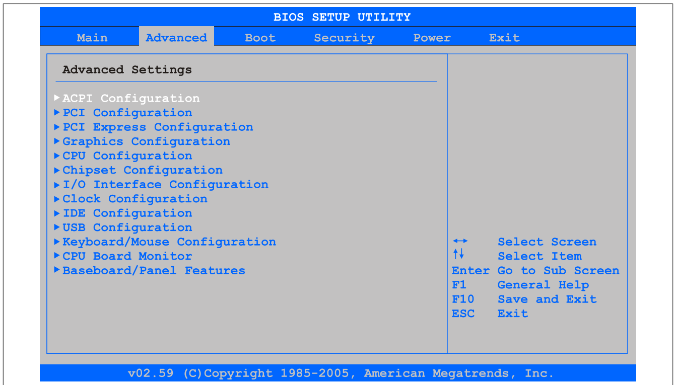
Figure 116: GM45 Advanced Menü
