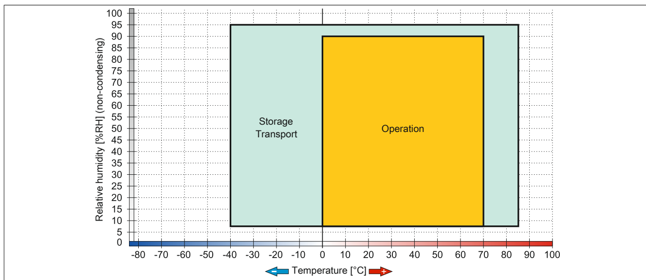
Figure 48: 5AC801.SSDI-03 ≤ Rev. C0 - Temperature/Humidity diagram
