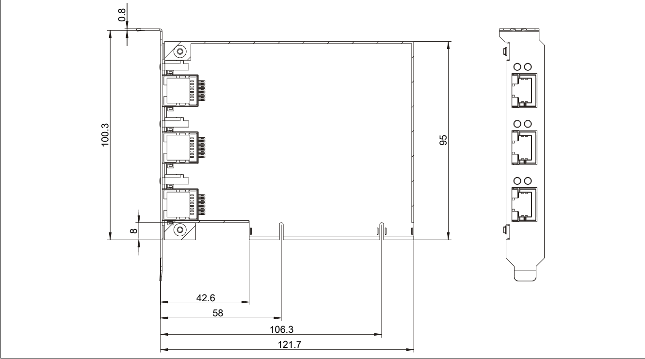
Figure 202: 5ACPCI.ETH3-01 - Dimensions
