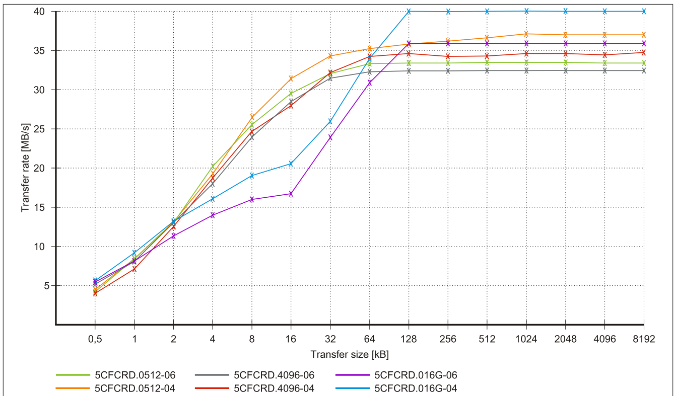
Figure 168: ATTO Disk Benchmark v2.34 read comparison - 5CFCRD.xxxx-04 and 5CFCRD.xxxx-06
