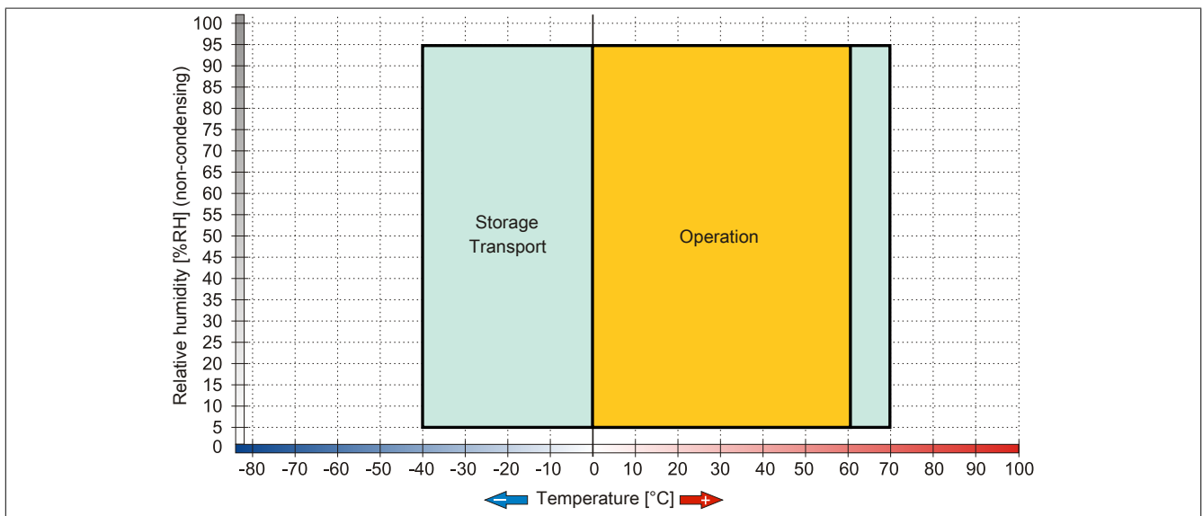
Figure 64: 5MMHDD.0500-00 - Temperature humidity diagram
