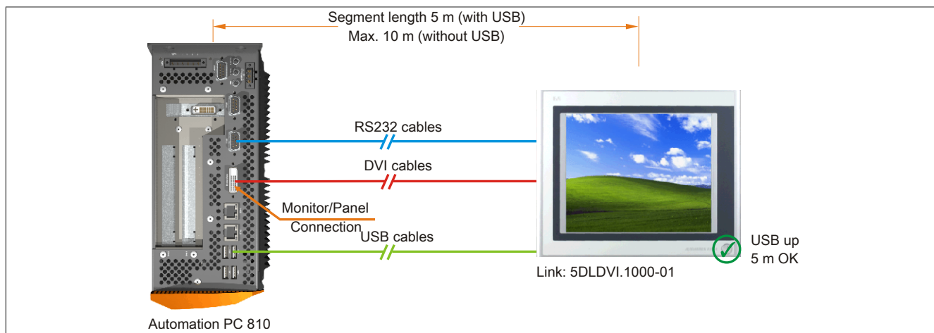
Figure 92: One Automation Panel 900 system via onboard DVI
