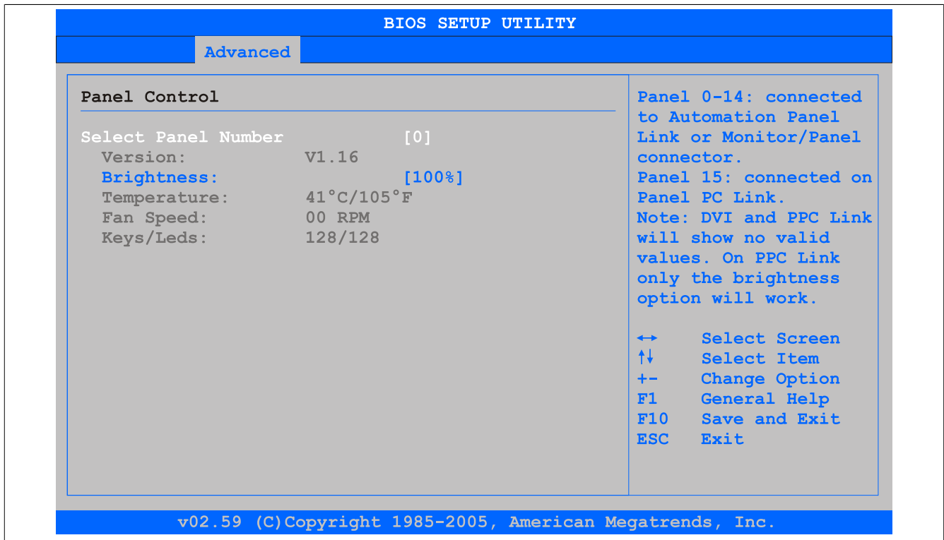
Figure 136: GM45 Panel Control
