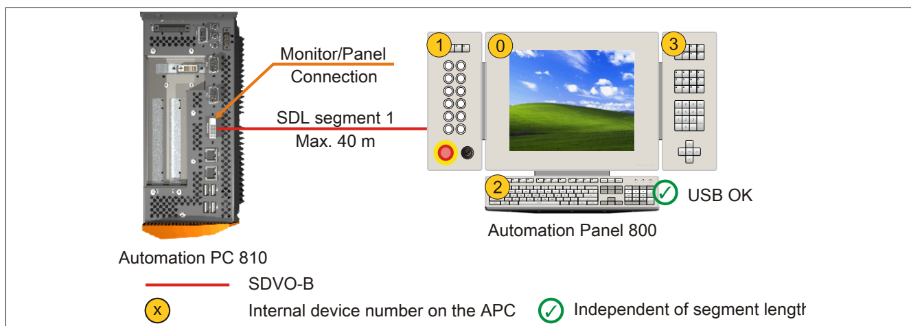
Figure 94: One Automation Panel 800 system via onboard SDL
