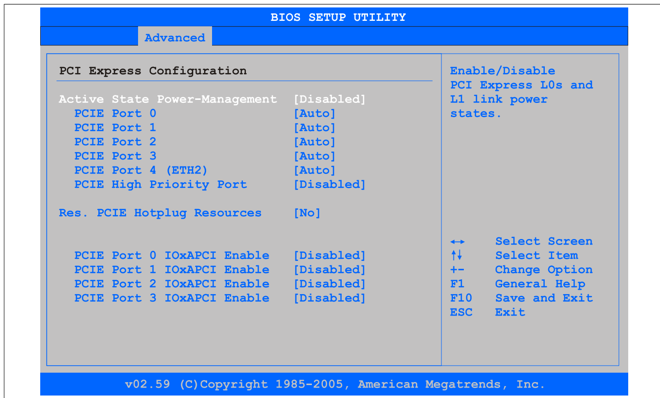
Figure 121: GM45 Advanced PCI Express Configuration
