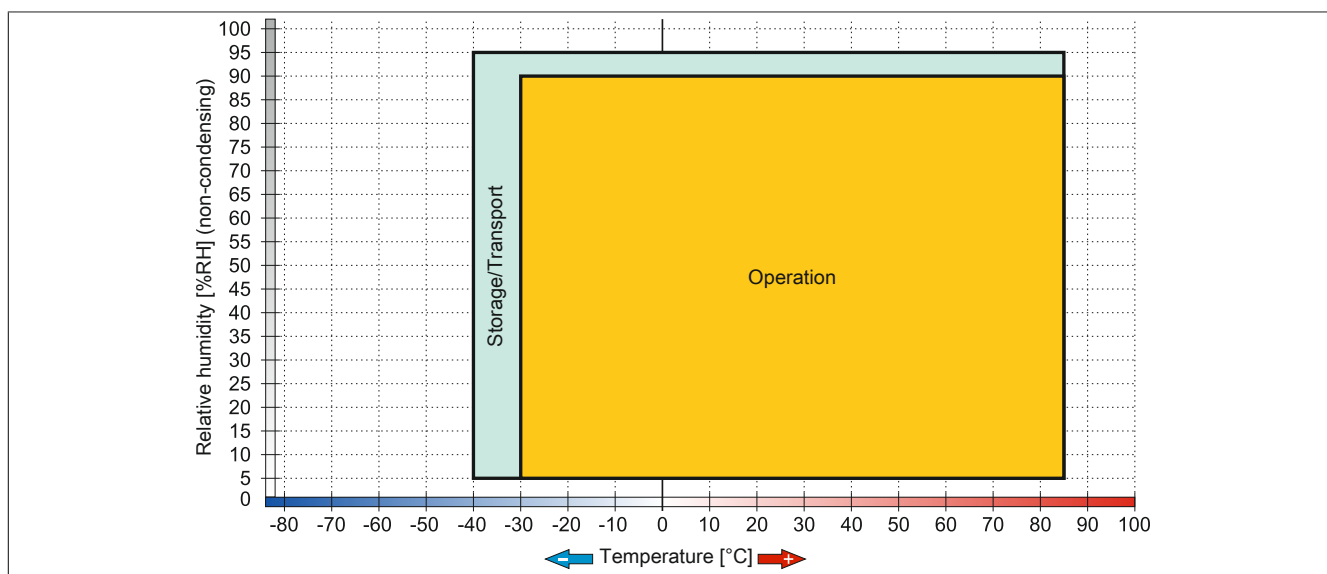
Figure 52: 5AC801.SSDI-05 - Temperature humidity diagram
