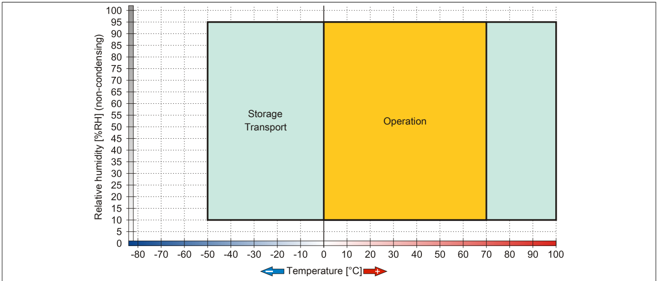
Figure 174: 5CFCRD.xxxx-03 - Temperature/Humidity diagram for CompactFlash cards
