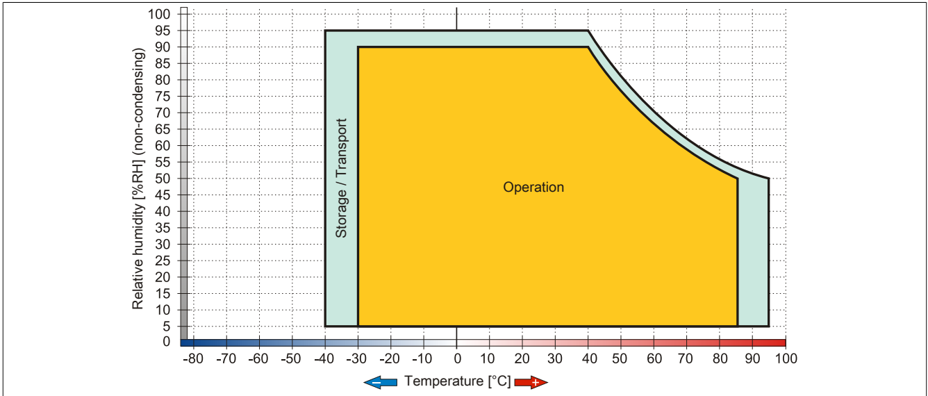
Figure 57: 5ACPCI.RAIC-03 - Temperature humidity diagram
