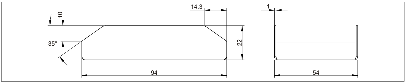
Figure 196: 5AC804.MFLT-00 - Dimensions
