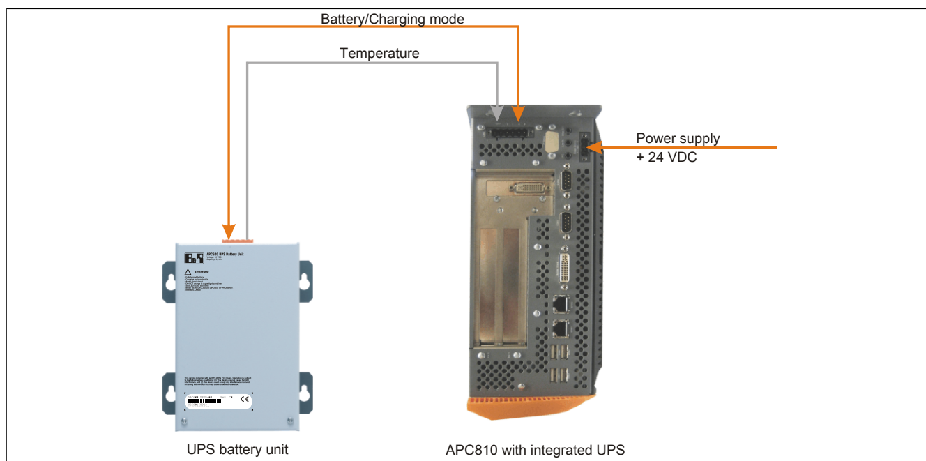
Figure 191: UPS principle
