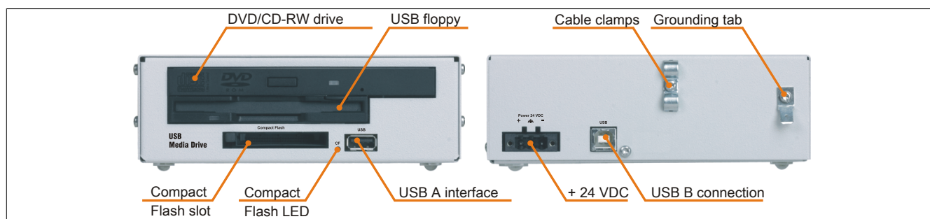
Figure 176: 5MD900.USB2-01 - Interfaces
