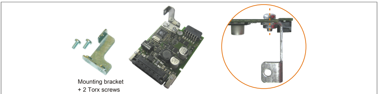
Figure 245: Installing the mounting bracket
