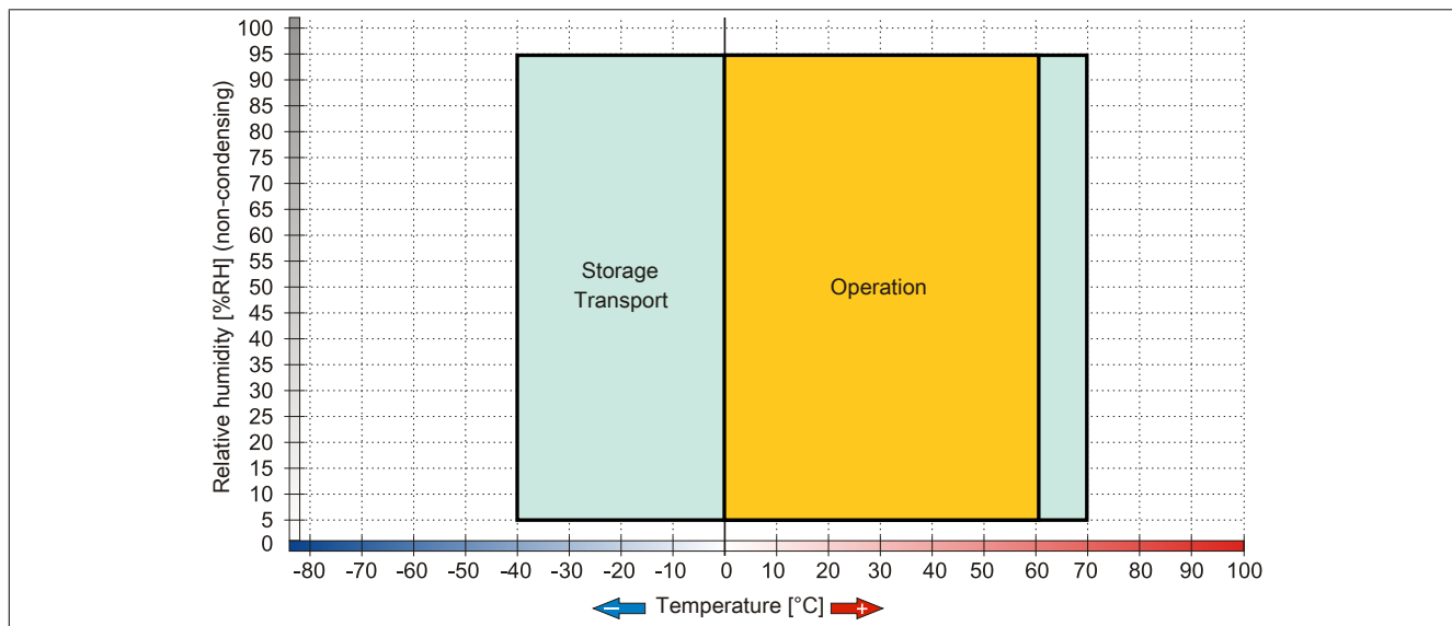
Figure 60: 5ACPCI.RAIC-05 - Temperature humidity diagram
