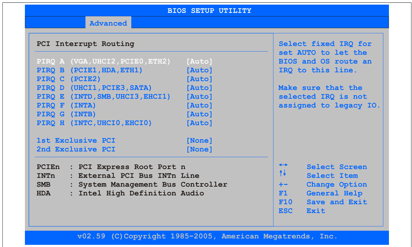
Figure 120: GM45 Advanced PCI Interrupt Routing
