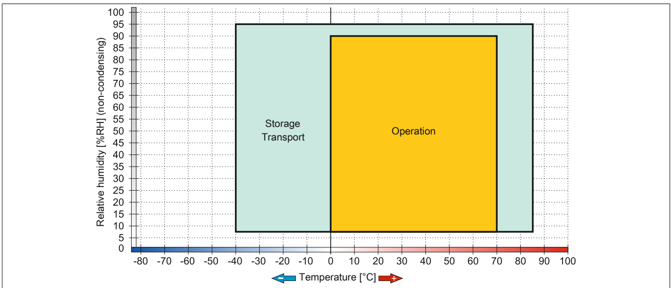
Figure 66: 5MMSSD.0060-01 ≤ Rev. C0 - Temperature/Humidity diagram
