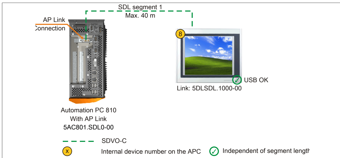
Figure 97: One Automation Panel 900 system via SDL AP Link
