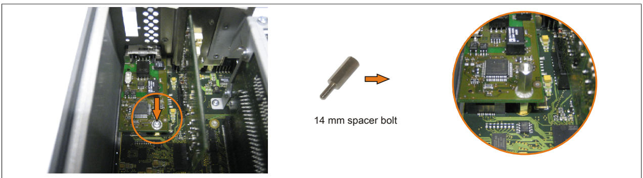
Figure 261: Screwing in the spacer bolt
