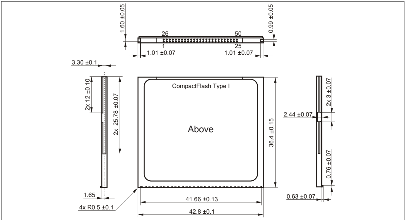
Figure 167: Type I CompactFlash card - Dimensions
