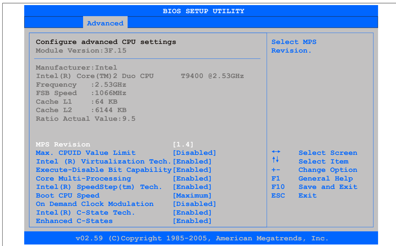
Figure 123: GM45 Advanced CPU Board Monitor
