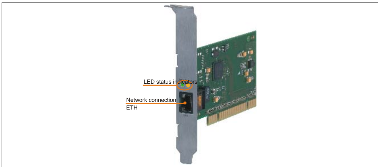
Figure 199: 5ACPCI.ETH1-01 - PCI 10/100 Ethernet card
