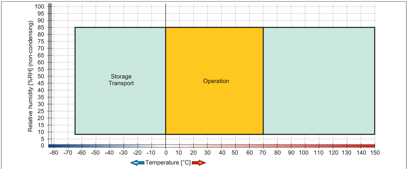
Figure 170: 5CFCRD.xxxx-04 - Temperature/Humidity diagram for CompactFlash cards
