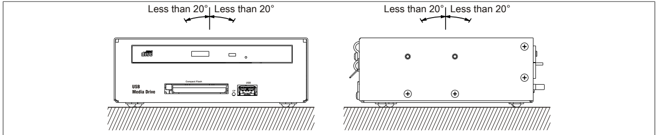
Figure 185: 5MD900.USB2-02 - Mounting orientation
