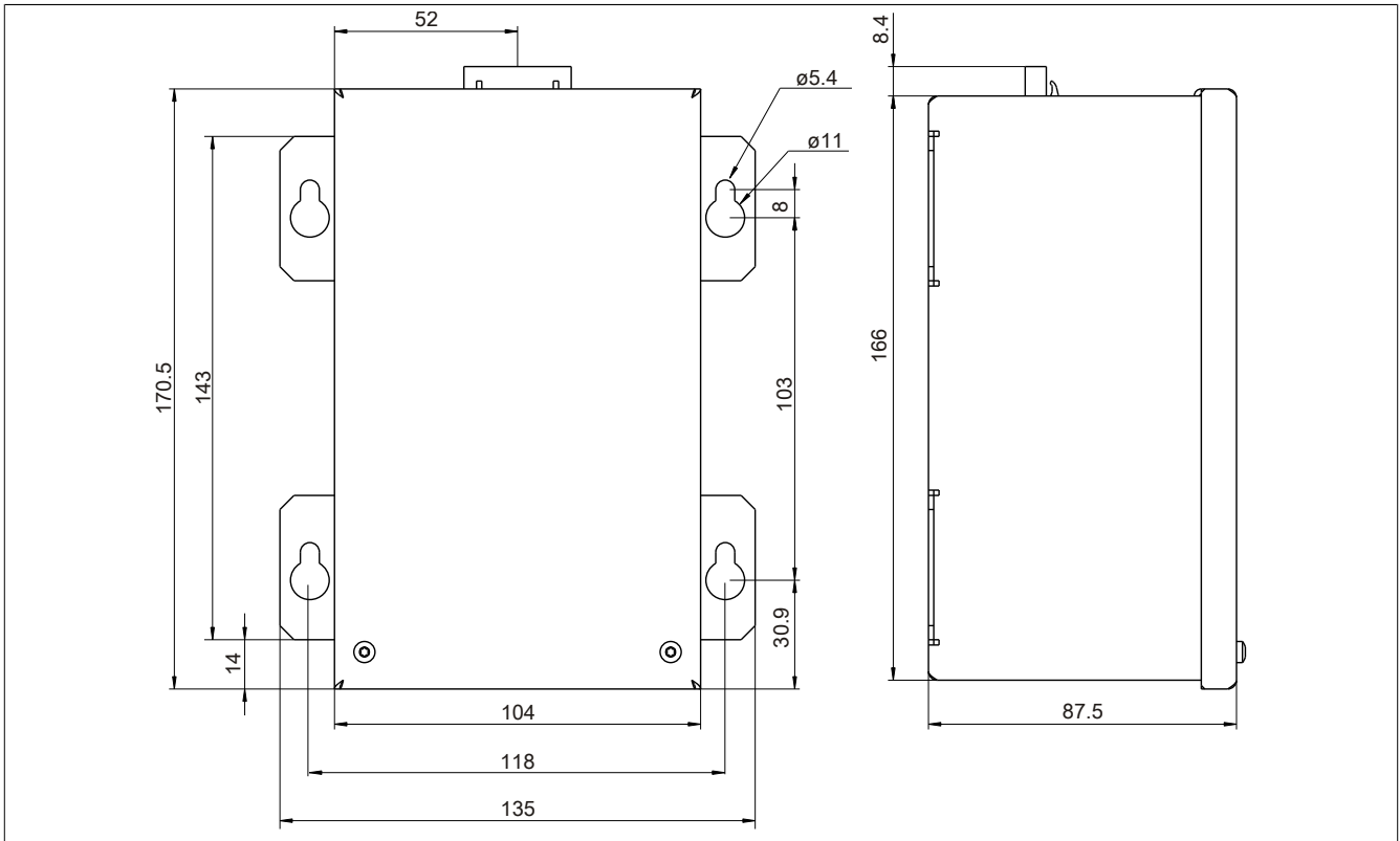
Figure 194: 5PC600.UPSB-00 - Dimensions
