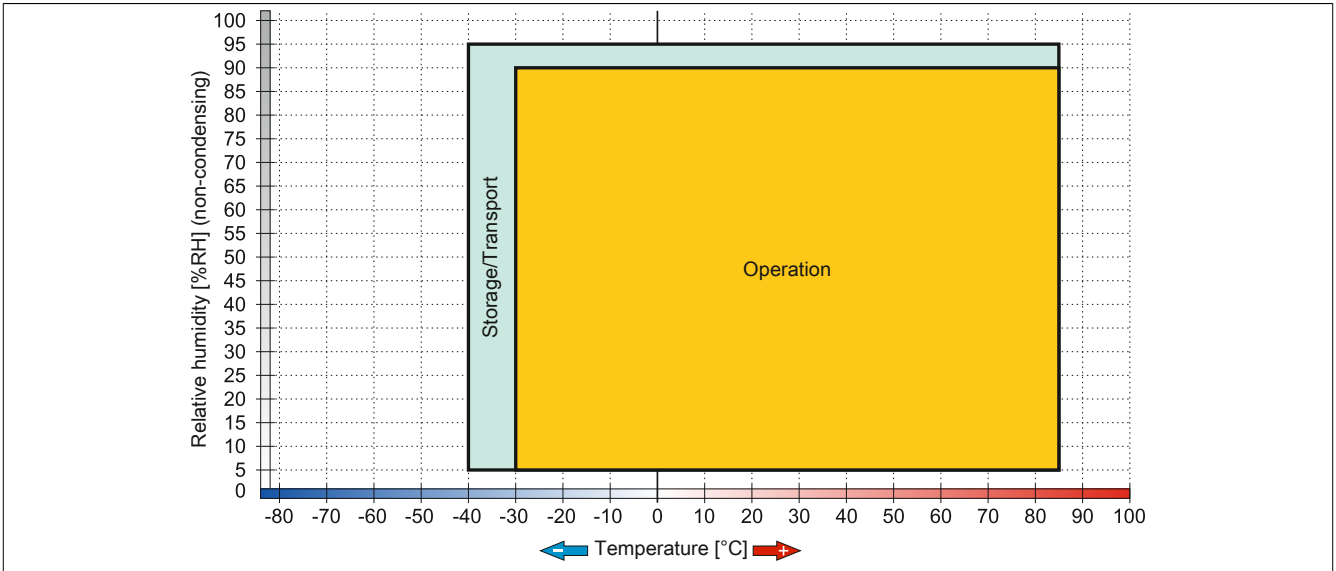
Figure 69: 5MMSSD.0128-01 ≥ Rev. D0 - Temperature/Humidity diagram
