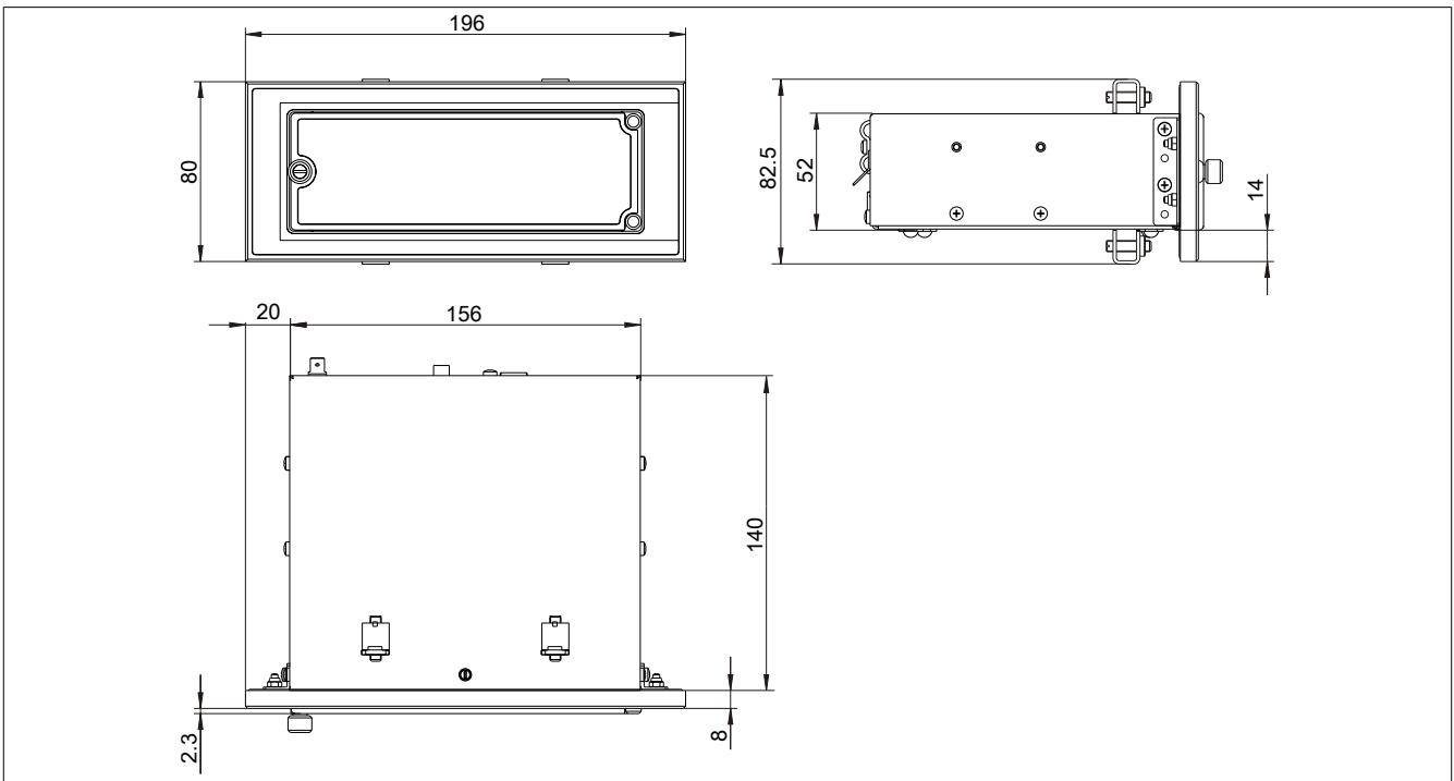
Figure 183: USB media drive with front cover - Dimensions
