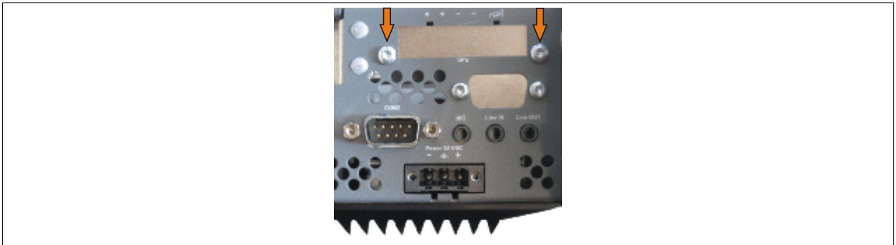
Figure 238: Removing the UPS module cover
