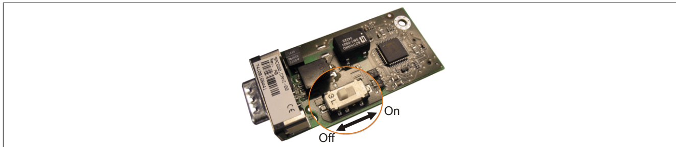
Figure 80: 5AC600.CANI-00 - Terminating resistor for add-on CAN interface
