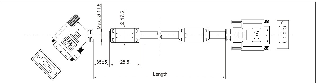
Figure 210: 5CASDL.0xxx-01 - Dimensions
