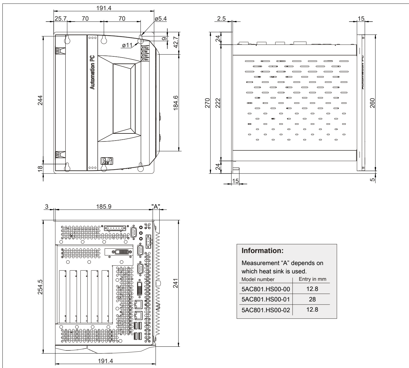
Figure 33: 5PC810.SX05-00 - Dimensions
