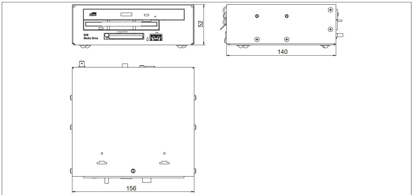
Figure 177: 5MD900.USB2-01 - Dimensions
