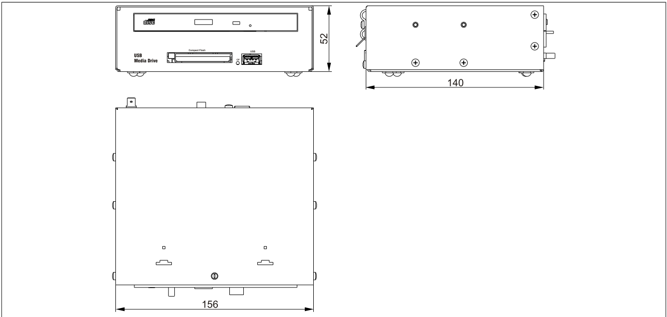
Figure 182: 5MD900.USB2-02 - Dimensions
