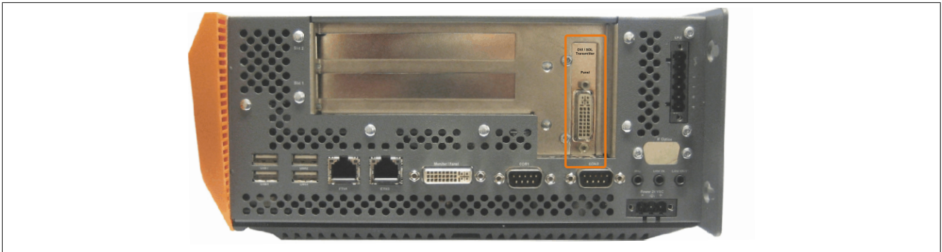
Figure 76: 5PC810.SX02-00 - Installation example in system unit
