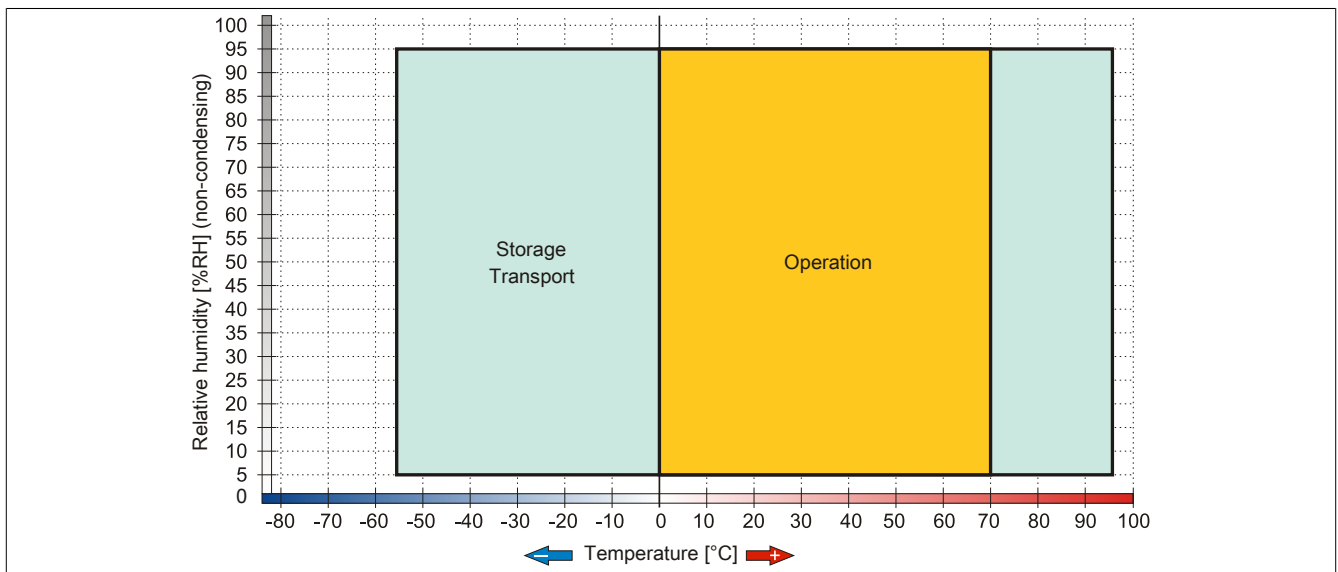
Figure 70: 5MMSSD.0180-00 - Temperature humidity diagram
