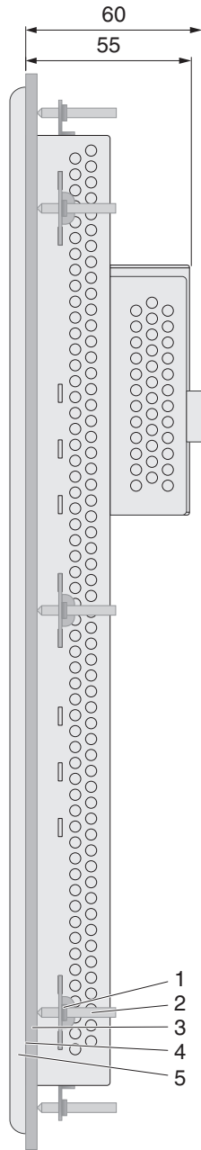
Figure 2-27 Side view, mounting depth (dimensions in mm)
