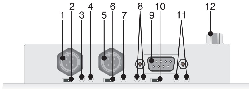
Figure 4-4 Rear view CAN
