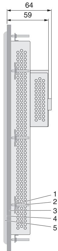
Figure 2-28 Side view, mounting depth (dimensions in mm)
