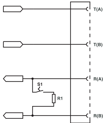
Figure 4-7 Termination possibilities RS-422 / RS-485 (intern)
