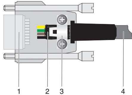
Figure 4-9 Shielding D-SUB connectors
