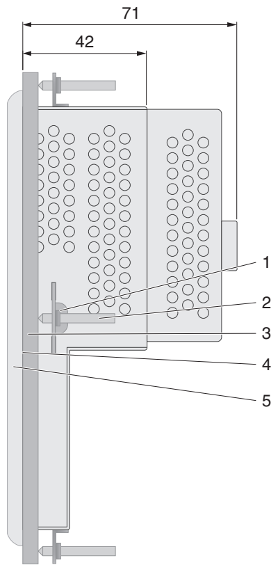
Figure 2-22 Side view, mounting depth (dimensions in mm)
