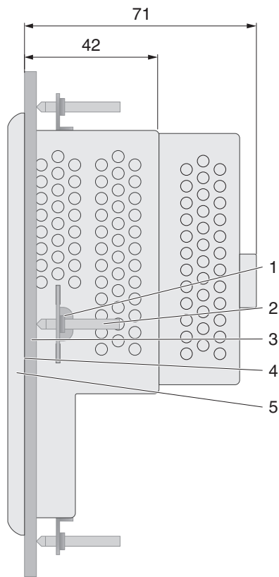
Figure 2-21 Side view, mounting depth (dimensions in mm)
