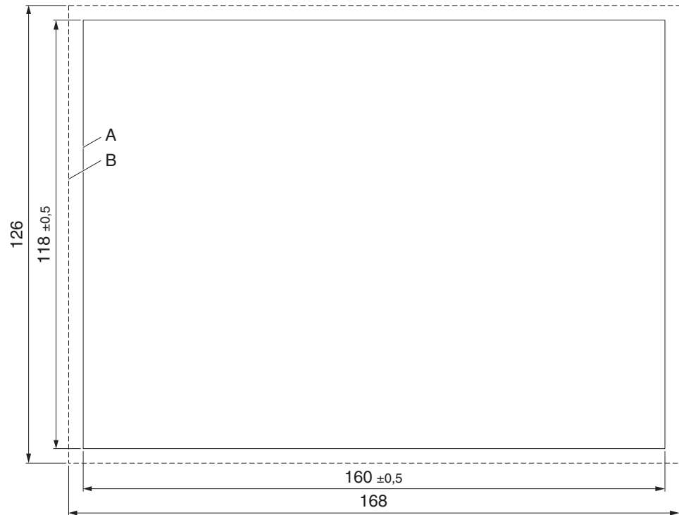
Figure 2-12 Mounting cutout (dimensions in mm)
