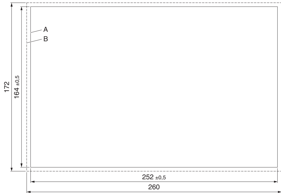
Figure 2-14 Mounting cutout (dimensions in mm)
