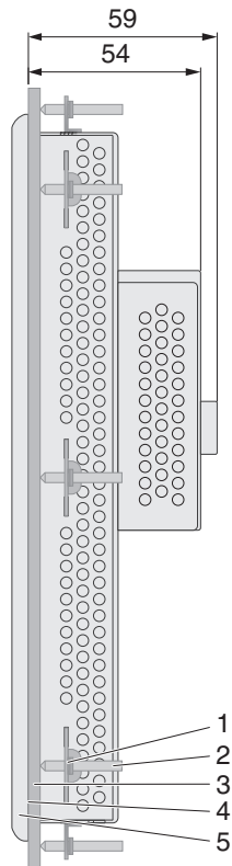
Figure 2-24 Side view, mounting depth (dimensions in mm)
