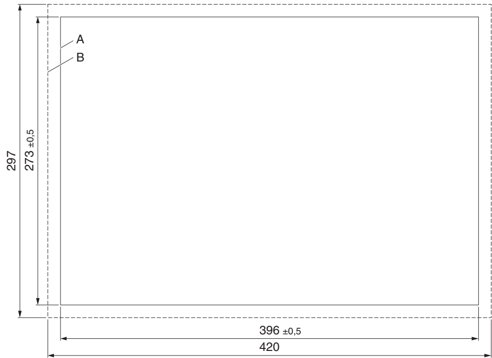
Figure 2-19 Mounting cutout (dimensions in mm)
