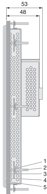
Figure 2-26 Side view, mounting depth (dimensions in mm)
