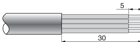
Figure 2-29 Preparing the cable
