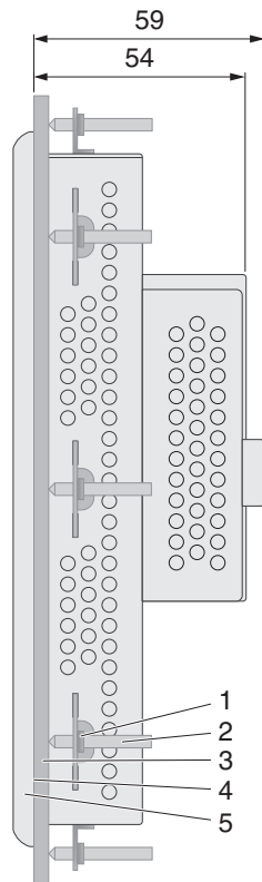
Figure 2-23 Side view, mounting depth (dimensions in mm)
