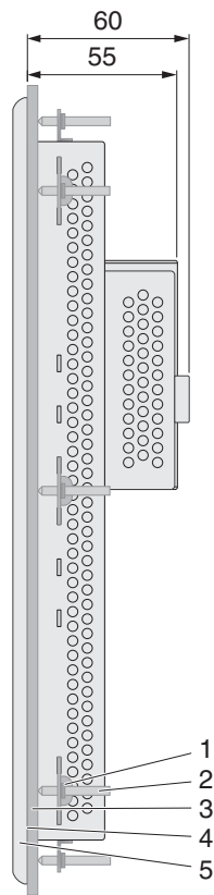
Figure 2-25 Side view, mounting depth (dimensions in mm)
