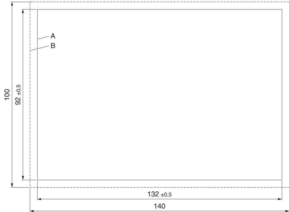
Figure 2-11 Mounting cutout (dimensions in mm)
