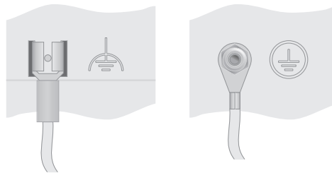
Figure 2-30 Noiseless ground / protective ground
