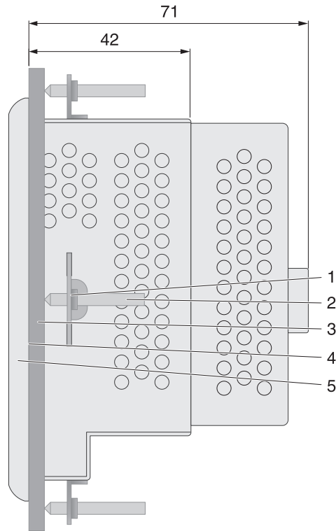
Figure 2-20 Side view, mounting depth (dimensions in mm)
