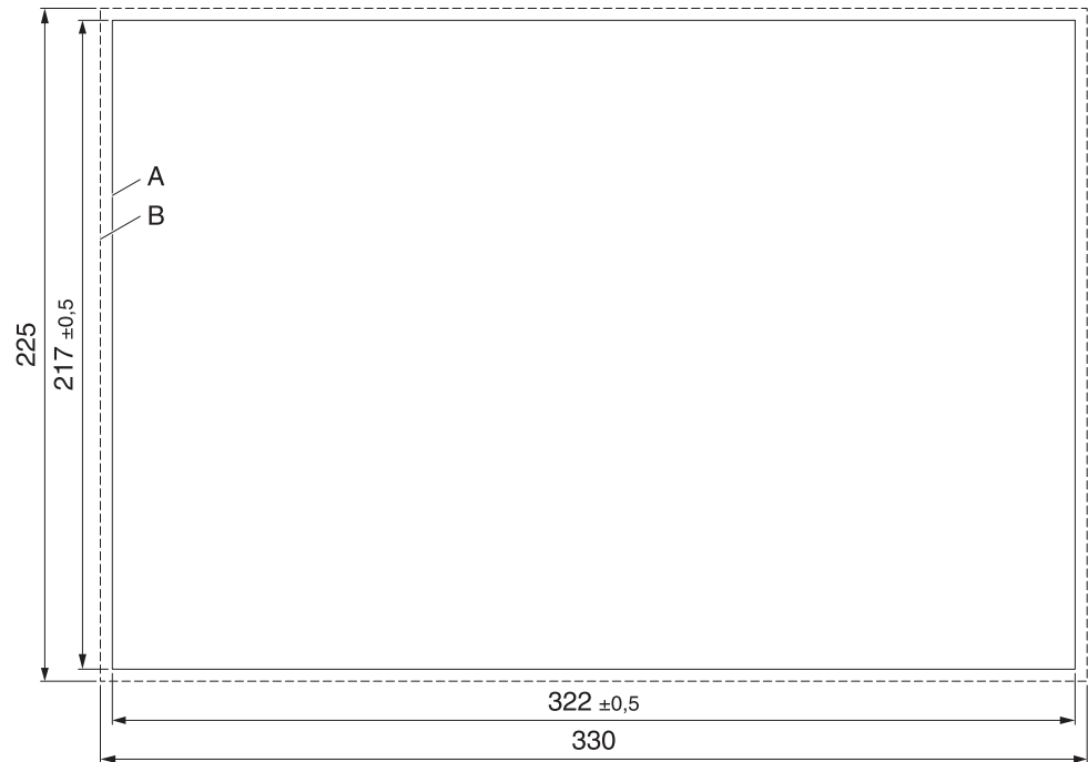
Figure 2-17 Mounting cutout (dimensions in mm)
