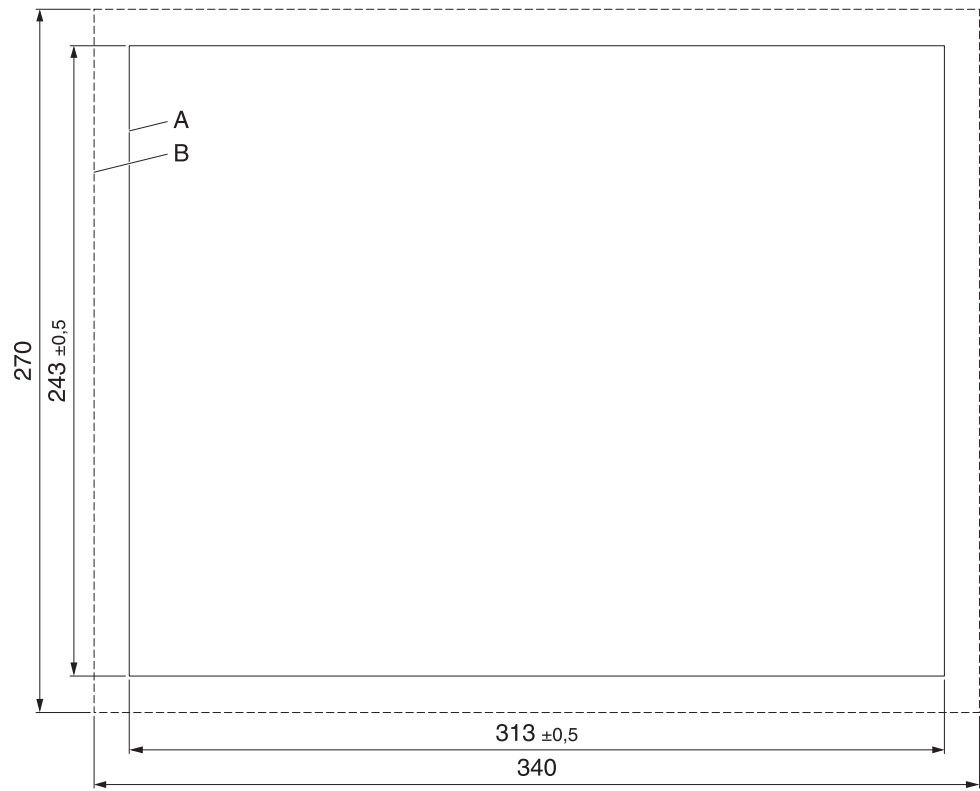
Figure 2-16 Mounting cutout (dimensions in mm)
