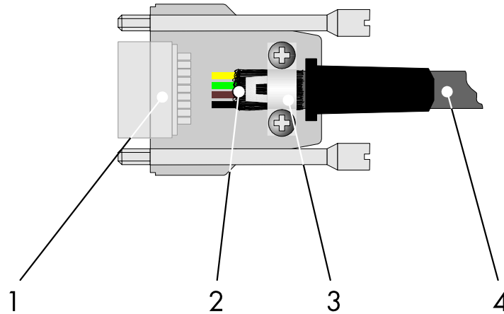
Figure 4-16 Shielding D-SUB connectors
