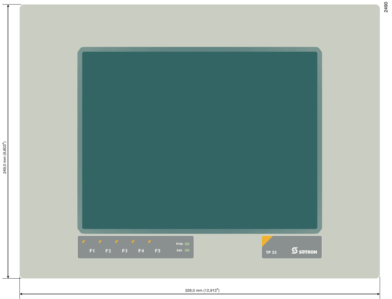
Figure 2-1 Front panel dimensions
