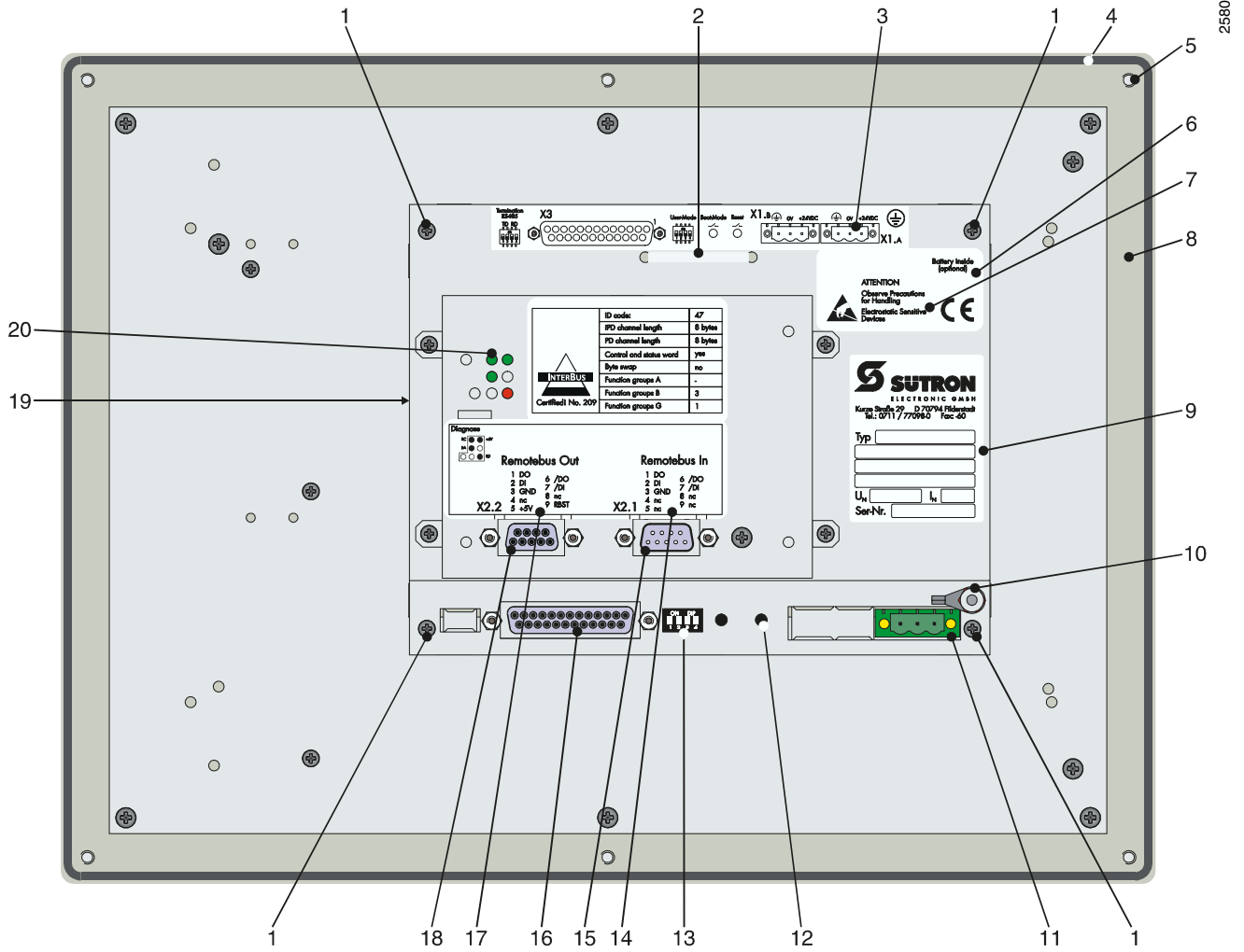
Figure 4-6 Rear view INTERBUS
