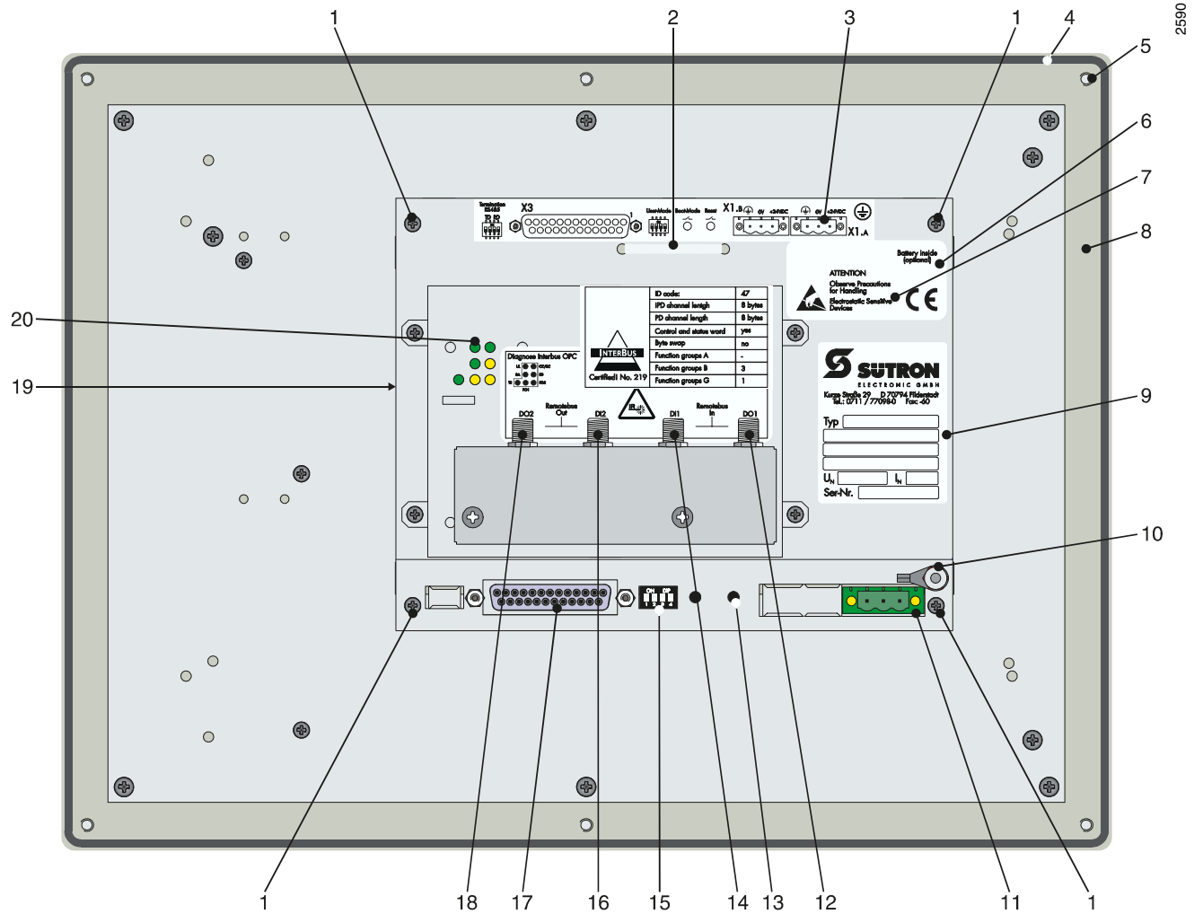
Figure 4-8 Rear view INTERBUS OPC LWL
