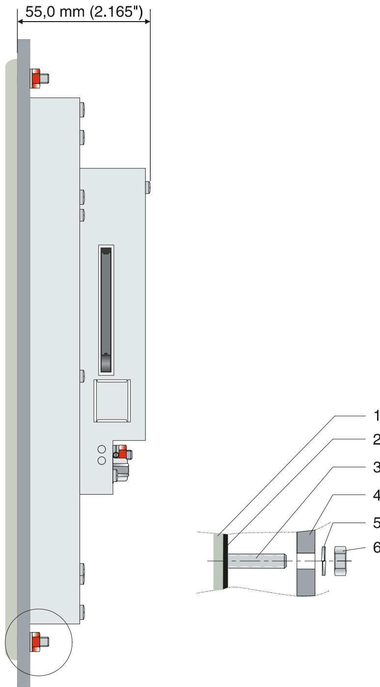
Figure 2-3 Side view and mounting depth for the standard device
