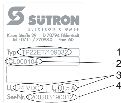
Figure 2-8 Nameplate
