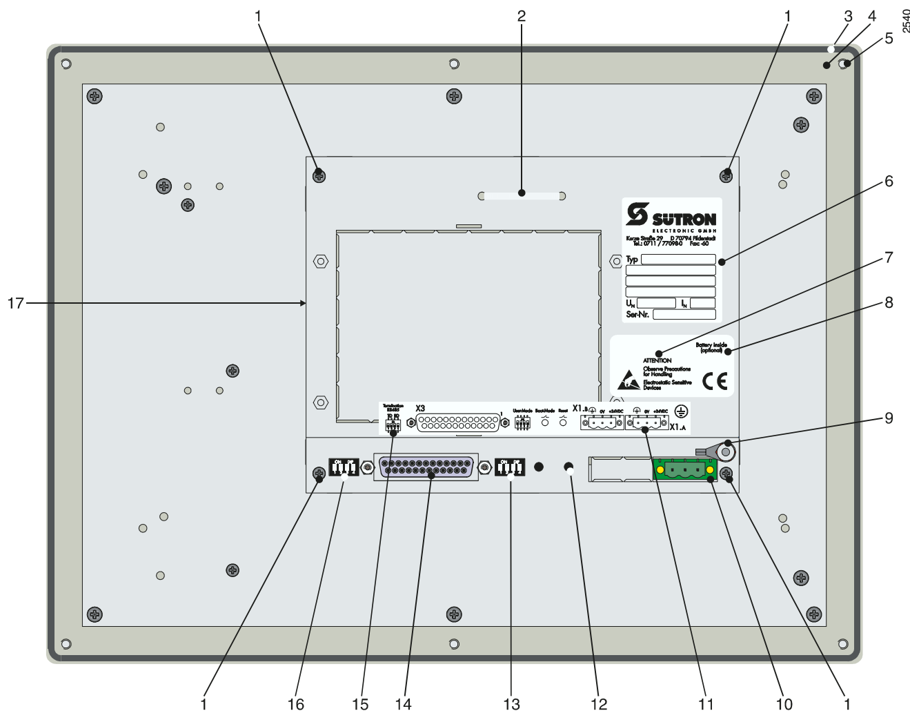
Figure 4-1 Rear view standard device
