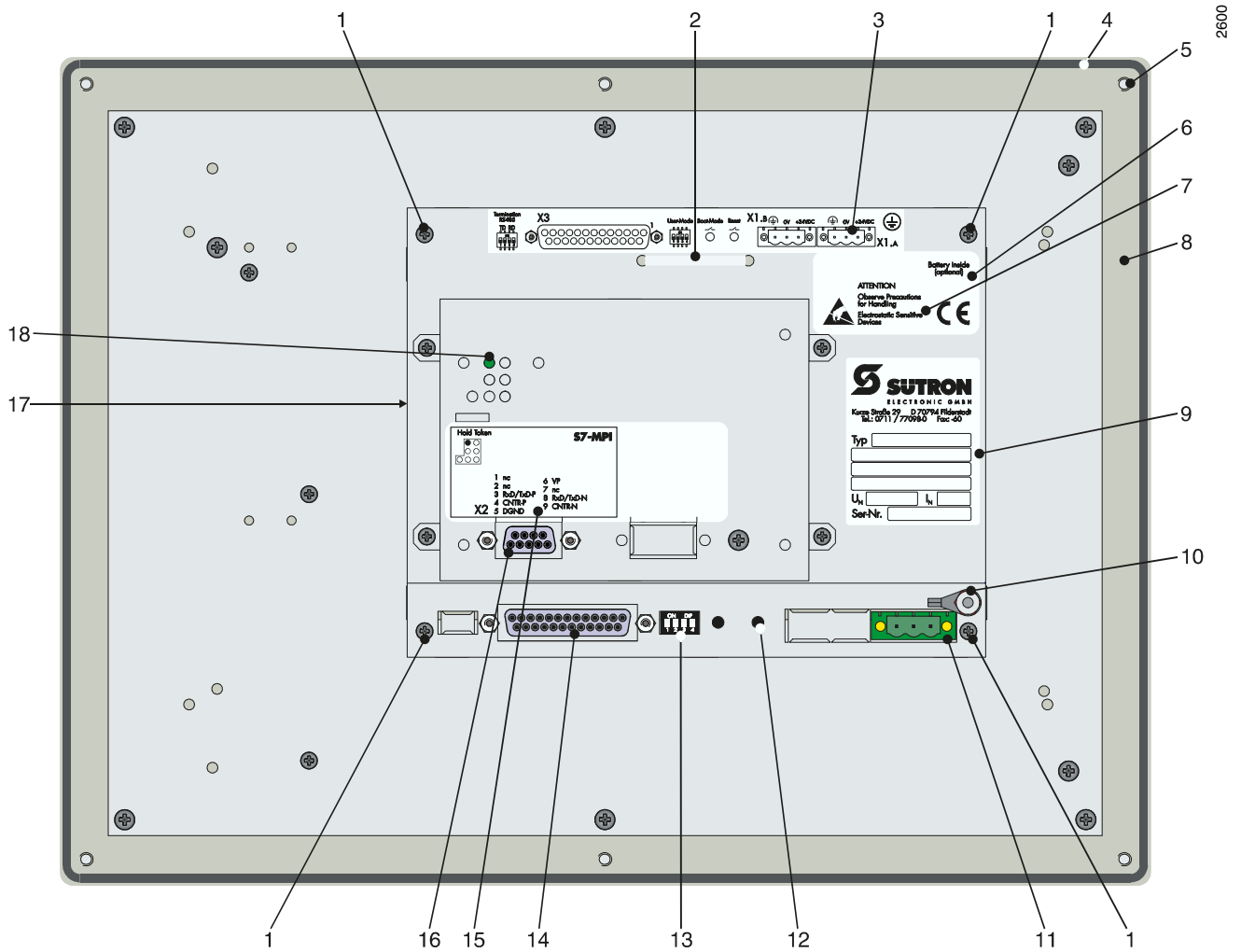
Figure 4-9 Rear view MPI
