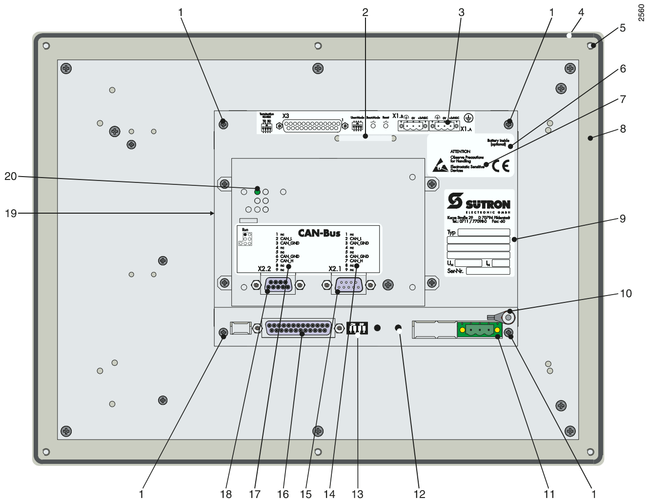
Figure 4-2 Rear view CAN bus
