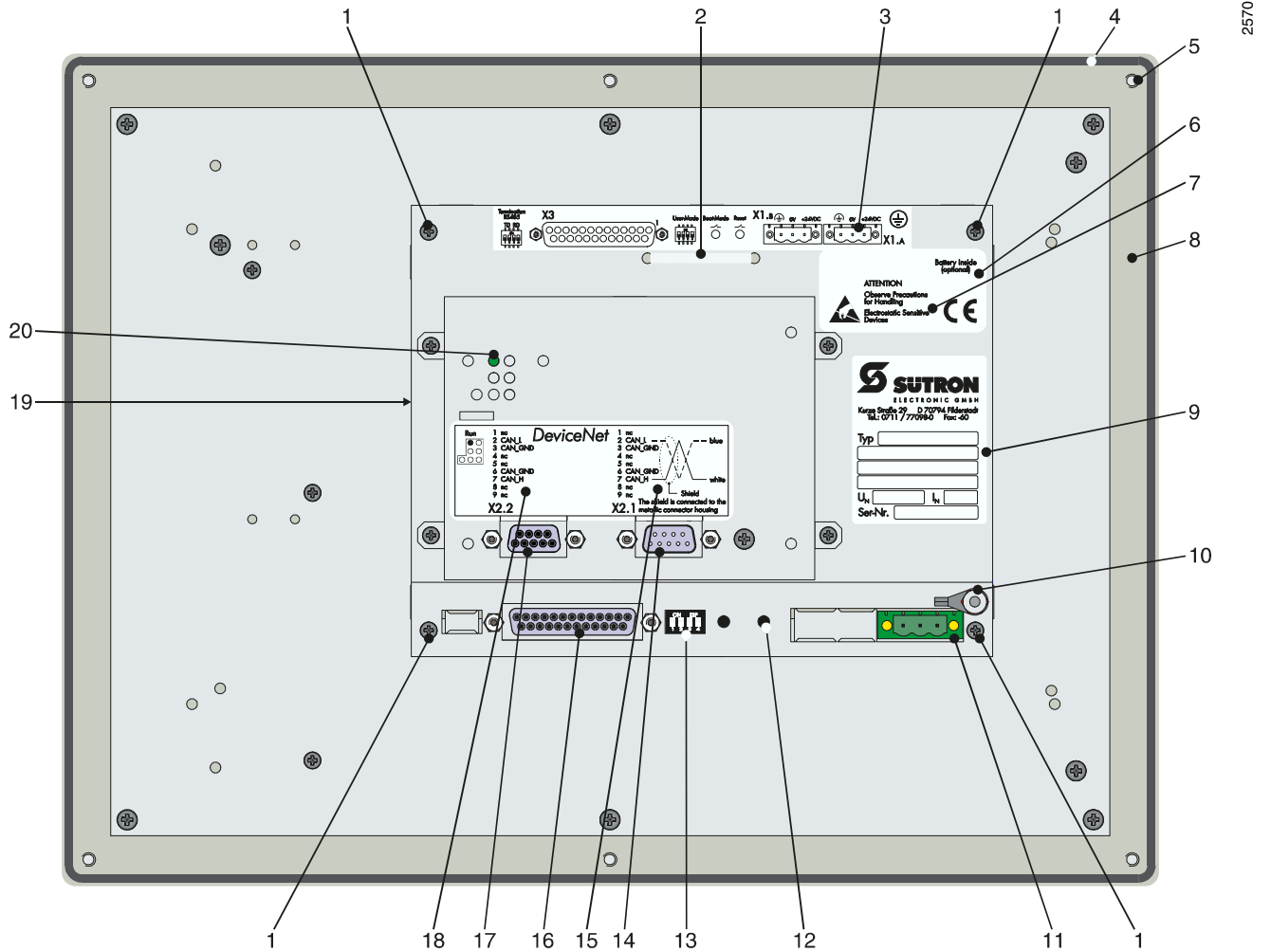
Figure 4-4 Rear view DeviceNet
