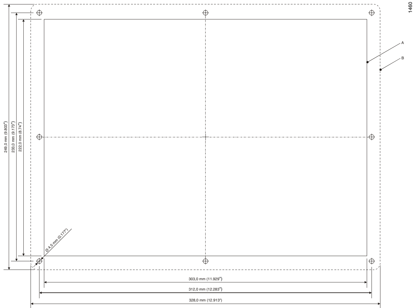
Figure 2-2 Mounting cutout
