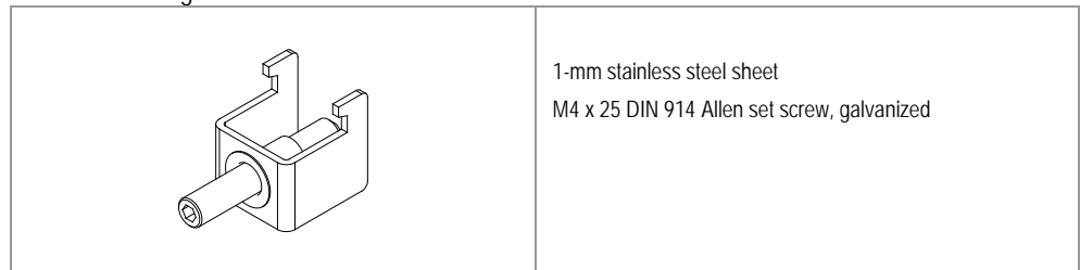
Abb. 5 Device holding bracket
