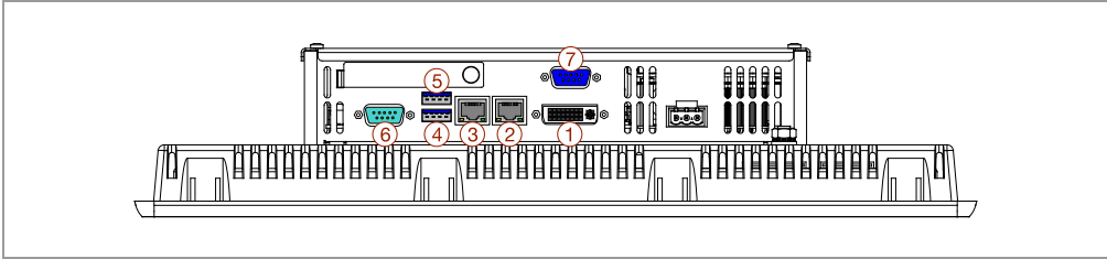
Abb. 10 Connections for peripherals
