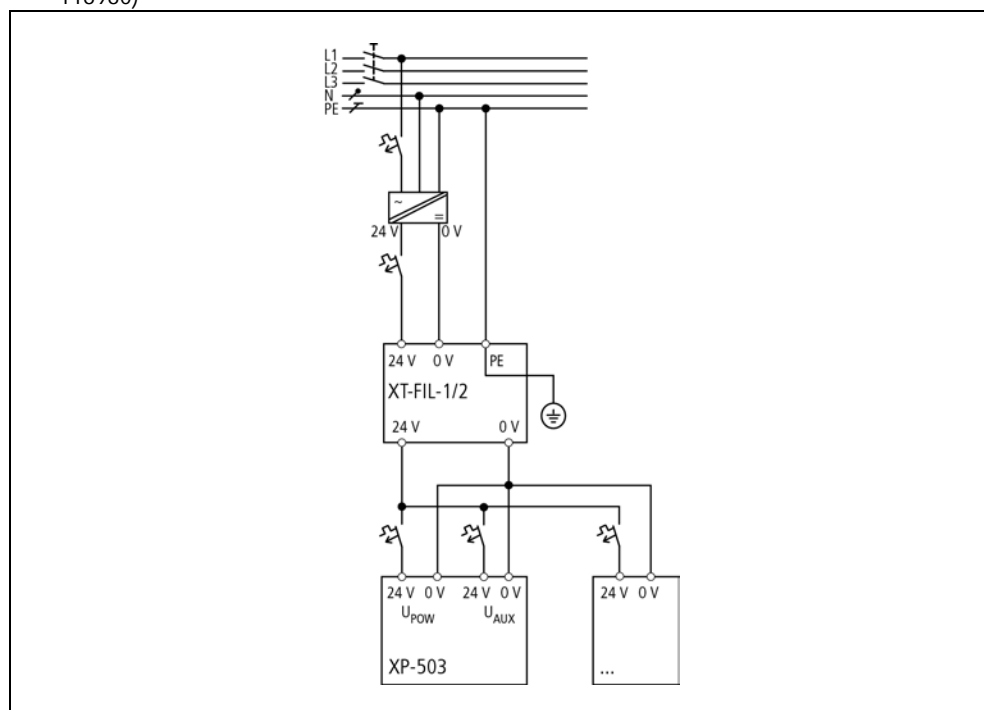
Abb. 6 Power supply with EMC filter
