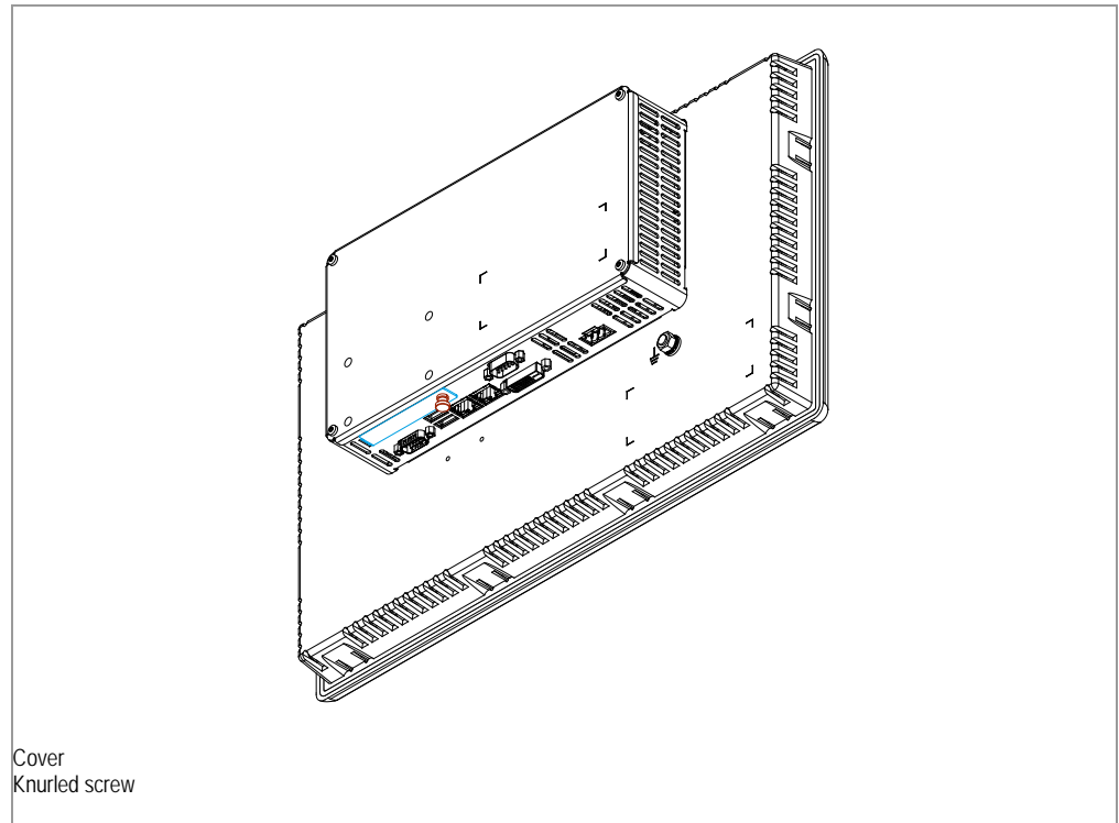
Abb. 11 CFast memory card location
