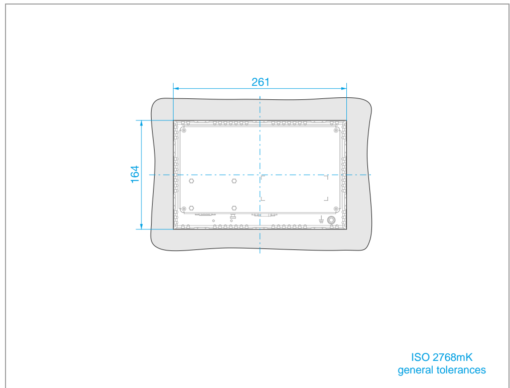
Abb. 15 XP-503-10 – fitting dimensions
