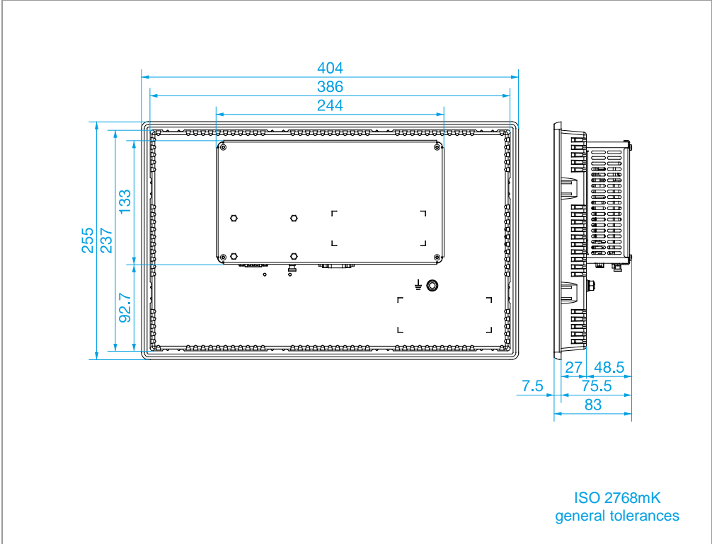
Abb. 17 XP-503-15 – device dimensions
