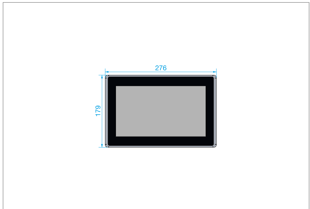
Abb. 13 XP-503-10 – front dimensions
