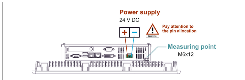
Abb. 7 Connecting the 24 V DC supply voltage
