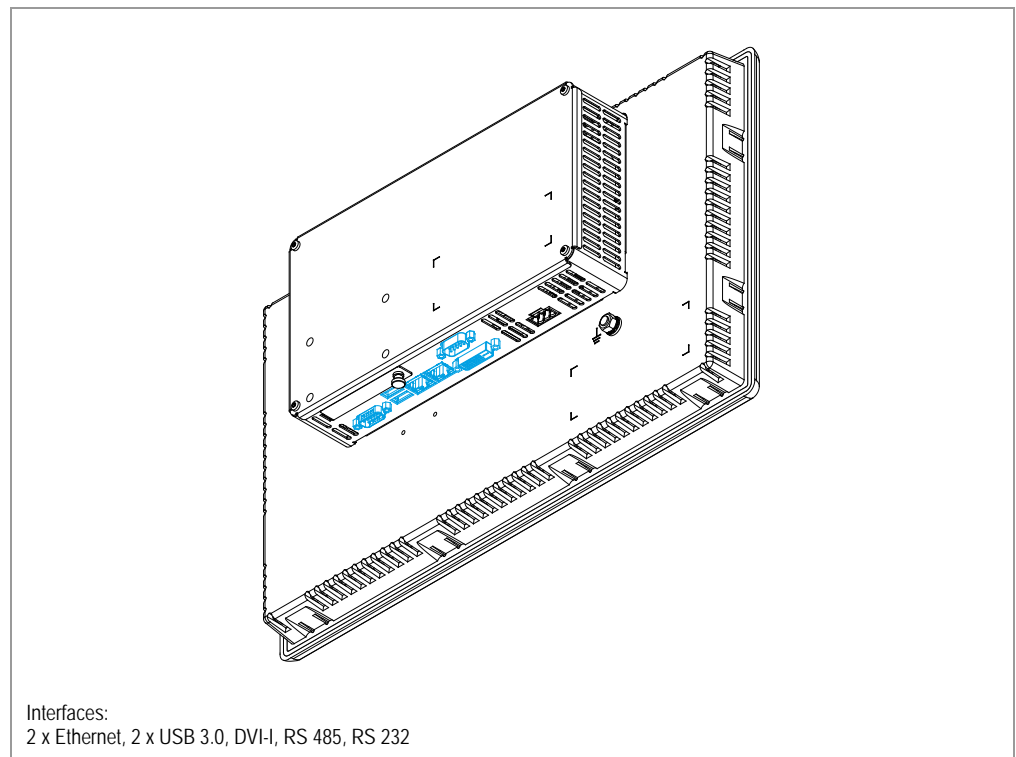
Abb. 9 Connection locations
