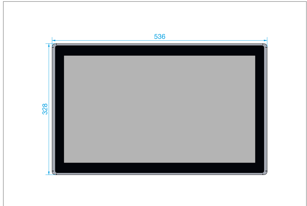
Abb. 19 XP-503-21 – front dimensions
