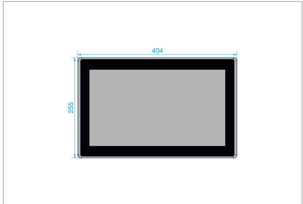
Abb. 16 XP-503-15 – front dimensions
