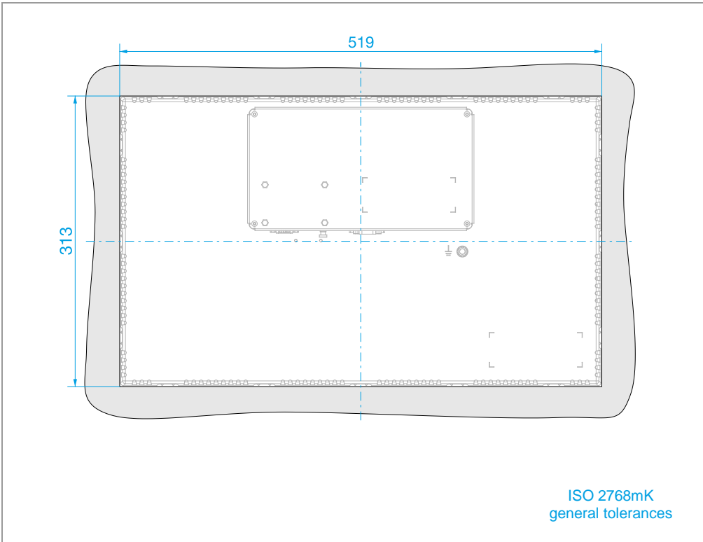
Abb. 21 XP-503-21 – fitting dimensions
