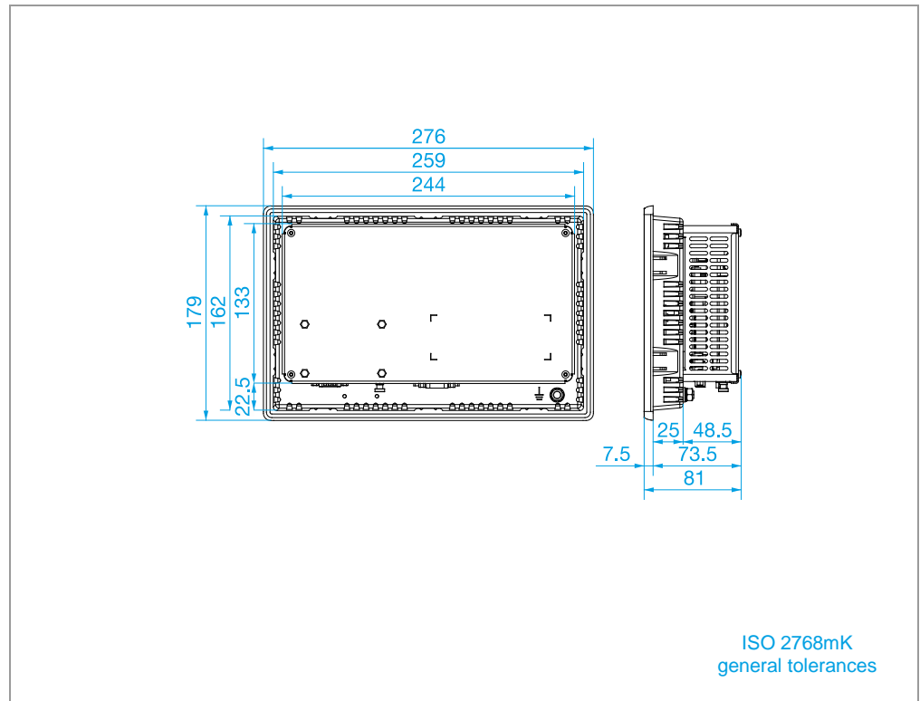
Abb. 14 XP-503-10 – device dimensions
