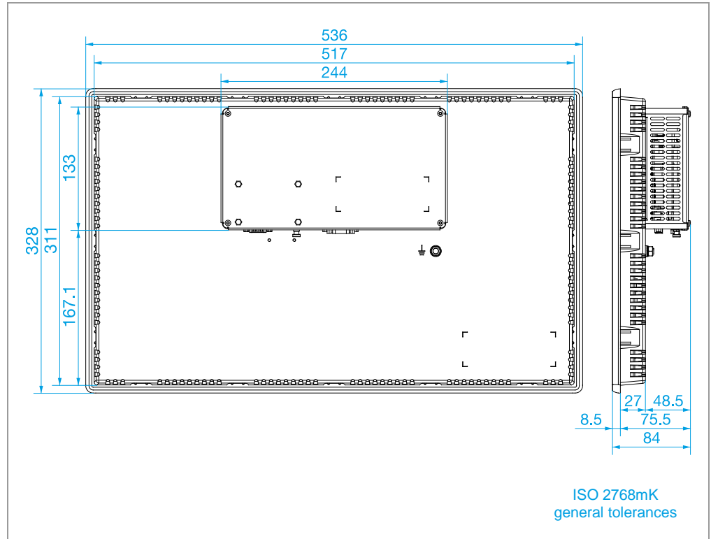
Abb. 20 XP-503-21 – device dimensions
