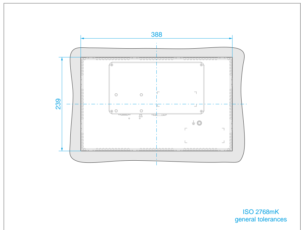
Abb. 18 XP-503-15 – fitting dimensions
