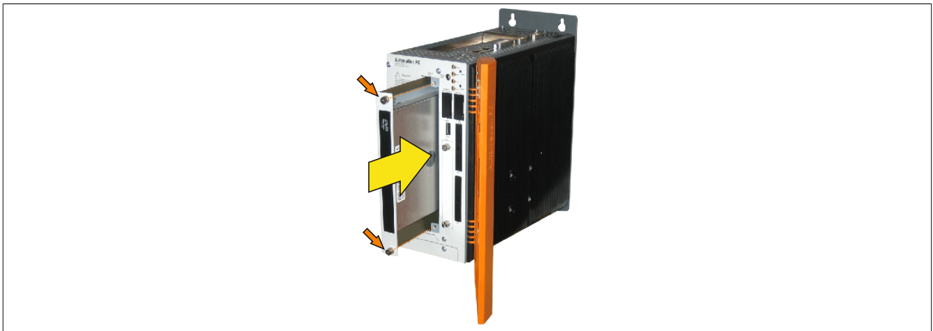
Figure 237: Installing the slide-in drive
