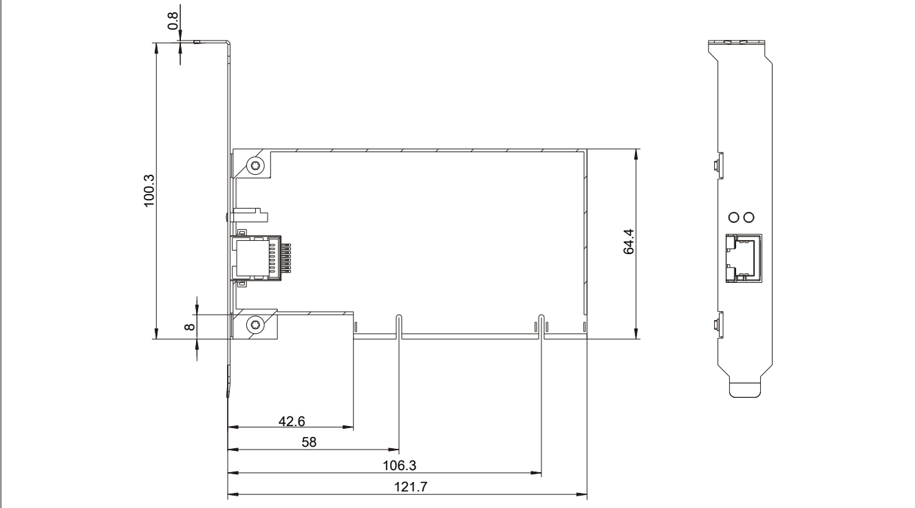
Figure 207: 5ACPCI.ETH1-01 - Dimensions
