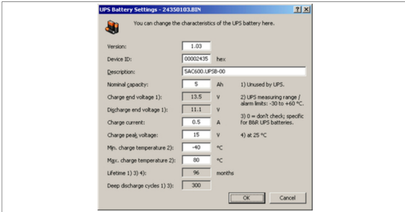
Figure 166: ADI Control Center - UPS battery settings
