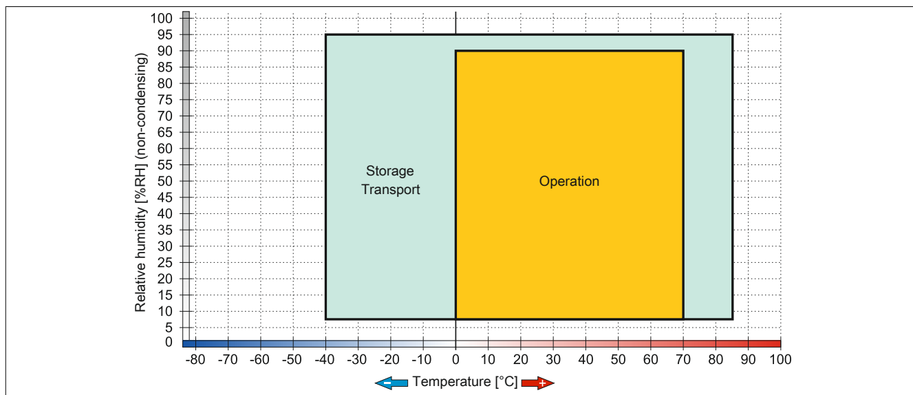
Figure 55: 5MMSSD.0060-01 ≤ Rev. C0 - Temperature/Humidity diagram
