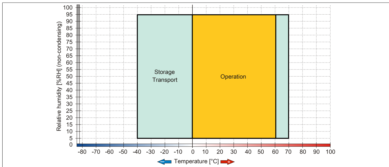
Figure 75: 5MMHDD.0500-00 - Temperature humidity diagram
