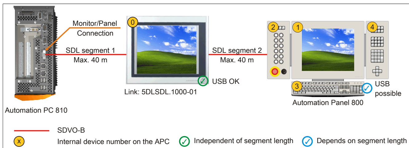
Figure 99: One AP900 system and one AP800 system via onboard SDL
