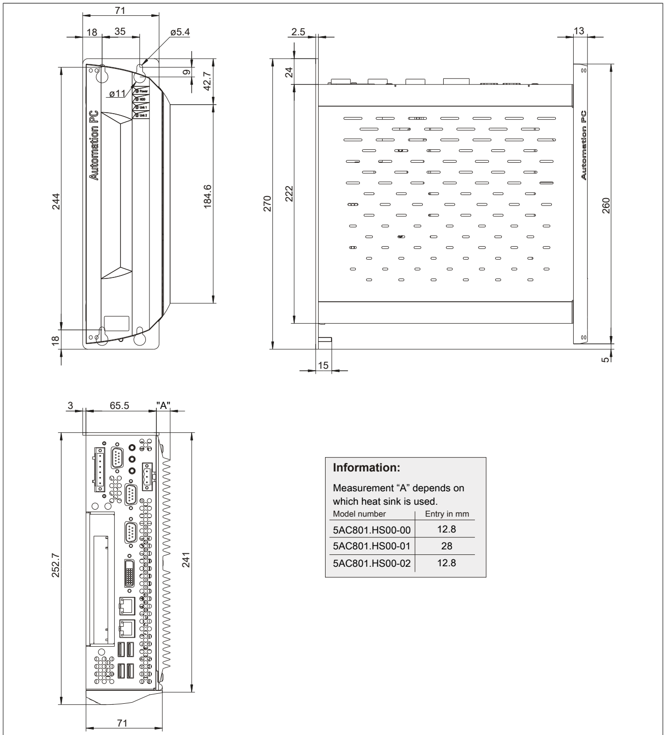
Figure 21: 5PC810.SX01-00 - Dimensions
