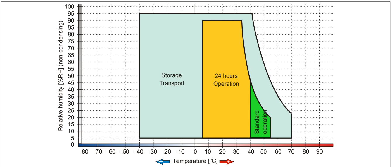
Figure 65: 5ACPCI.RAIC-01 - Temperature humidity diagram
