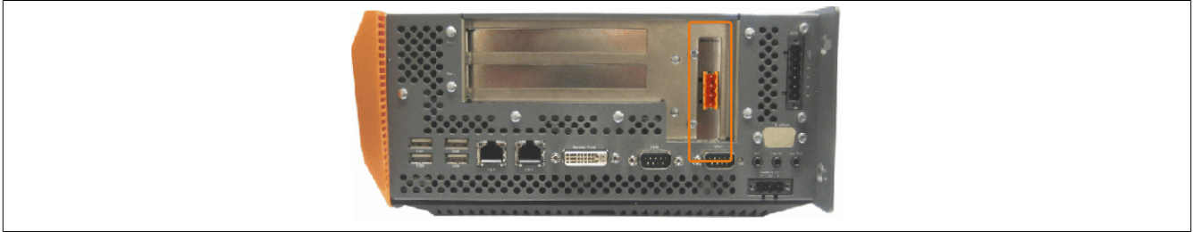
Figure 81: Installation example with the 5PC810.SX02-00 system unit
