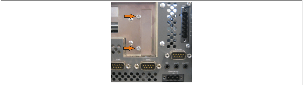
Figure 286: Removing the AP Link module cover
