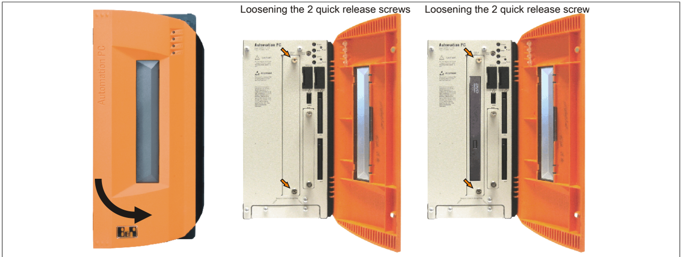
Figure 238: Loosening the quick release screws
