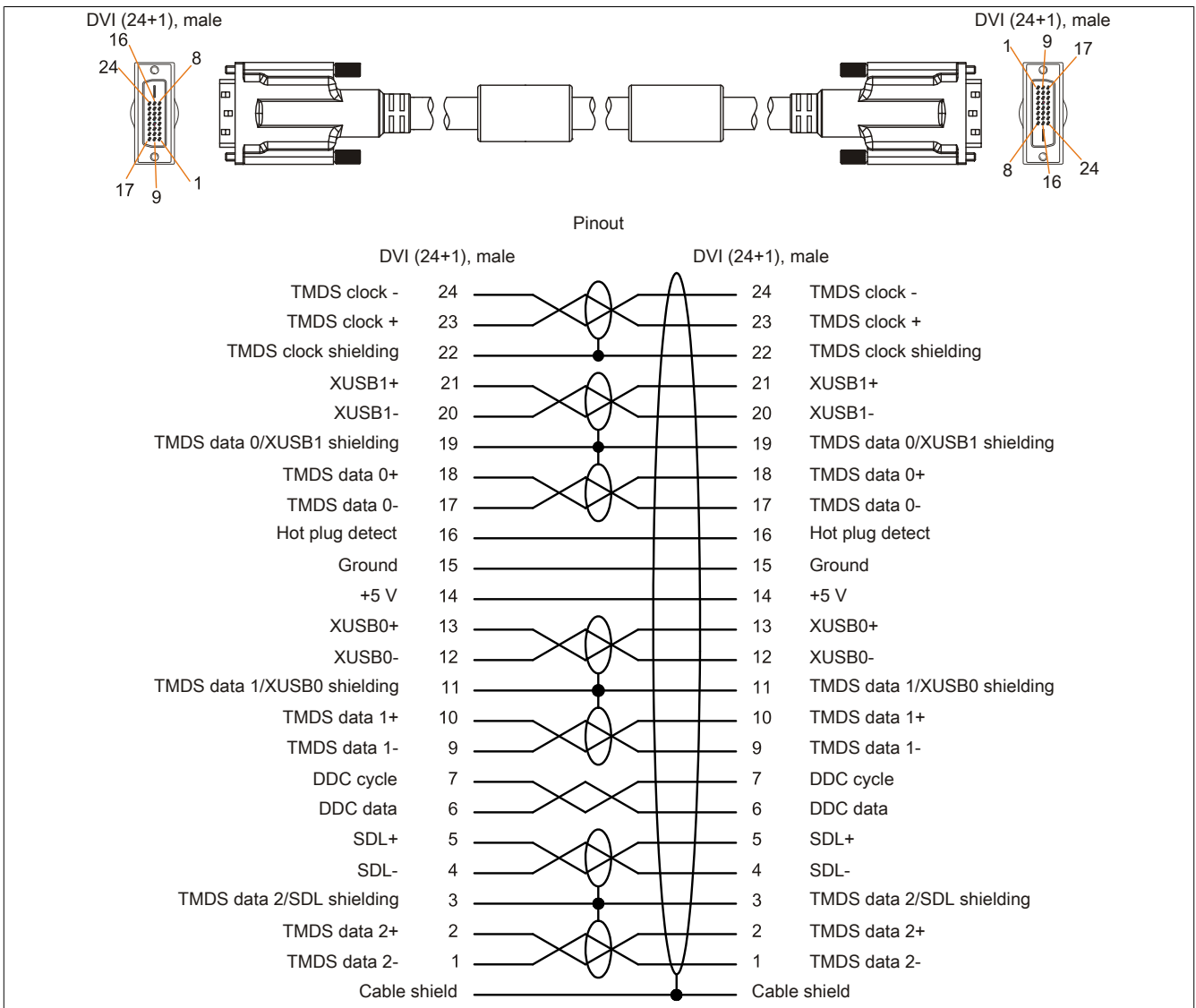
Figure 221: 5CASDL.0xxx-03 - Pinout
