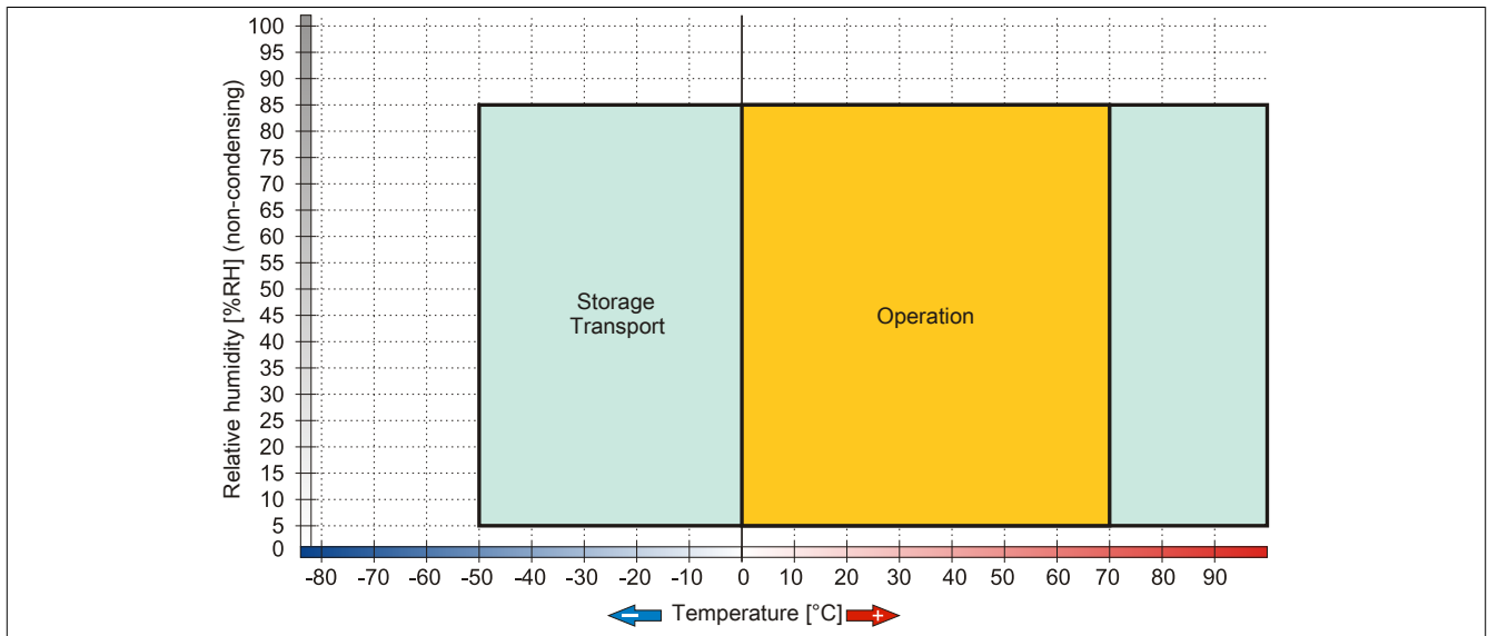
Figure 197: 5MMUSB.xxxx-01 - Temperature/Humidity diagram
