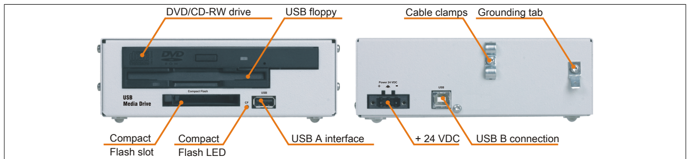
Figure 183: 5MD900.USB2-01 - Interfaces
