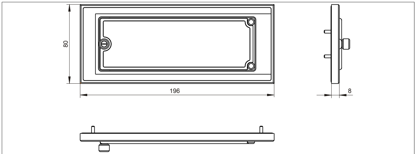
Figure 193: 5A5003.03 - Dimensions
