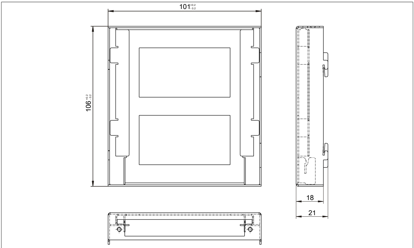
Figure 229: 5AC801.FRAM-00 - Dimensions
