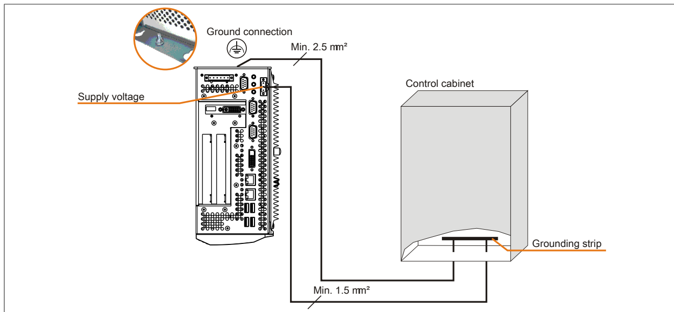
Figure 93: Grounding concept
