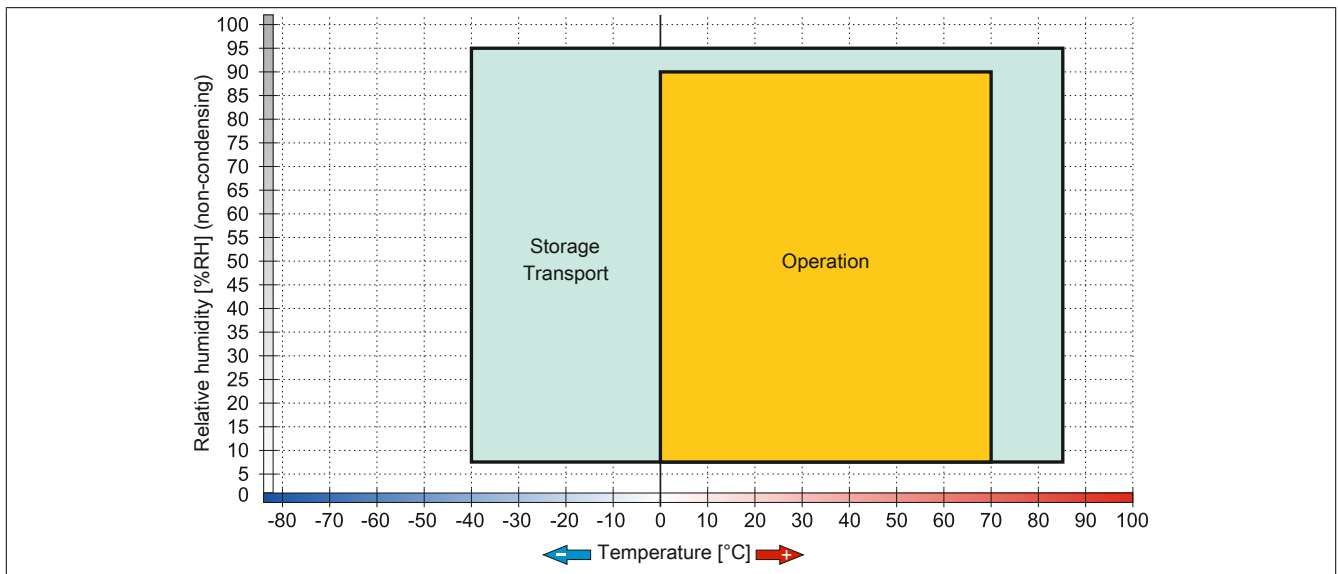
Figure 57: 5MMSSD.0128-01 ≤ Rev. C0 - Temperature/Humidity diagram
