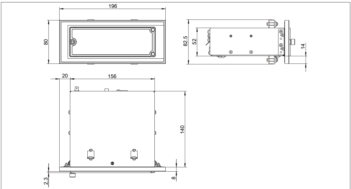
Figure 190: USB media drive with front cover - Dimensions
