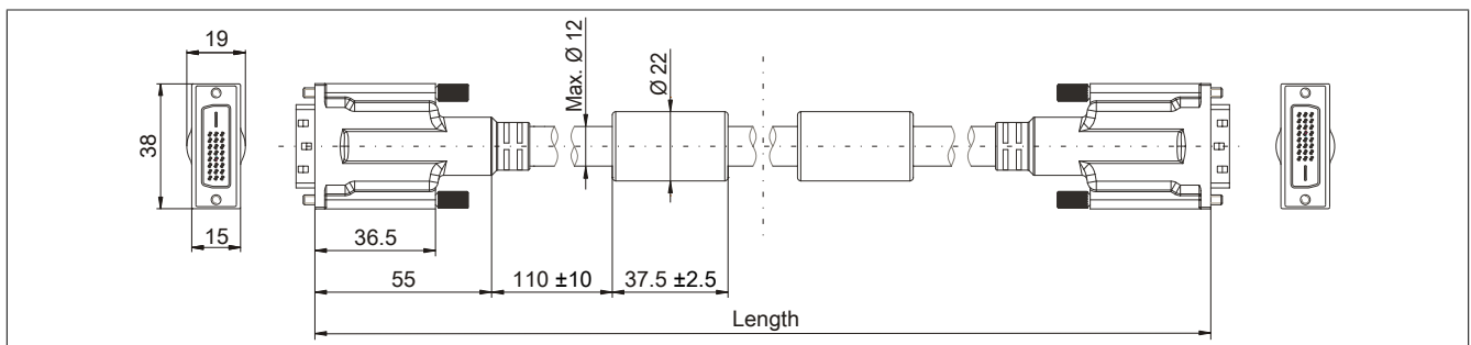
Figure 220: 5CASDL.0xxx-03 - Dimensions
