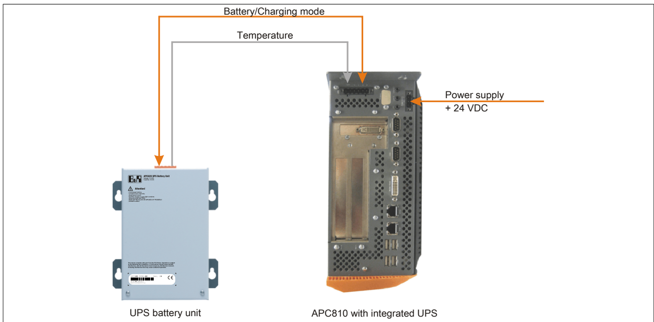
Figure 198: UPS principle
