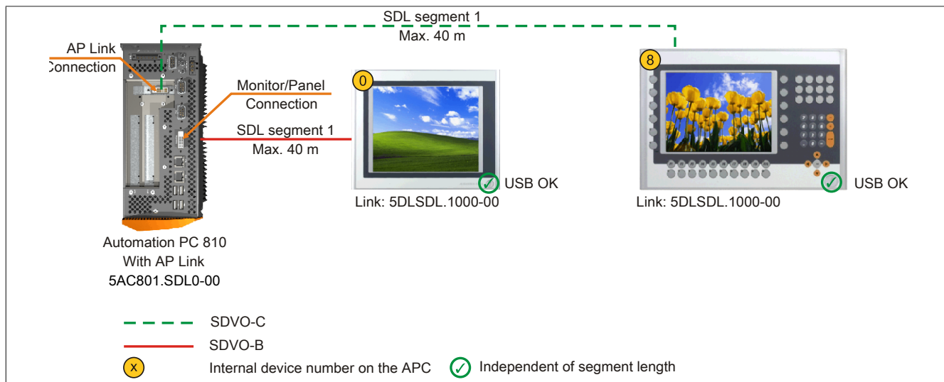
Figure 103: Two Automation Panel 900 systems via onboard SDL and SDL AP Link
