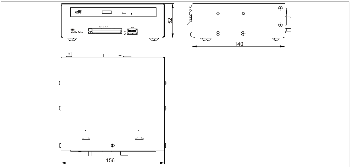
Figure 189: 5MD900.USB2-02 - Dimensions
