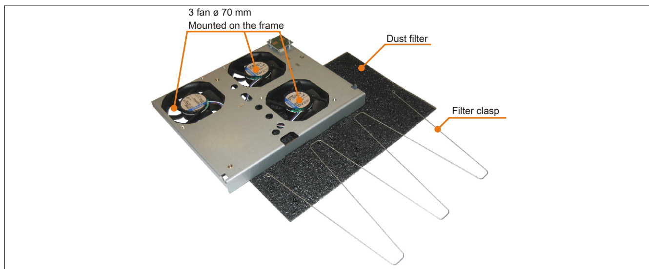
Figure 79: 5PC810.FA05-00 - Fan kit
