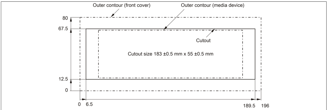
Figure 191: USB media drive with front cover - Installation cutout
