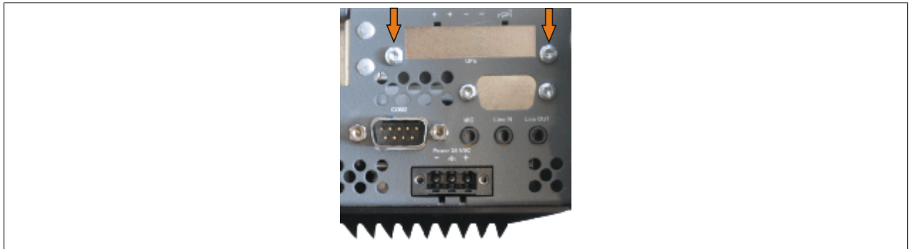
Figure 245: Removing the UPS module cover
