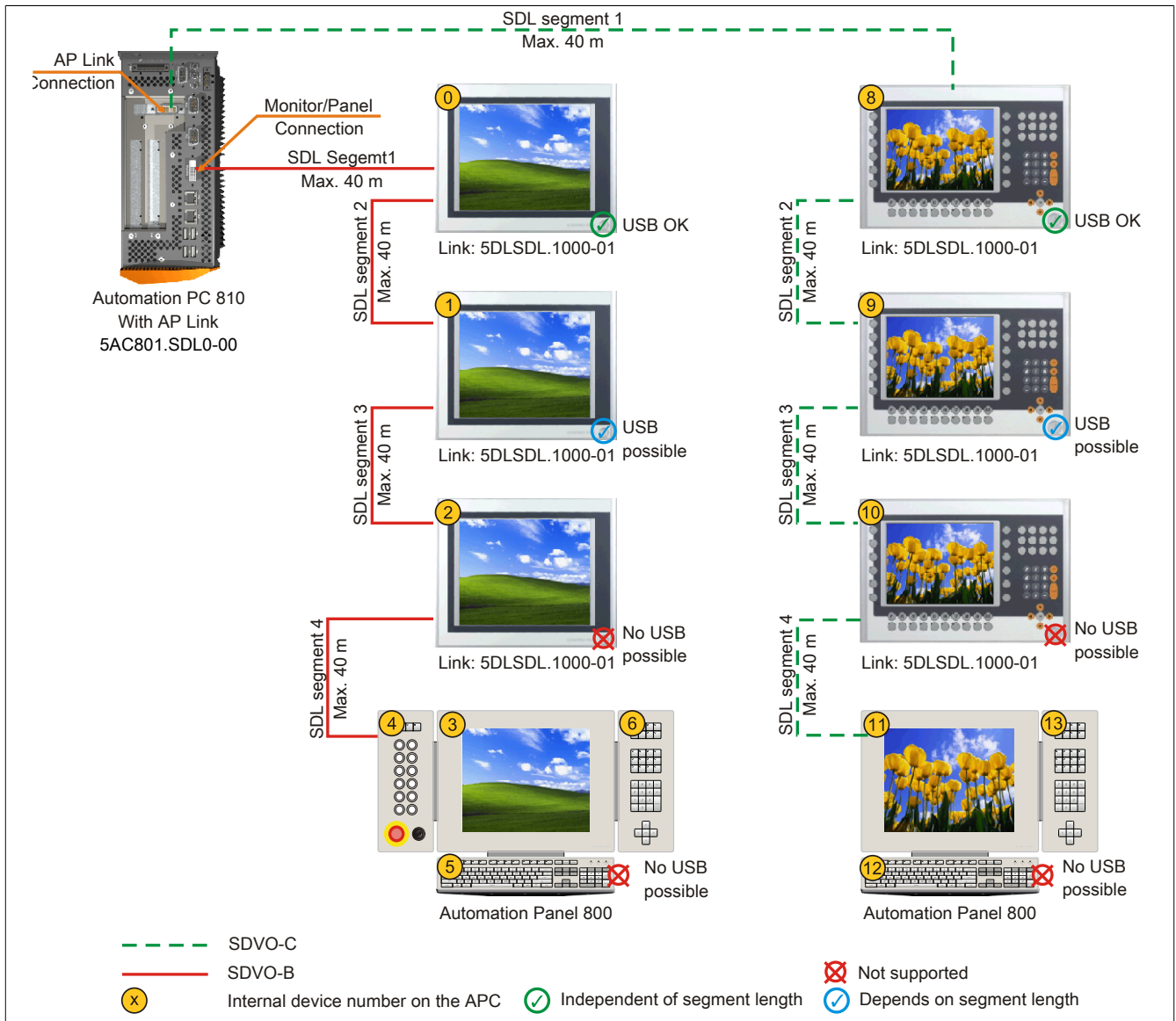
Figure 105: Six AP900 and two AP800 systems via onboard SDL and SDL AP Link
