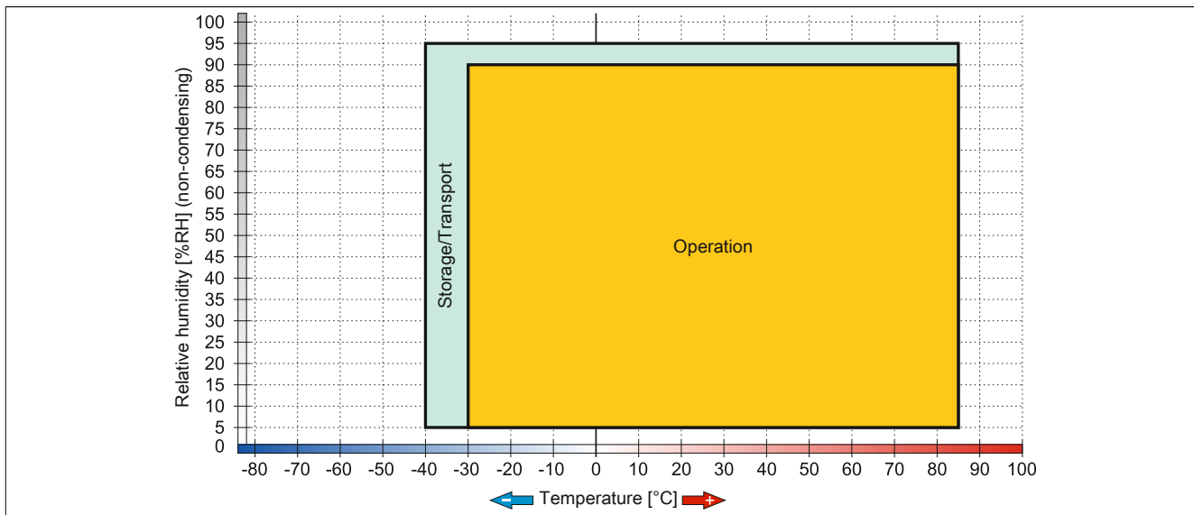
Figure 52: 5AC801.SSDI-04 ≥ Rev. D0 - Temperature/Humidity diagram
