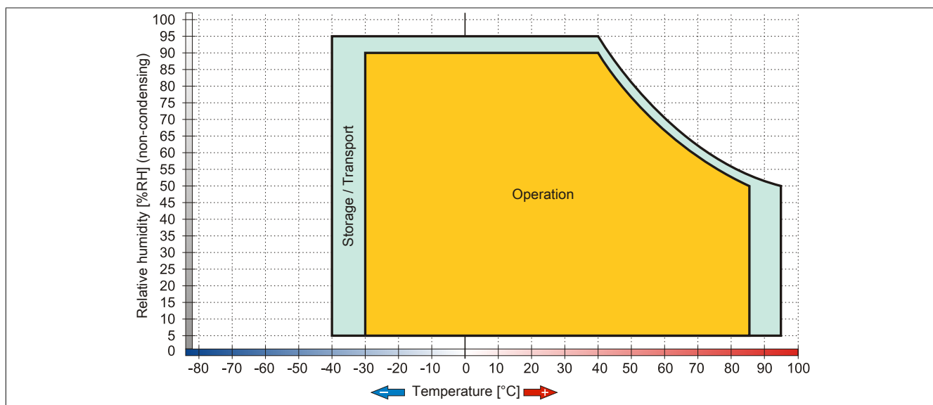
Figure 69: 5ACPCI.RAIC-04 - Temperature humidity diagram
