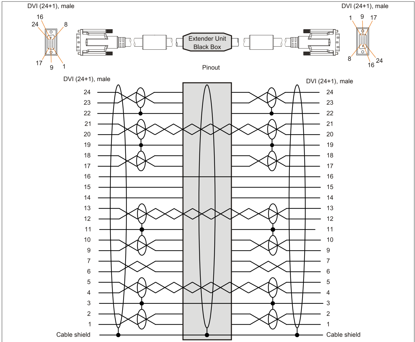
Figure 224: 5CASDL.0xx0-13 - Pinout
