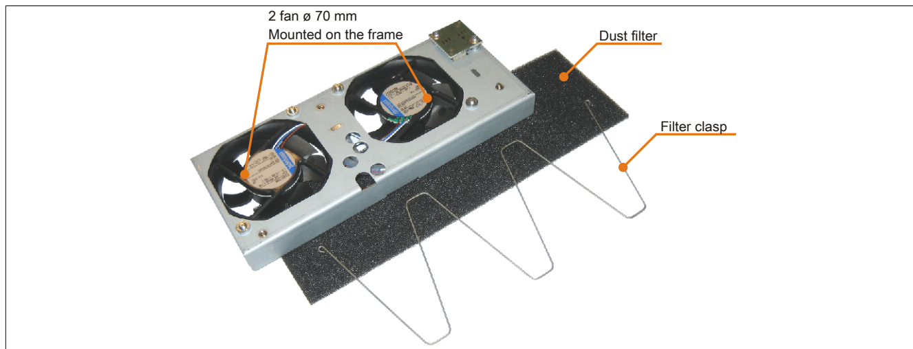
Figure 77: 5PC810.FA02-00 and 5PC810.FA02-01 - Fan kit
