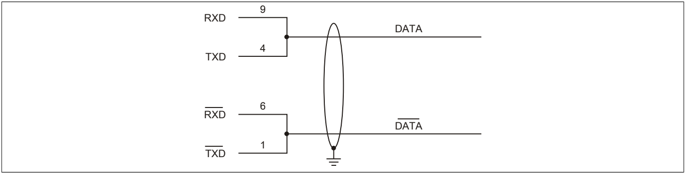
Figure 86: Add-on RS232/422/485 interface - Operated in RS485 mode
