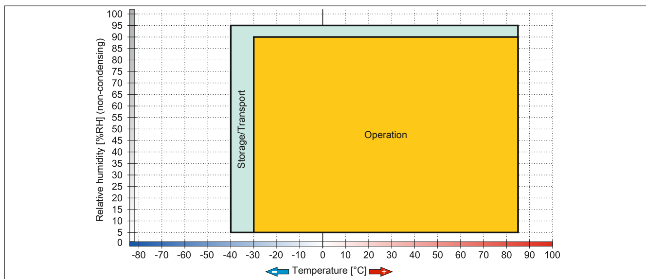
Figure 53: 5AC801.SSDI-05 - Temperature humidity diagram
