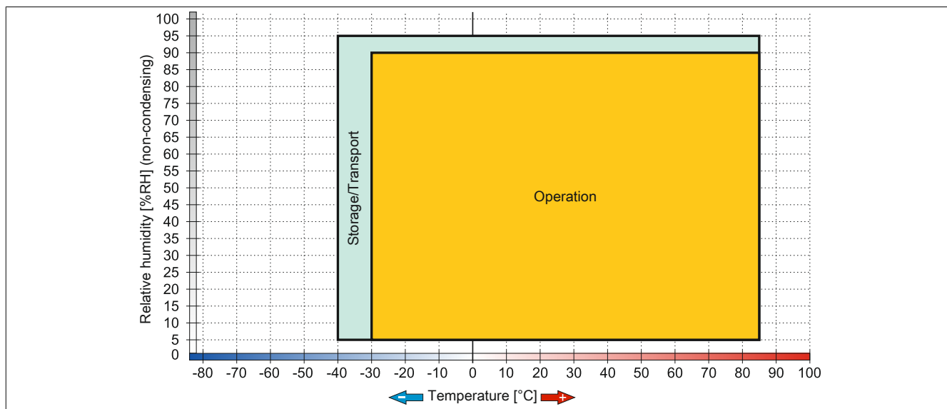
Figure 60: 5MMSSD.0256-00 - Temperature/Humidity diagram
