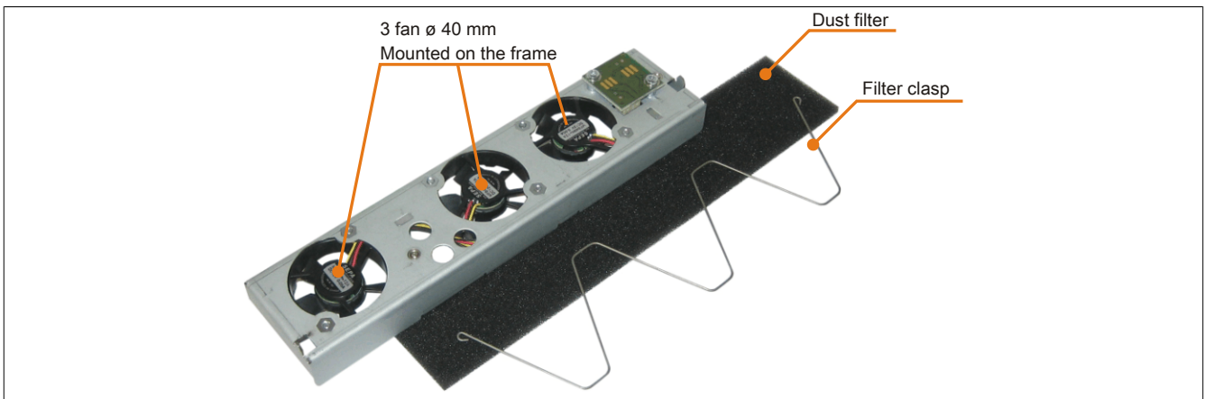
Figure 76: 5PC810.FA01-00 - Fan kit
