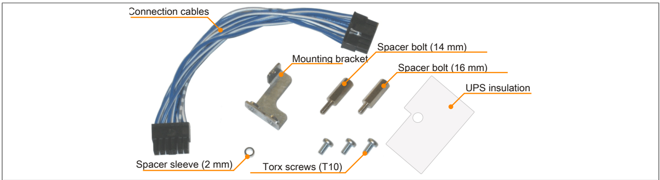
Figure 244: 5AC600. UPSI-00 Add-on UPS module - Installation materials
