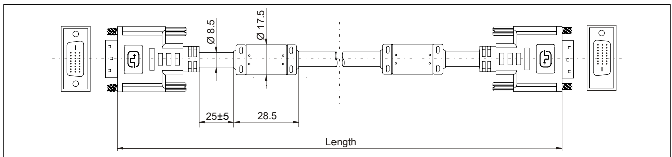
Figure 211: 5CADVI.0xxx-00 - Dimensions
