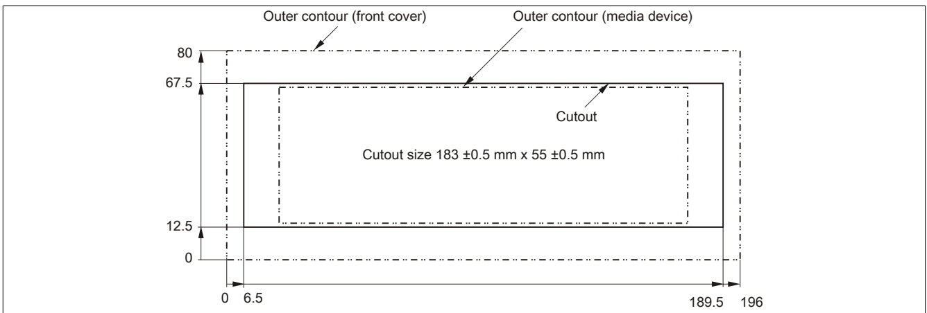
Figure 195: USB media drive with front cover - Installation cutout
