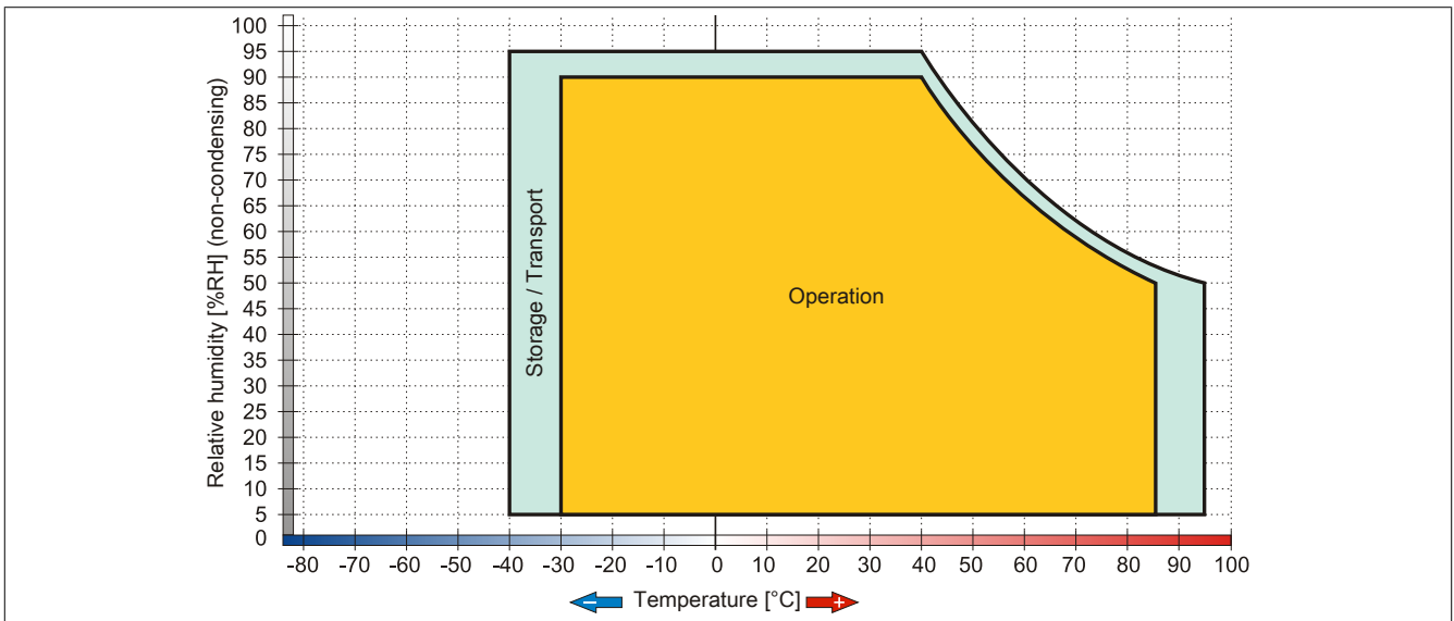
Figure 61: 5AC801.HDDS-00 - Temperature humidity diagram
