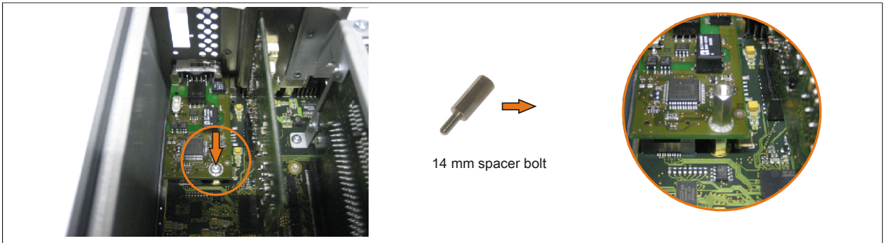
Figure 268: Screwing in the spacer bolt
