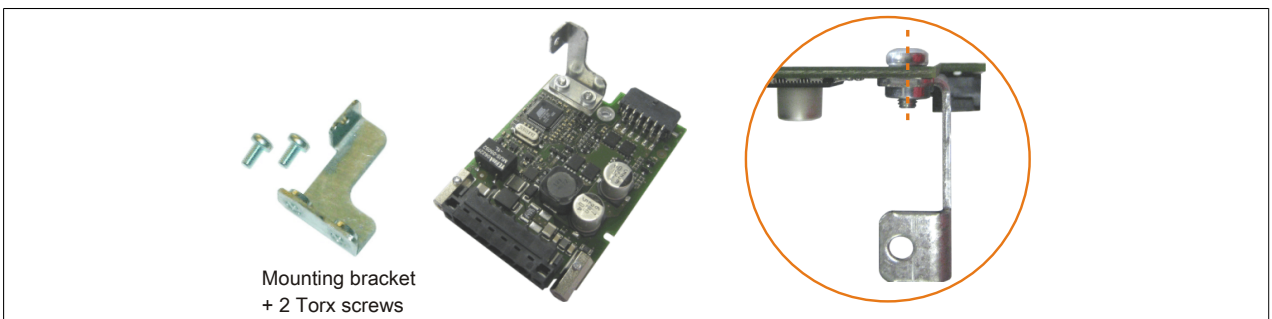
Figure 275: Installing the mounting bracket
