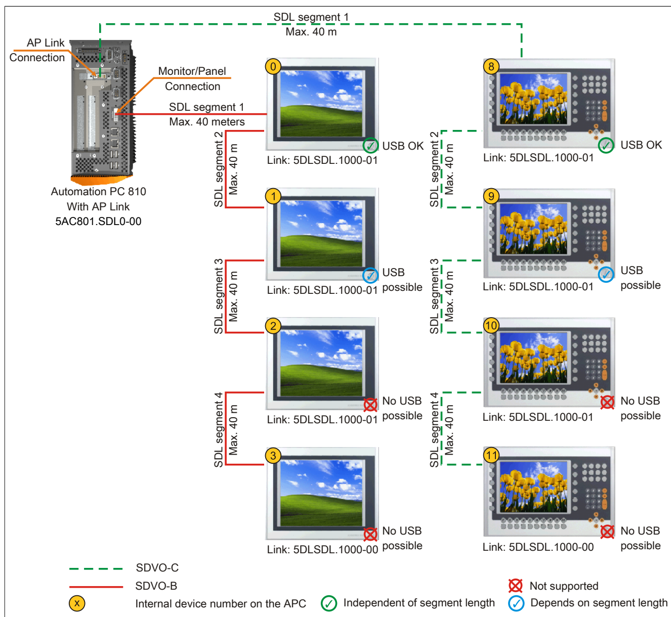
Figure 104: Eight Automation Panel 900 systems via onboard SDL and SDL AP Link
