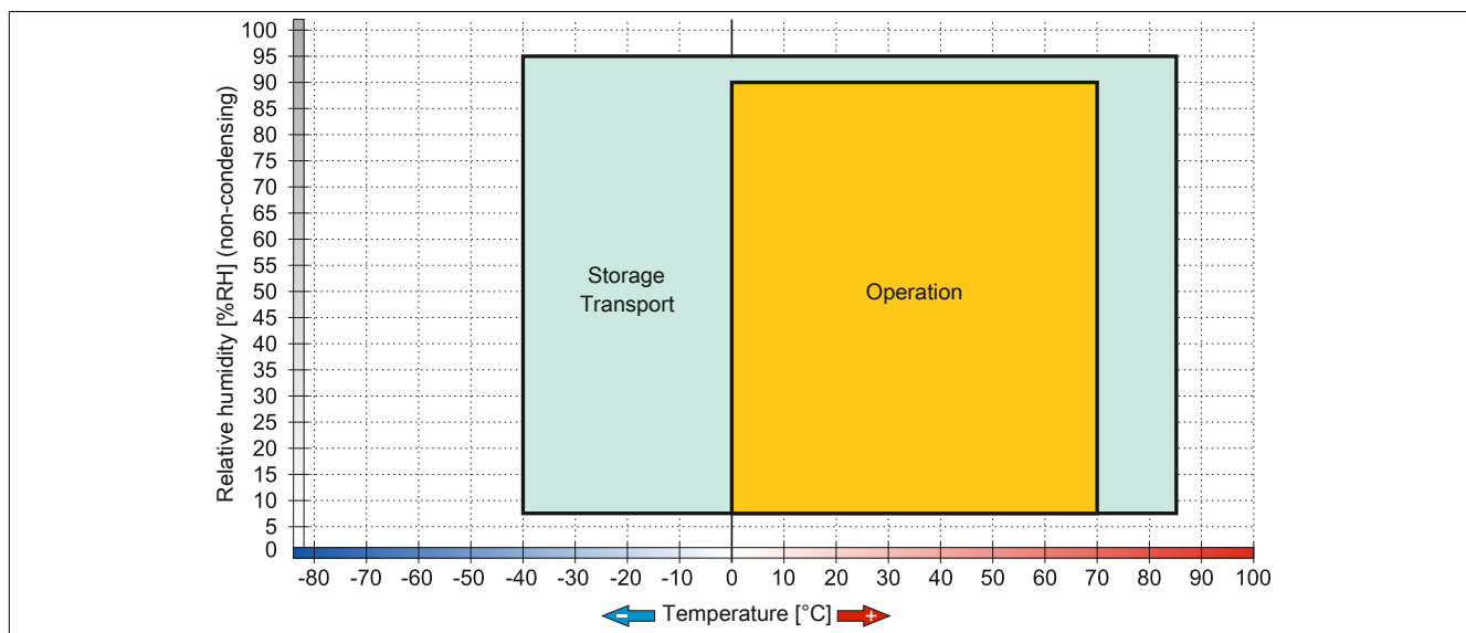
Figure 49: 5AC801.SSDI-03 ≤ Rev. C0 - Temperature/Humidity diagram
