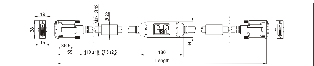
Figure 223: 5CASDL.0xx0-13 - Dimensions
