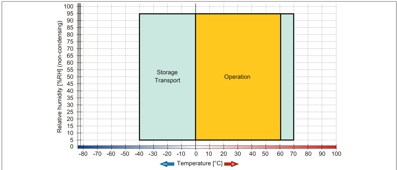
Figure 71: 5ACPCI.RAIC-05 - Temperature humidity diagram
