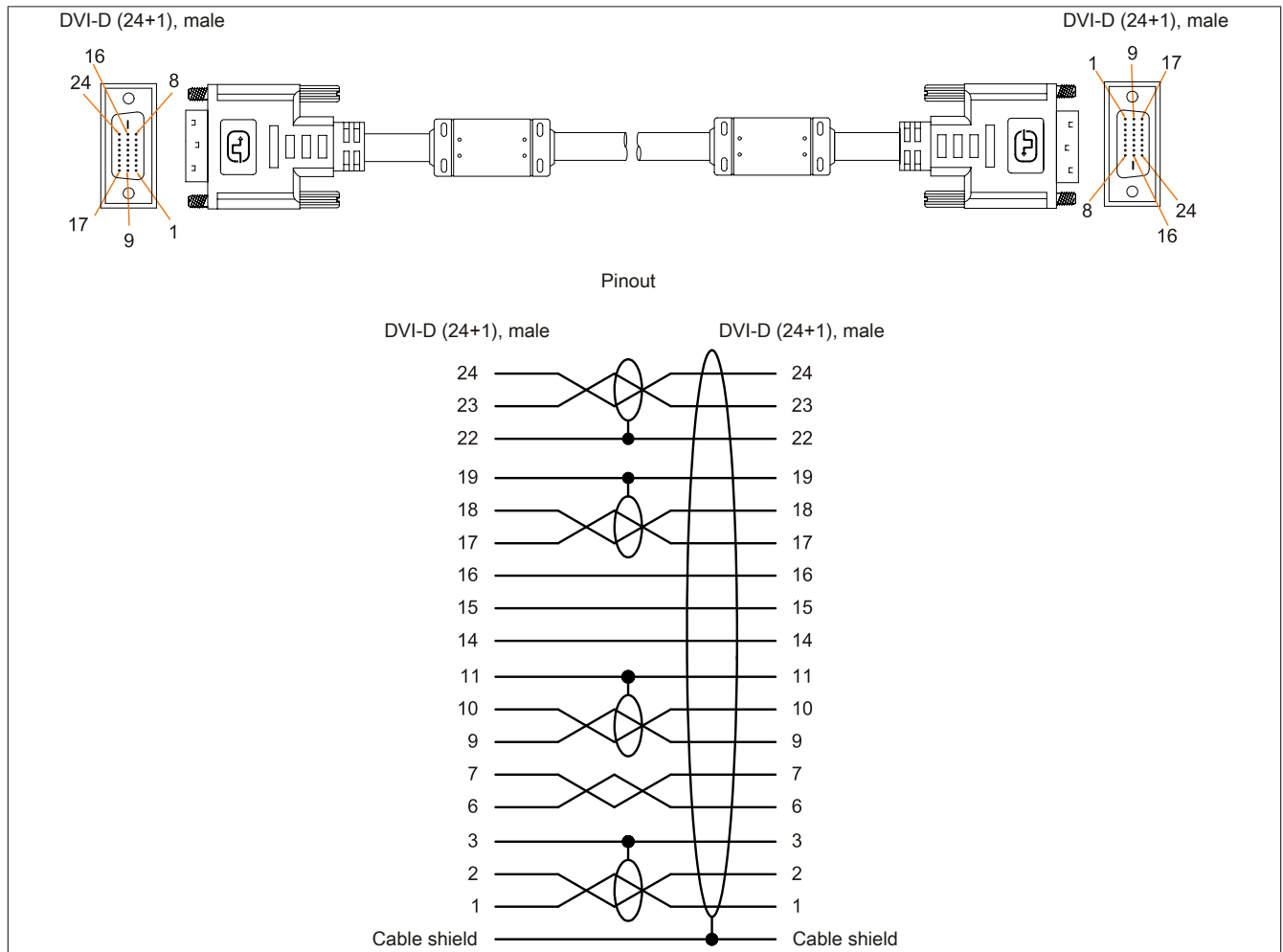
Figure 212: 5CADVI.0xxx-00 - Pinout
