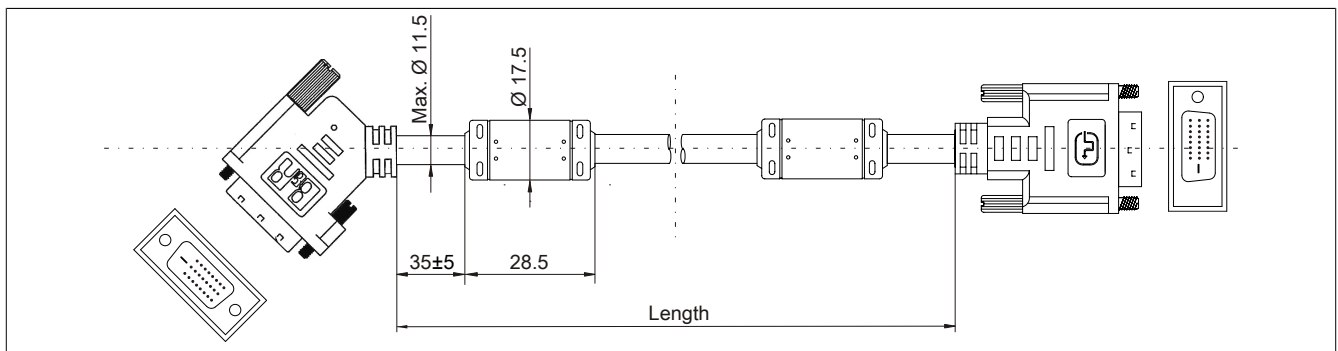
Figure 217: 5CASDL.0xxx-01 - Dimensions
