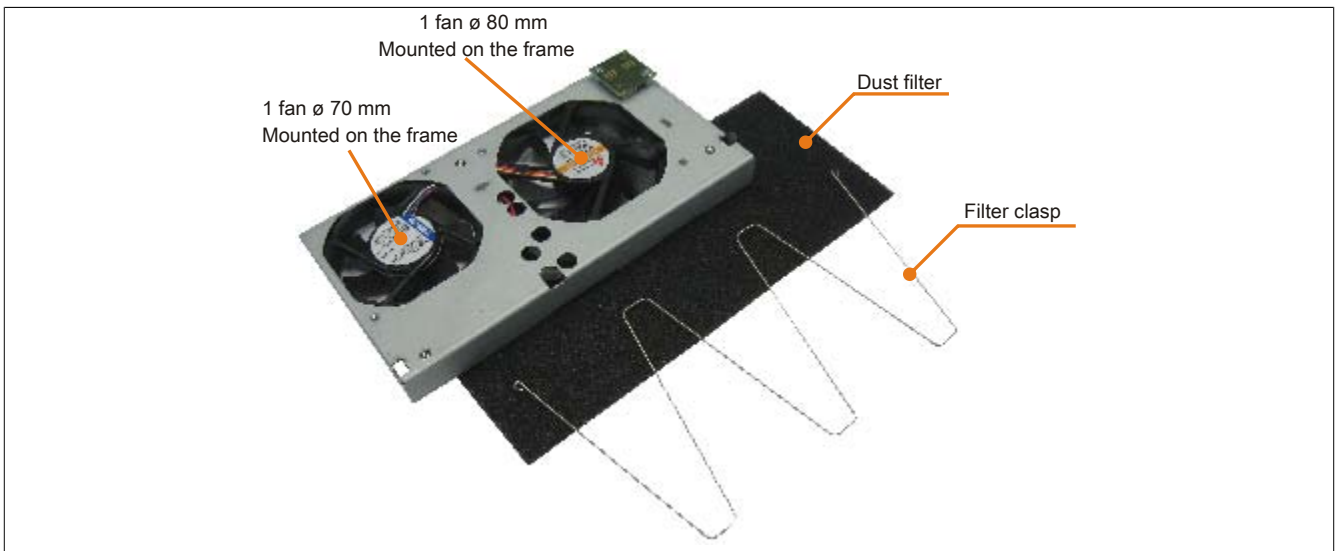
Figure 78: 5PC810.FA03-00 - Fan kit
