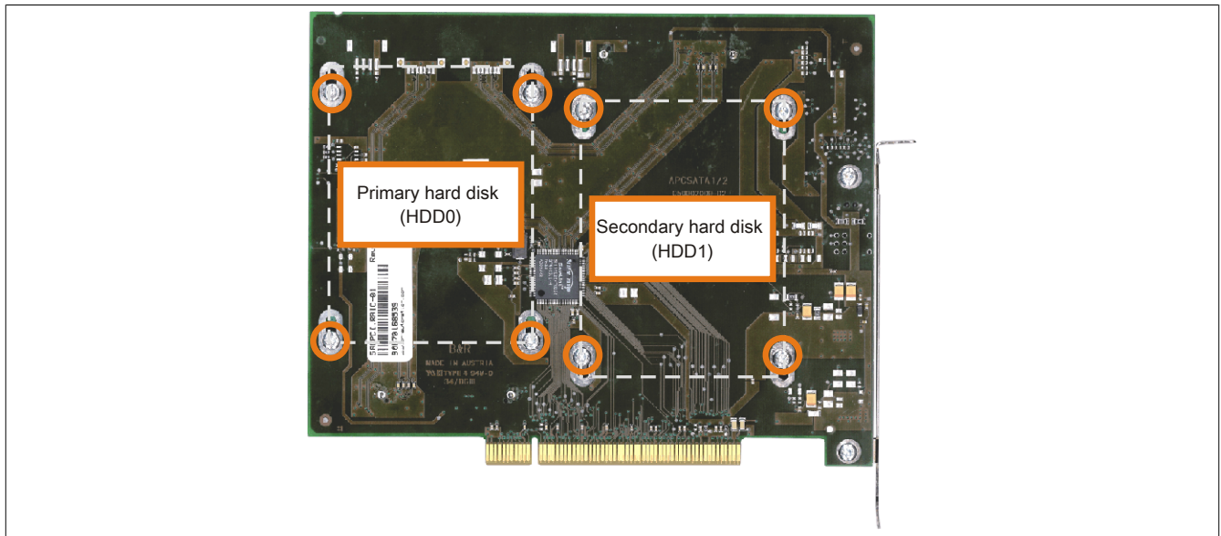
Figure 288: Screw layout on the back side of the 5ACPCI.RAIC-03 SATA RAID controller
