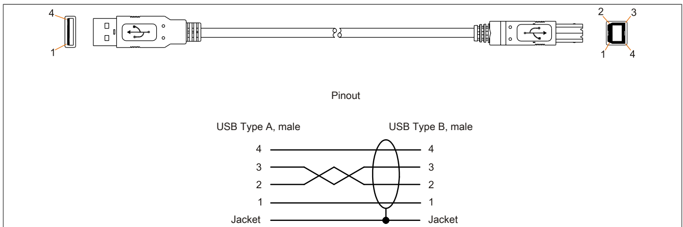
Figure 226: 5CAUSB.00xx-00 USB cables - Pinout
