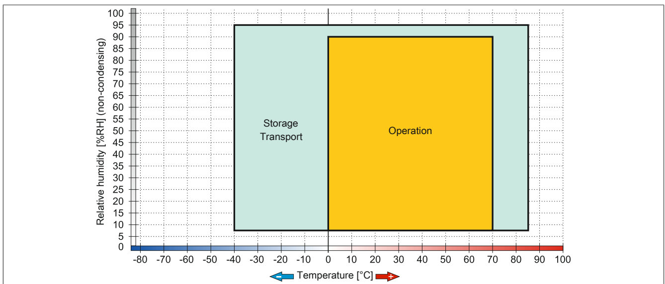
Figure 51: 5AC801.SSDI-04 ≤ Rev. C0 - Temperature/Humidity diagram
