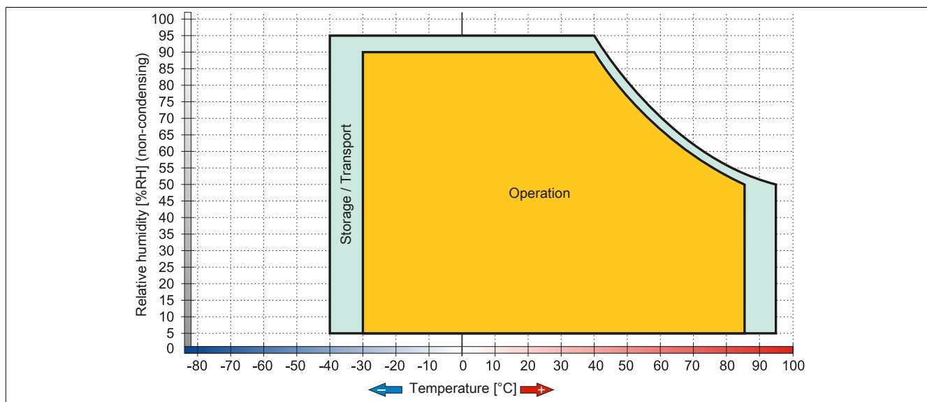
Figure 68: 5ACPCI.RAIC-03 - Temperature humidity diagram
