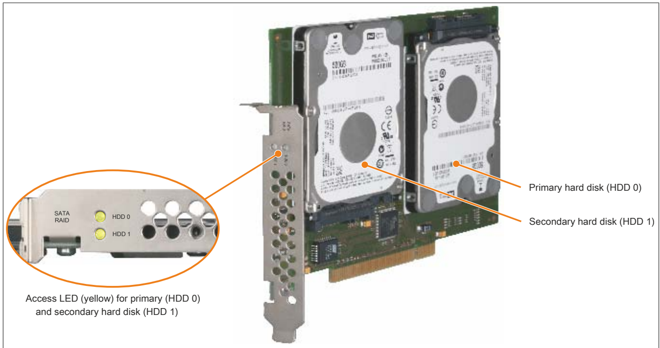
Figure 72: PCI SATA RAID controller
