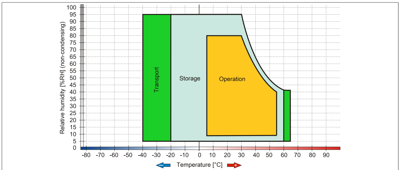
Figure 62: 5AC801.DVDS-00 - Temperature humidity diagram
