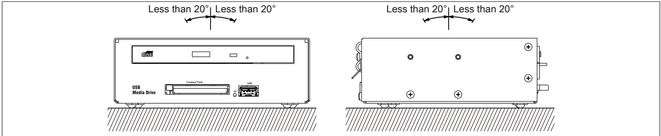
Figure 192: 5MD900.USB2-02 - Mounting orientation
