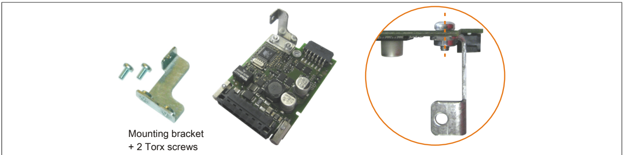
Figure 269: Installing the mounting bracket
