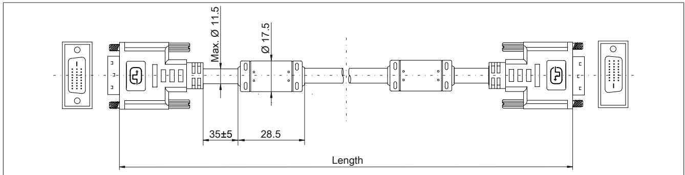
Figure 214: 5CASDL.0xxx-00- Dimensions
