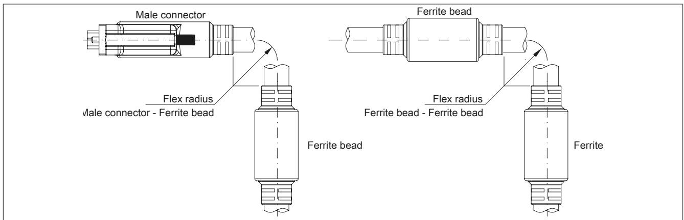
Figure 219: Flex radius specifications
