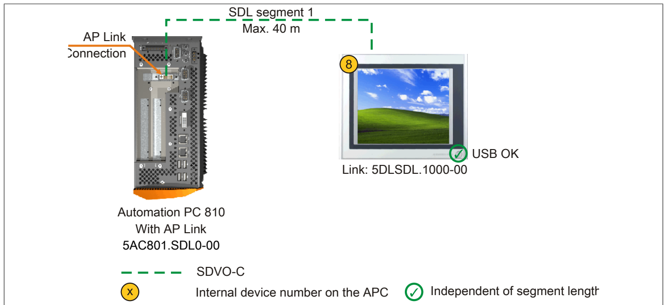
Figure 101: One Automation Panel 900 system via SDL AP Link
