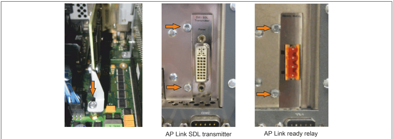
Figure 287: Installing the AP Link module
