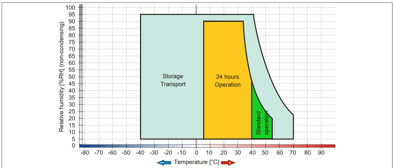
Figure 66: 5ACPCI.RAIC-02 - Temperature humidity diagram
