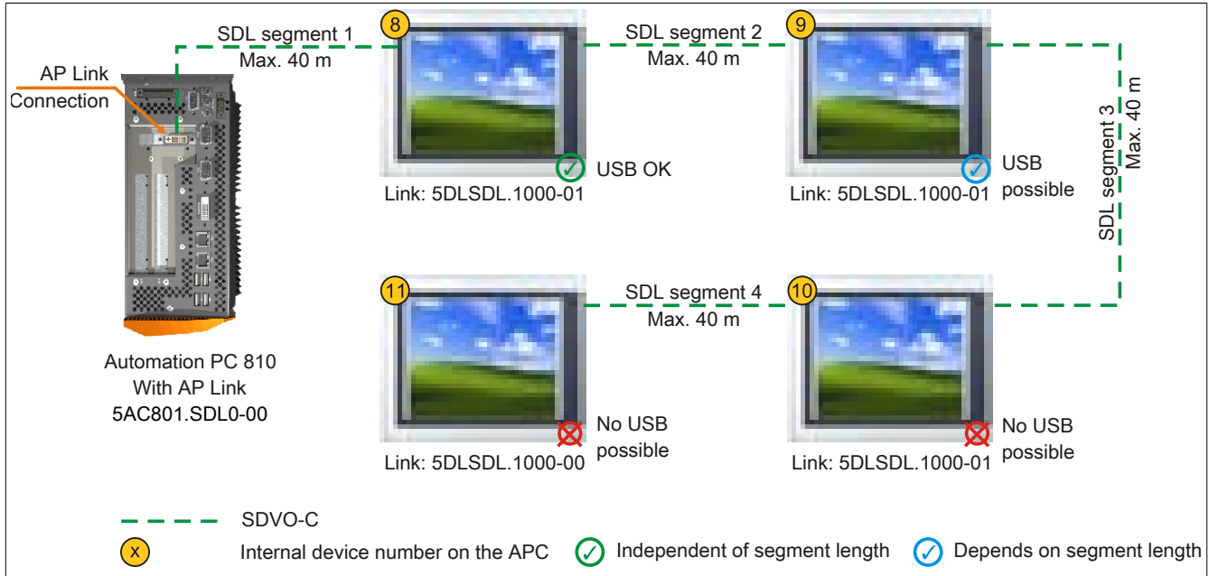
Figure 102: Four Automation Panel 900 systems via SDL AP Link
