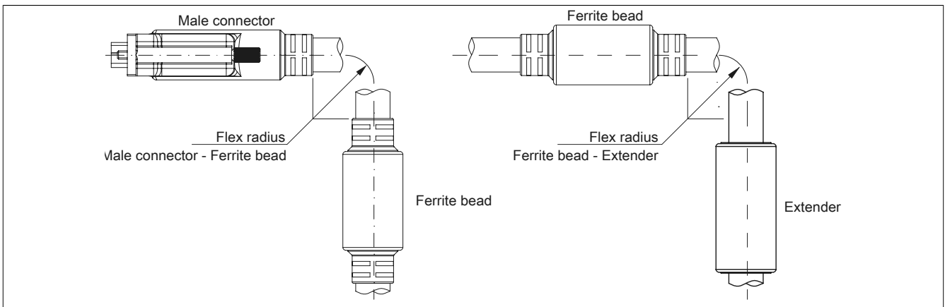
Figure 222: Flex radius specification with extender
