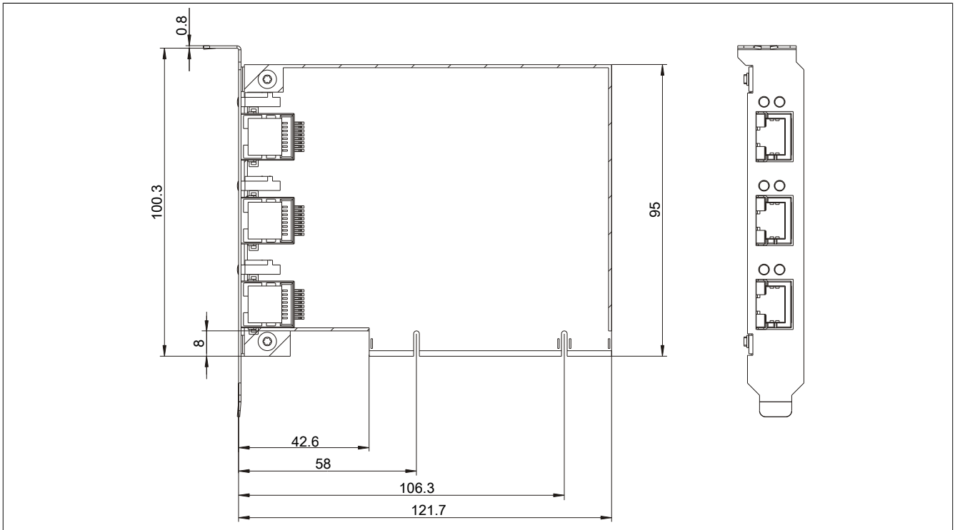
Figure 209: 5ACPCI.ETH3-01 - Dimensions
