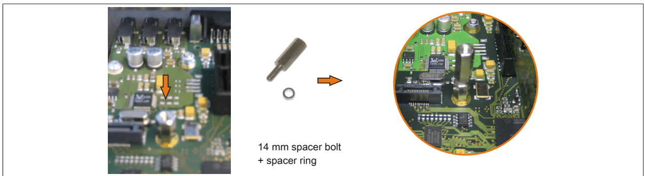
Figure 246: Screwing in the spacer bolt and spacer ring
