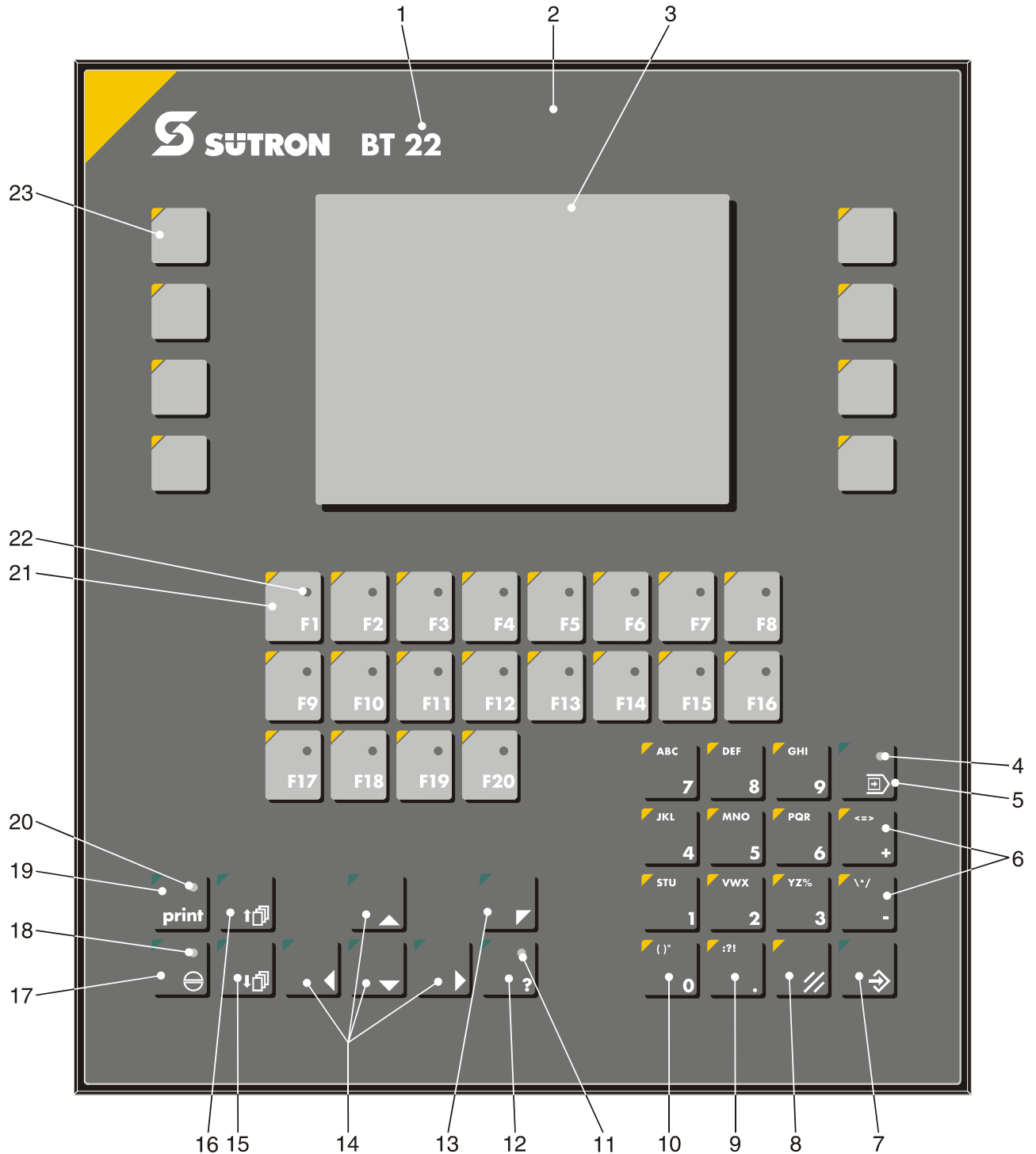
Figure 3-1 Front view
