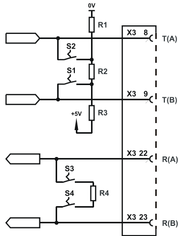
Figure 4-4 Block diagram termination RS485
