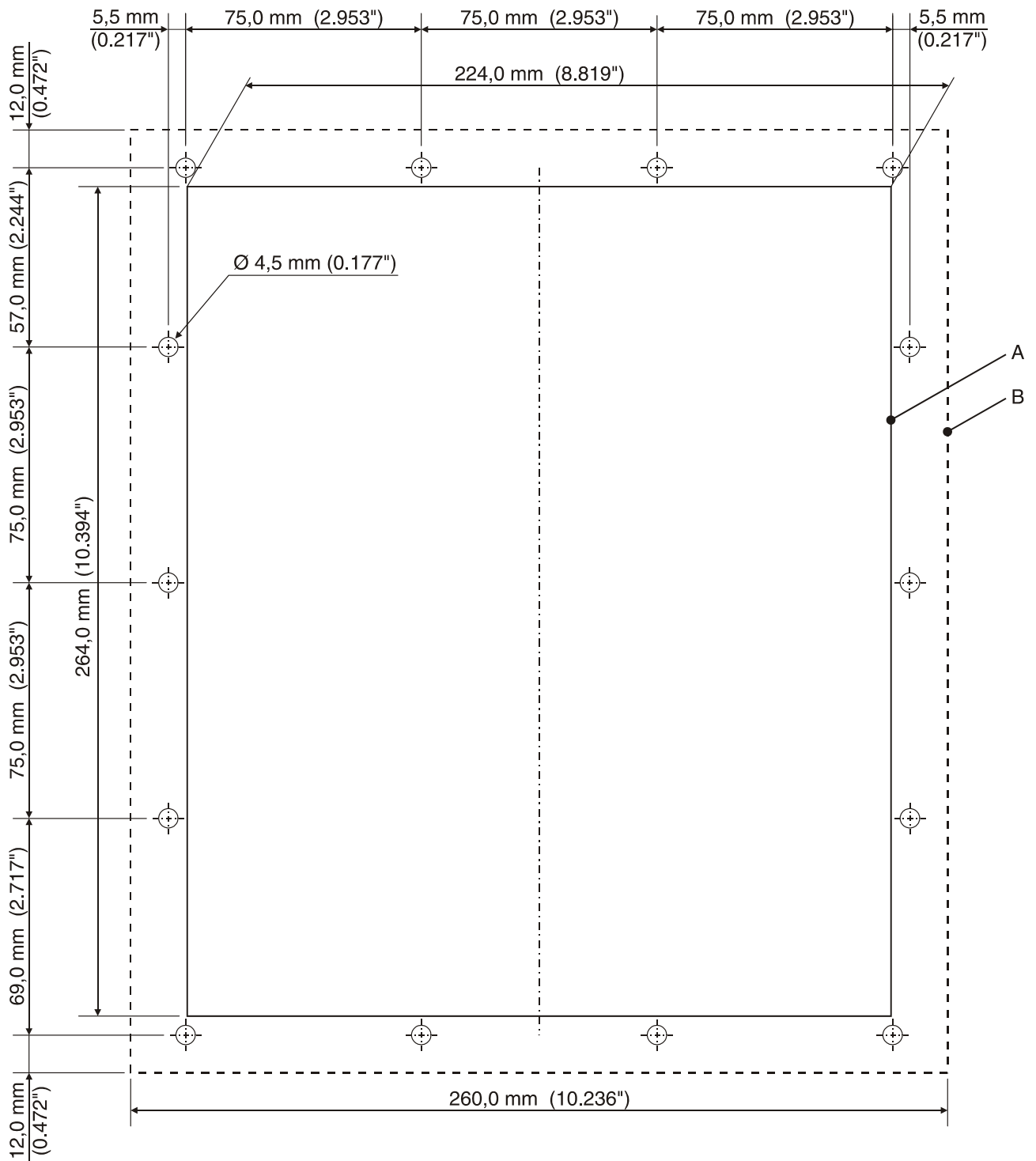
Figure 2-2 Mounting cutout
