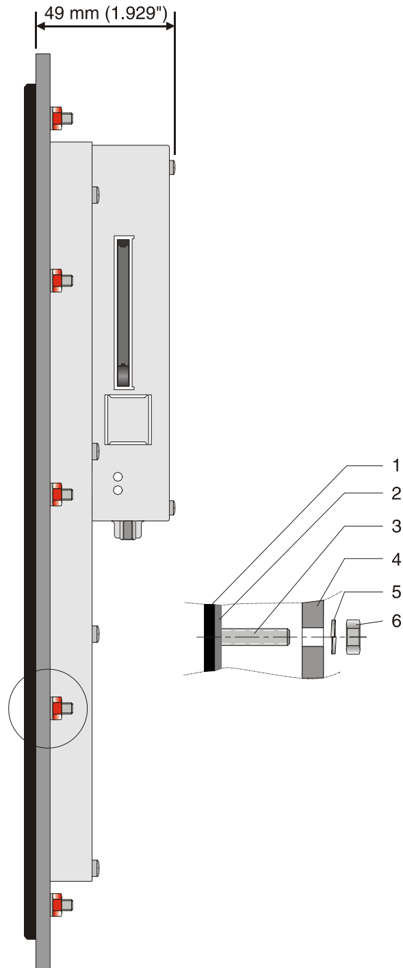
Figure 2-3 Side view and mounting depth for the standard device
