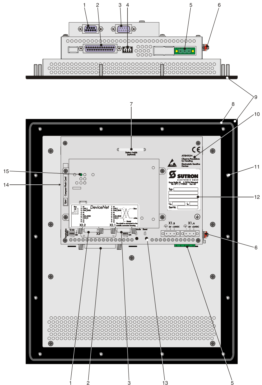
Figure 4-10 Rear view DeviceNet
