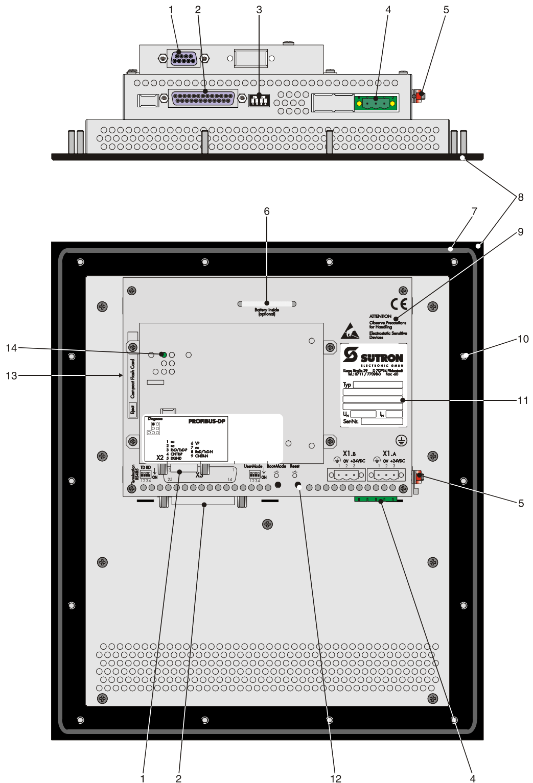
Figure 4-21 Rear view PROFIBUS-DP
