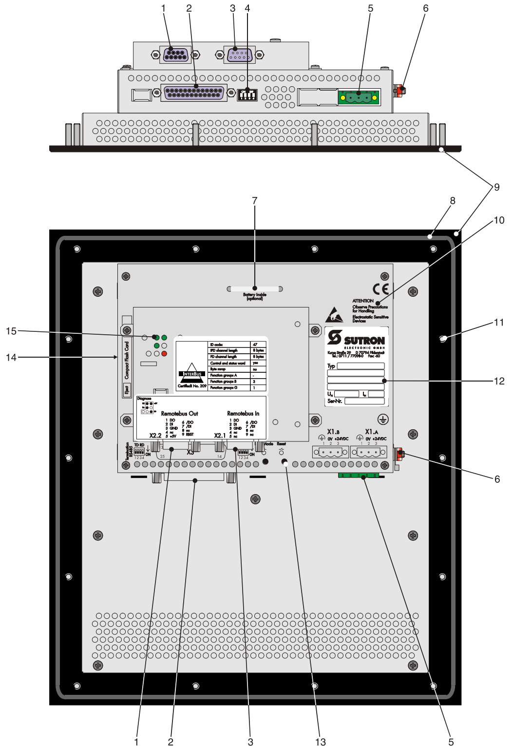
Figure 4-13 Rear view INTERBUS
