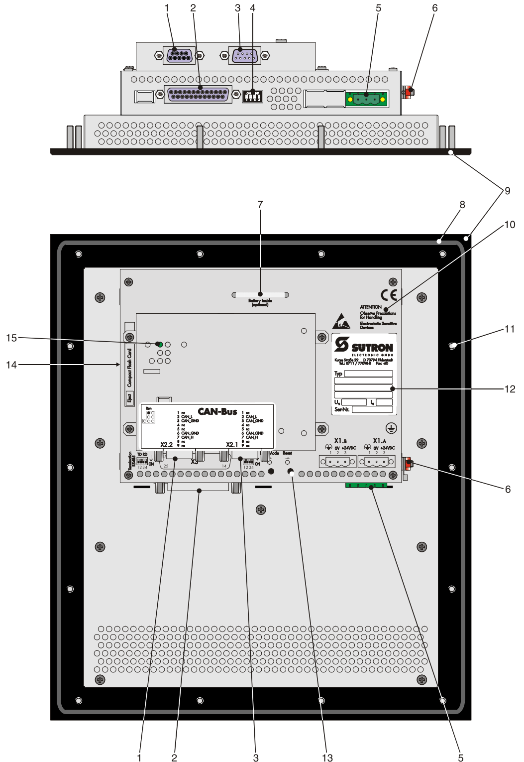
Figure 4-7 Rear view CAN
