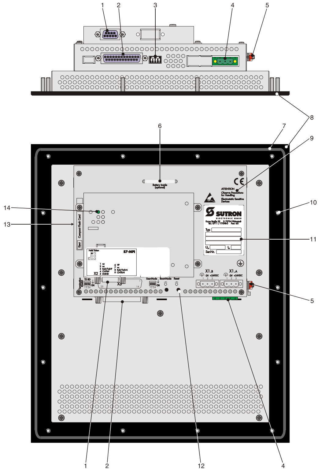
Figure 4-18 Rear View MPI
