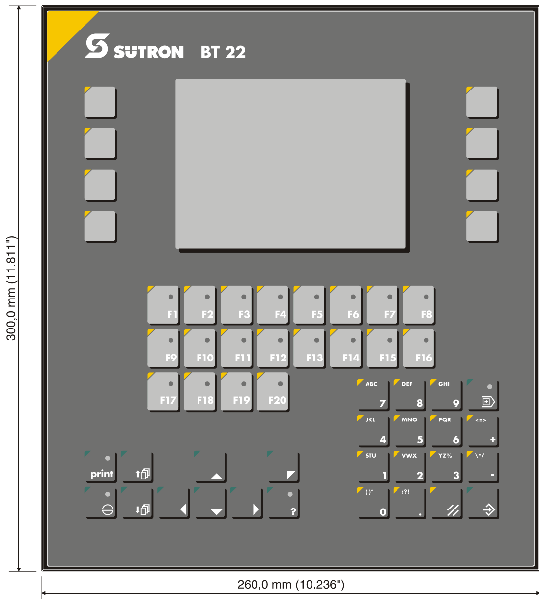
Figure 2-1 Front panel dimensions
