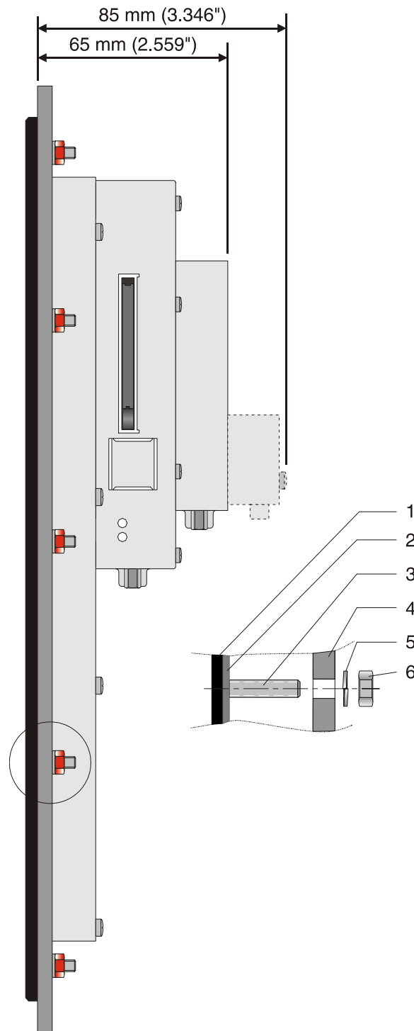
Figure 2-4 Side view and mounting depth for the field bus device
