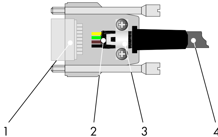
Figure 4-27 Shielding D-SUB connectors
