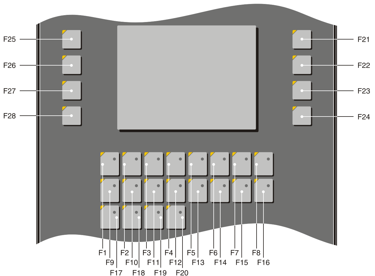
Figure 3-2 Arrangement of the function keys
