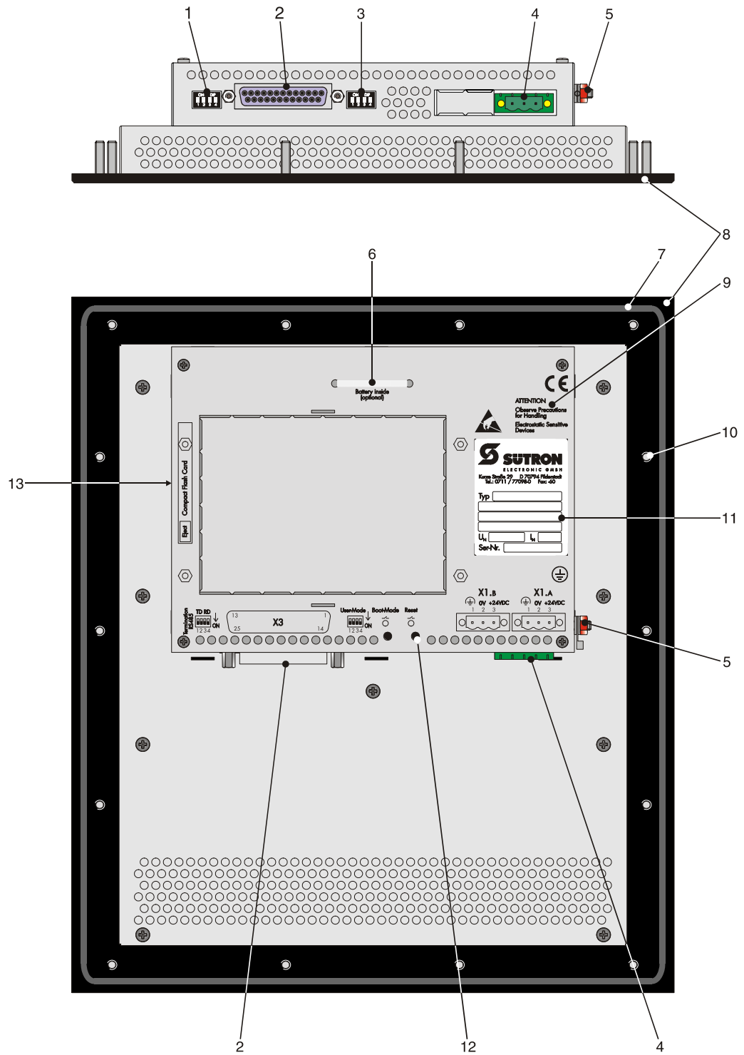
Figure 4-1 Rear view TTY / RS485 / RS232c
