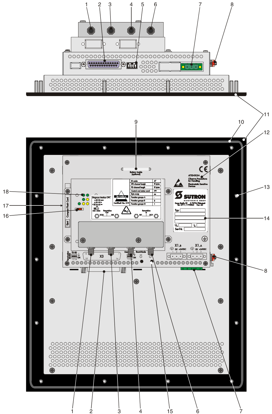
Figure 4-16 Rear view INTERBUS OPC LWL
