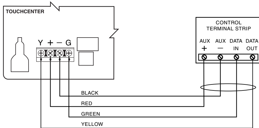
POWERING THE TOUCHCENTER KEYPAD FROM THE CONTROL
